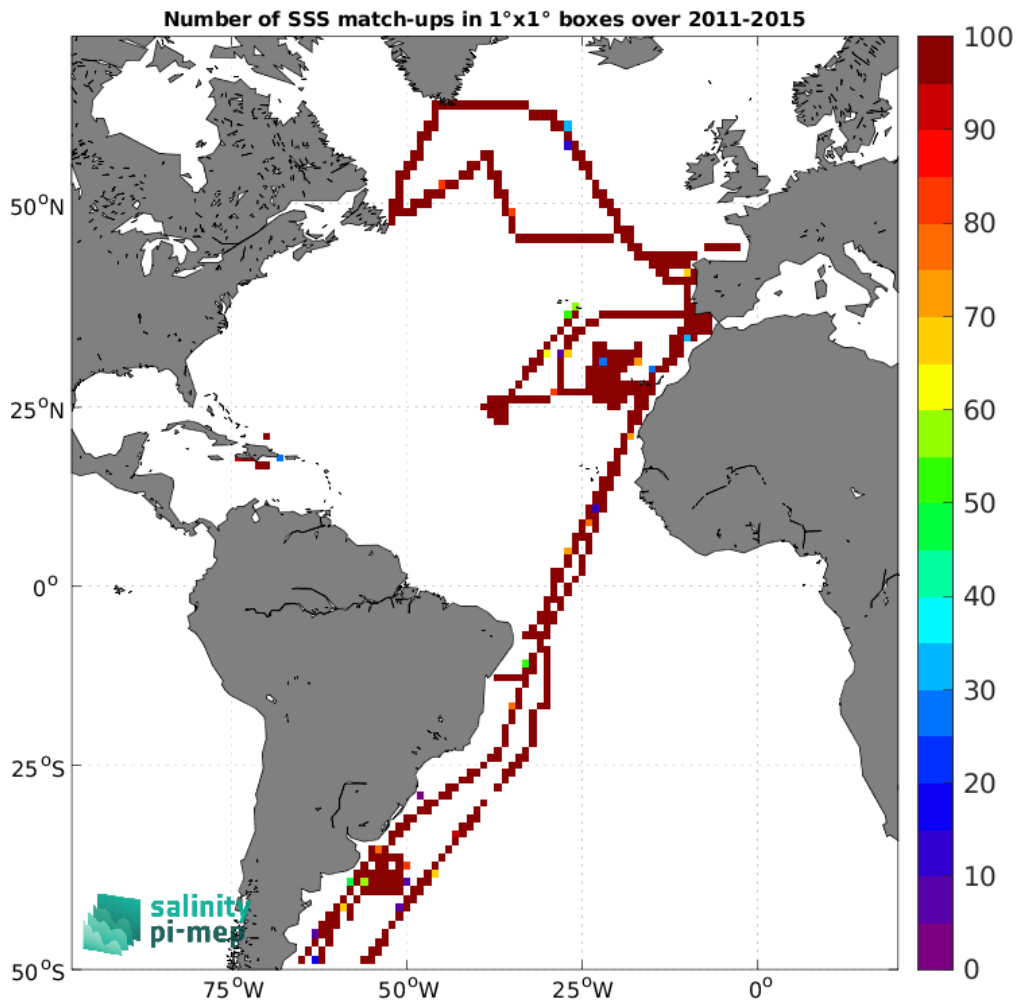
Figure 4: Number of SSS match-ups between TSG (CSIC-UTM) SSS and the Aquarius SSS L3 CAP v5 - Monthly (JPL) SSS product for the Atlantic Ocean Pi-MEP region over 1^{\circ} \times 1^{\circ} boxes and for the full satellite product period.
