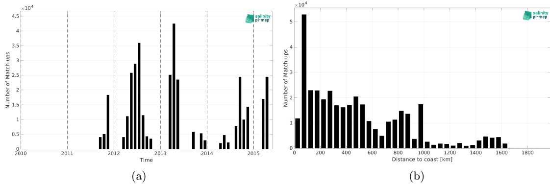
Figure 1: Number of match-ups between TSG (CSIC-UTM) and Aquarius SSS L3 CAP v5 - Monthly (JPL) SSS as a function of time (a) and as function of the distance to coast (b) over the Atlantic Ocean Pi-MEP region and for the full satellite product period.
