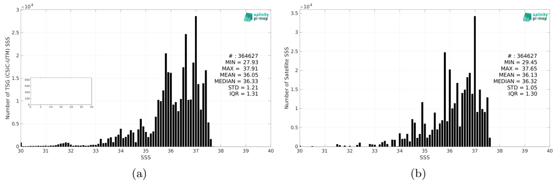
Figure 2: Histograms of SSS from TSG (CSIC-UTM) (a) and Aquarius SSS L3 CAP v5 - Monthly (JPL) (b) considering all match-up pairs per bins of 0.1 over the Atlantic Ocean Pi-MEP region and for the full satellite product period.
