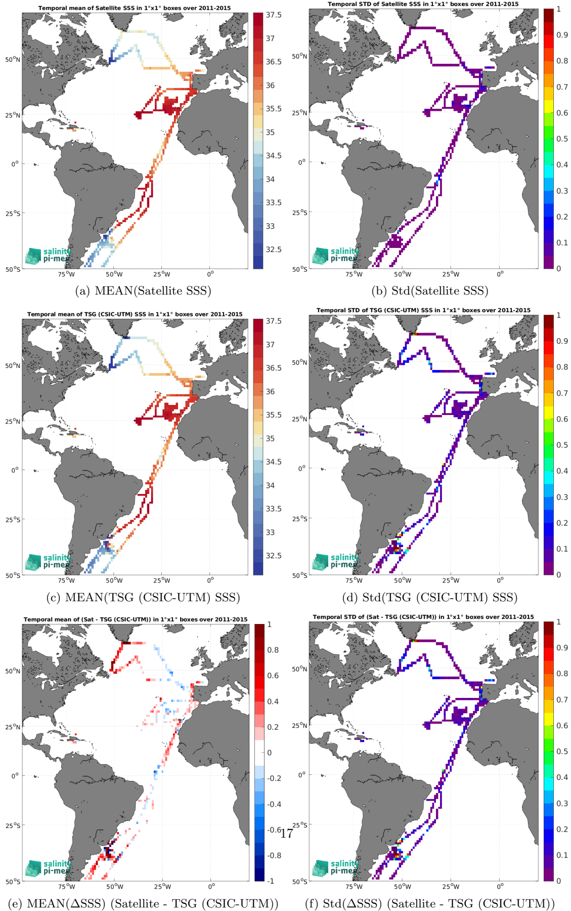
Figure 6: Temporal mean (left) and Std (right) of SSS from Aquarius SSS L3 CAP v5 - Monthly (JPL) (top), TSG (CSIC-UTM) (middle), and of \Delta SSS (Satellite - TSG (CSIC-UTM)). Only match-up pairs are used to generate these maps.
