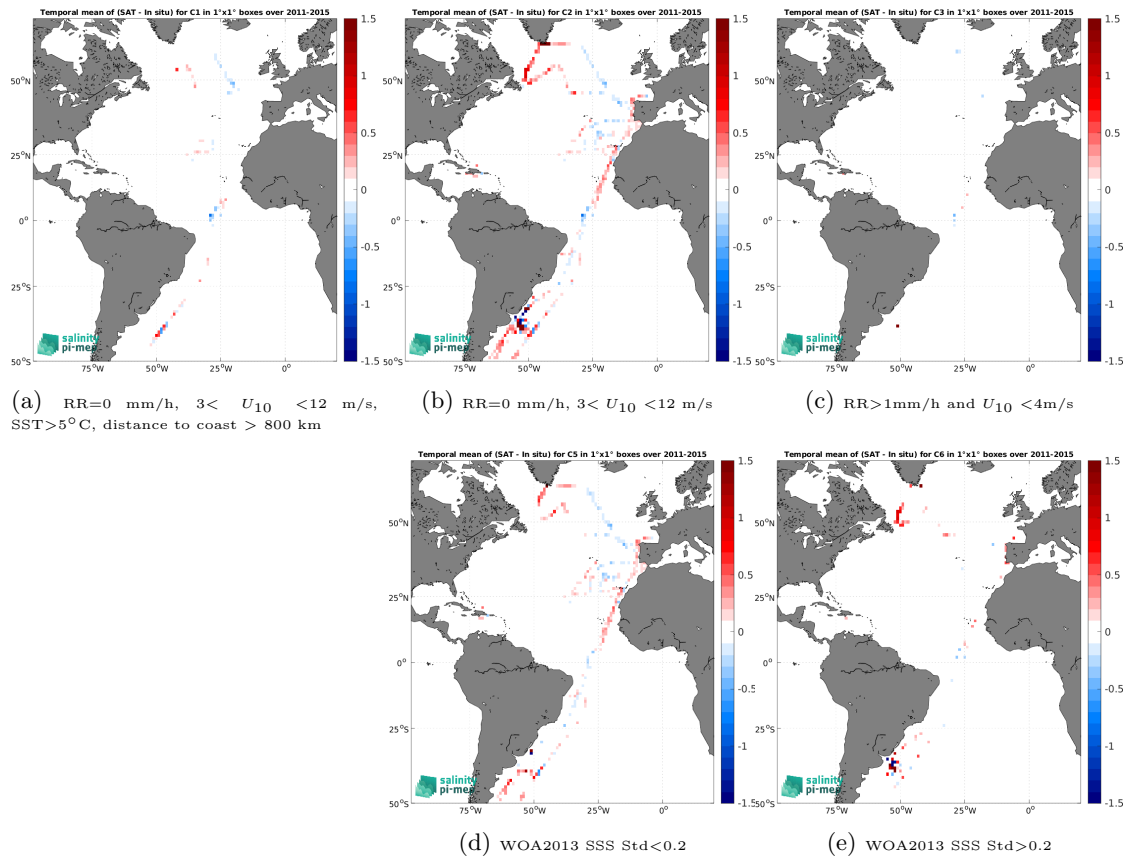
Figure 12: Temporal mean gridded over spatial boxes of size 1^\circ \times 1^\circ of \Delta\text{SSS} (Aquarius SSS L3 CAP v5 - Monthly (JPL) - TSG (CSIC-UTM)) for 5 different subdatasets corresponding to:RR=0 mm/h, 3 < U_{10} < 12 m/s, SST >5^\circ\text{C} , distance to coast > 800 km (a), RR=0 mm/h, 3 < U_{10} < 12 m/s (b), RR >1 mm/h and U_{10} < 4 m/s (c), WOA2013 SSS Std <0.2 (d), WOA2013 SSS Std >0.2 (e).
