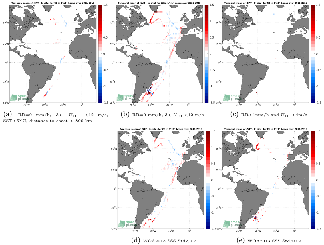
Figure 12: Temporal mean gridded over spatial boxes of size 1^\circ \times 1^\circ of \Delta SSS (Aquarius SSS L3 CAP v5 - Monthly (JPL) - TSG (CSIC-UTM)) for 5 different subdatasets corresponding to:RR=0 mm/h, 3 < U_{10} < 12 m/s, SST >5^\circ\text{C} , distance to coast > 800 km (a), RR=0 mm/h, 3 < U_{10} < 12 m/s (b), RR >1 mm/h and U_{10} < 4 m/s (c), WOA2013 SSS Std <0.2 (d), WOA2013 SSS Std >0.2 (e).
