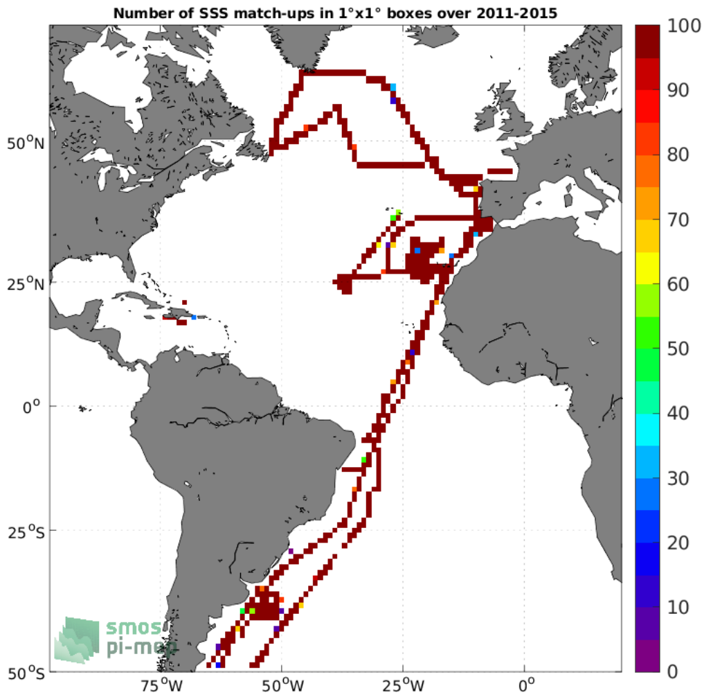
Figure 4: Number of SSS match-ups between TSG (CSIC-UTM) SSS and the Aquarius SSS L3 CAP v5 - Monthly (JPL) SSS product for the Atlantic Ocean Pi-MEP region over 1°x1° boxes and for the full satellite product period.
