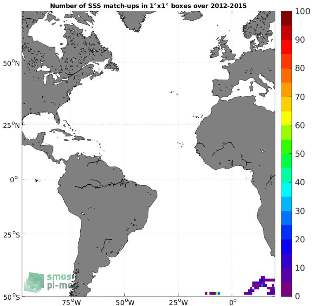
Figure 4: Number of SSS match-ups between Marine mammals SSS and the Aquarius SSS L3 CAP v5 - Monthly (JPL) SSS product for the Atlantic Ocean Pi-MEP region over 1°×1° boxes and for the full satellite product period.
