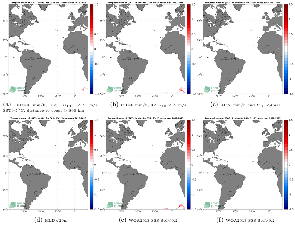
Figure 12: Temporal mean gridded over spatial boxes of size 1^\circ \times 1^\circ of \Delta SSS (Aquarius SSS L3 CAP v5 - Monthly (JPL) - Marine mammals) for 6 different subdatasets corresponding to:RR=0 mm/h, 3 < U_{10} < 12 m/s, SST>5°C, distance to coast > 800 km (a), RR=0 mm/h, 3 < U_{10} < 12 m/s (b), RR>1mm/h and U_{10} < 4 m/s (c),MLD<20m (d),WOA2013 SSS Std<0.2 (e),WOA2013 SSS Std>0.2 (f).
