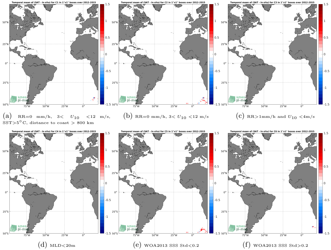
Figure 12: Temporal mean gridded over spatial boxes of size 1°x1° of \Delta SSS (Aquarius SSS L3 CAP v5 - Monthly (JPL) - Sea mammals) for 6 different subdatasets corresponding to:RR=0 mm/h, 3 < U_{10} < 12 m/s, SST > 5°C, distance to coast > 800 km (a), RR=0 mm/h, 3 < U_{10} < 12 m/s (b), RR > 1mm/h and U_{10} < 4 m/s (c),MLD < 20m (d),WOA2013 SSS Std < 0.2 (e),WOA2013 SSS Std > 0.2 (f).
