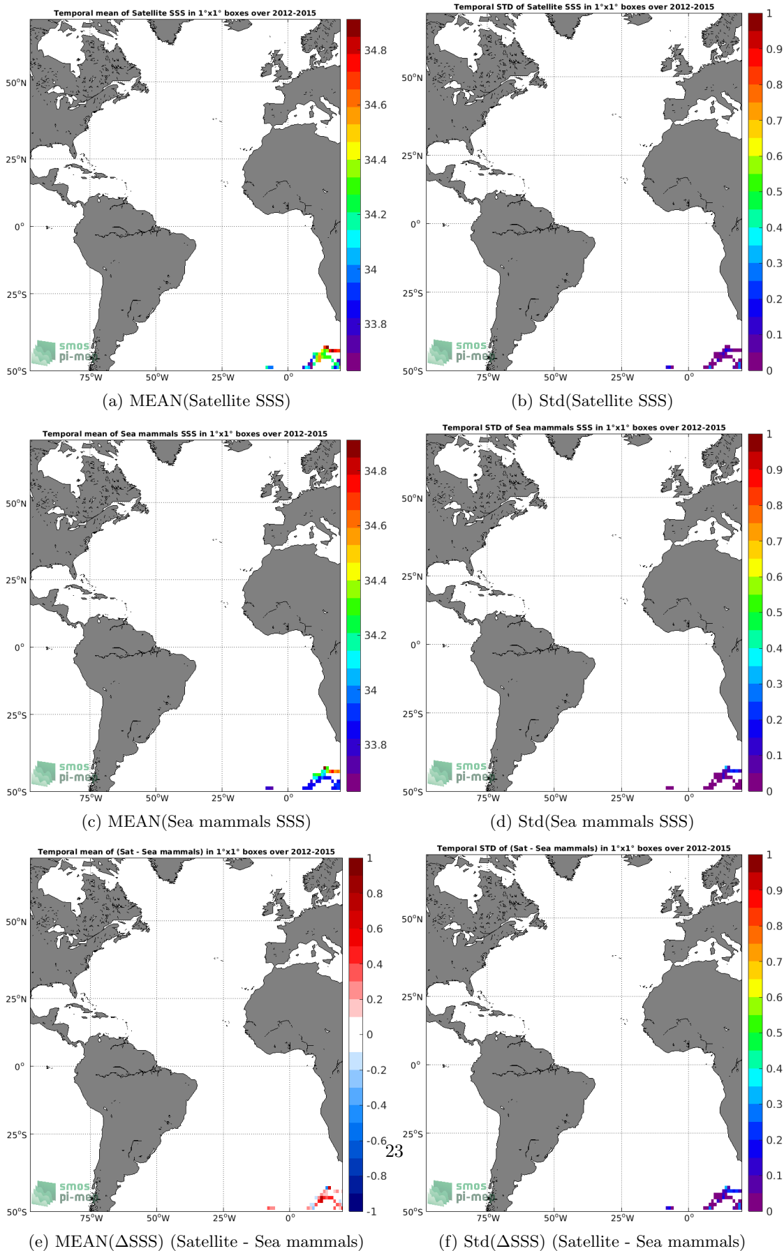
Figure 6: Temporal mean (left) and Std (right) of SSS from Aquarius SSS L3 CAP v5 - Monthly (JPL) (top), Sea mammals (middle), and of \Delta SSS (Satellite - Sea mammals). Only match-up pairs are used to generate these maps.
