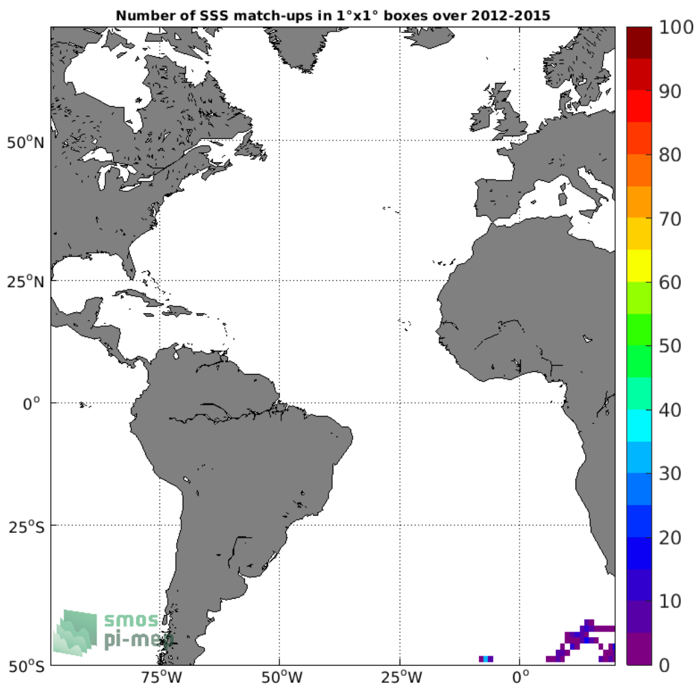
Figure 4: Number of SSS match-ups between Sea mammals SSS and the Aquarius SSS L3 CAP v5 - Monthly (JPL) SSS product for the Atlantic Ocean Pi-MEP region over 1°x1° boxes and for the full satellite product period.
