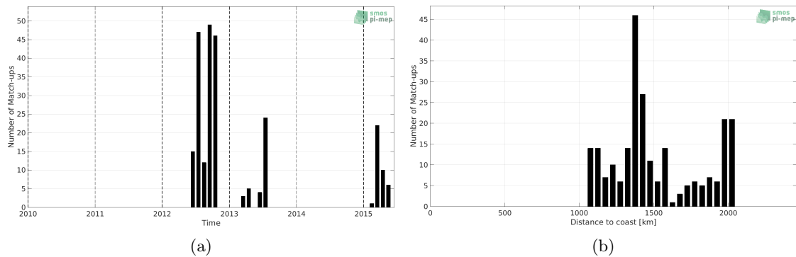
Figure 1: Number of match-ups between Sea mammals and Aquarius SSS L3 CAP v5 - Monthly (JPL) SSS as a function of time (a) and as function of the distance to coast (b) over the Atlantic Ocean Pi-MEP region and for the full satellite product period.
