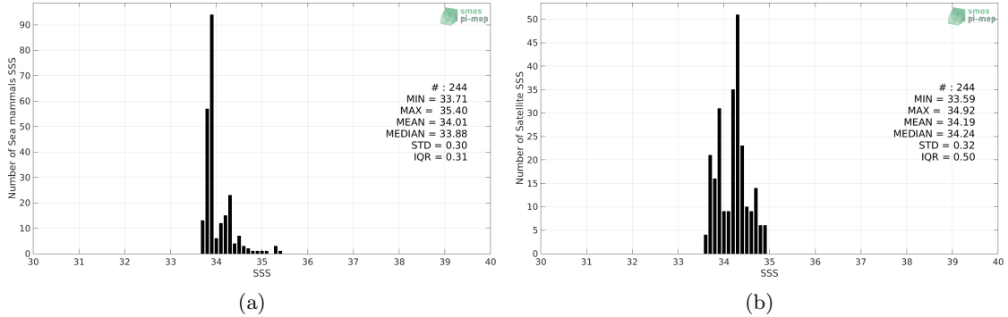
Figure 2: Histograms of SSS from Sea mammals (a) and Aquarius SSS L3 CAP v5 - Monthly (JPL) (b) considering all match-up pairs per bins of 0.1 over the Atlantic Ocean Pi-MEP region and for the full satellite product period.
