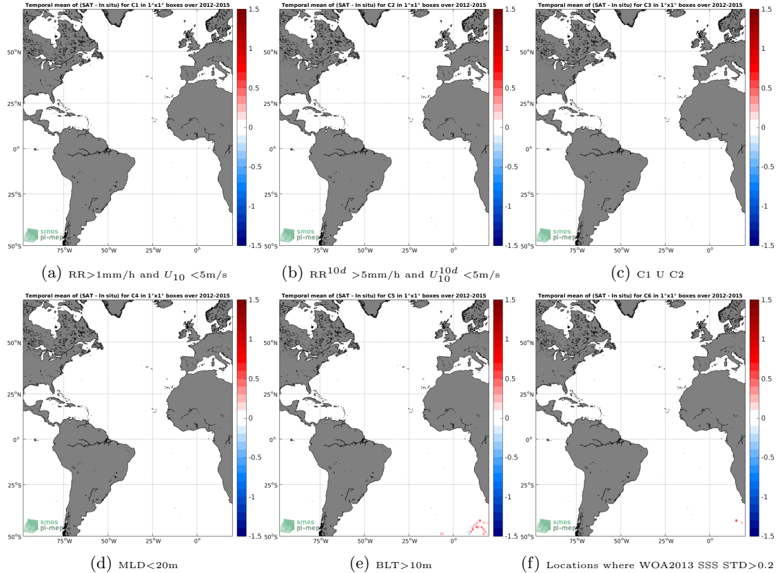
Figure 12: Temporal mean gridded over spatial boxes of size 1^\circ \times 1^\circ of \Delta\text{SSS} (Aquarius-L3-JPL-V5-MONTHLY - Sea mammals) for 6 different subdatasets corresponding to: \text{RR} > 1\text{mm/h} and U_{10} < 5\text{m/s} (a), \text{RR}^{10d} > 5\text{mm/h} and U_{10}^{10d} < 5\text{m/s} (b), C1 U C2 (c), \text{MLD} < 20\text{m} (d), \text{BLT} > 10\text{m} (e), Locations where WOA2013 SSS STD > 0.2 (f).
