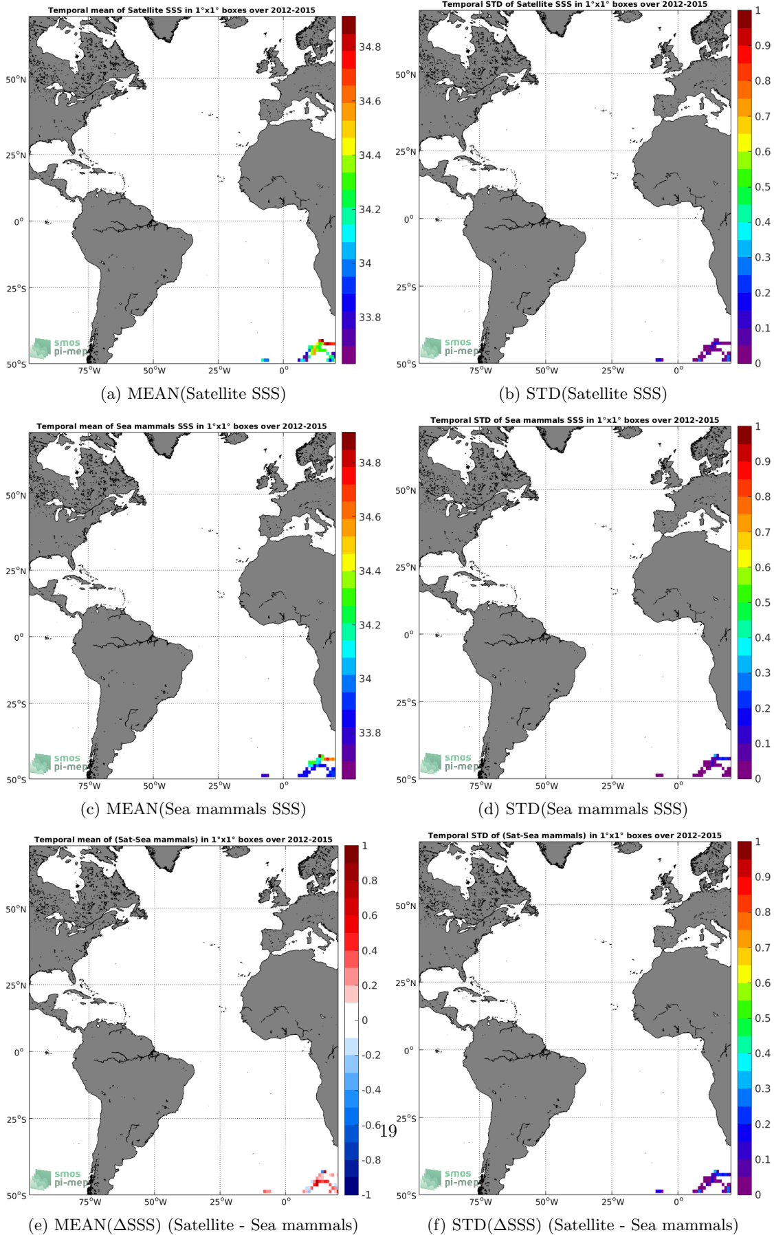
Figure 6: Temporal mean (left) and STD (right) of SSS from Aquarius-L3-JPL-V5-MONTHLY (top), Sea mammals (middle), and of \Delta SSS (Satellite - Sea mammals). Only match-up pairs are used to generate these maps.
