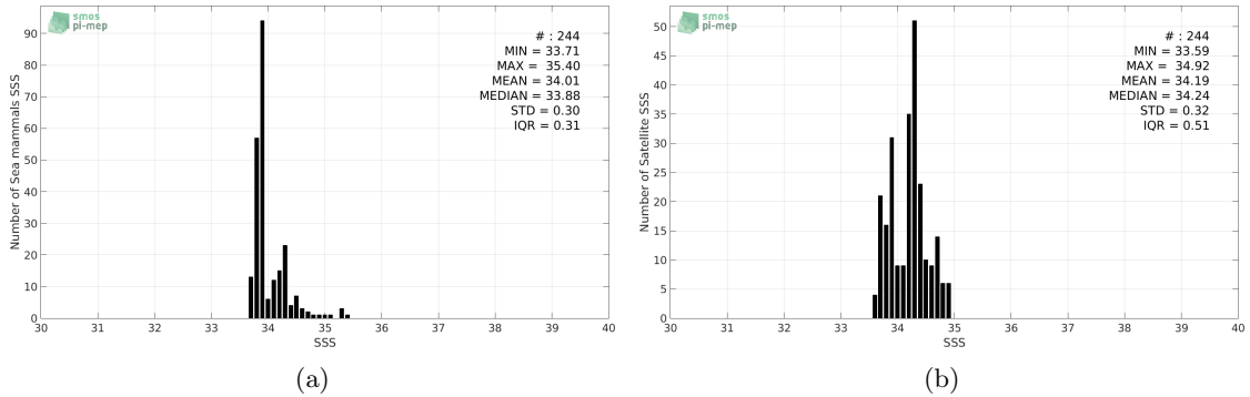
Figure 2: Histograms of SSS from Sea mammals (a) and Aquarius-L3-JPL-V5-MONTHLY (b) considering all match-up pairs per bins of 0.1 over the Atlantic Ocean Pi-MEP region and for the full satellite product period.
