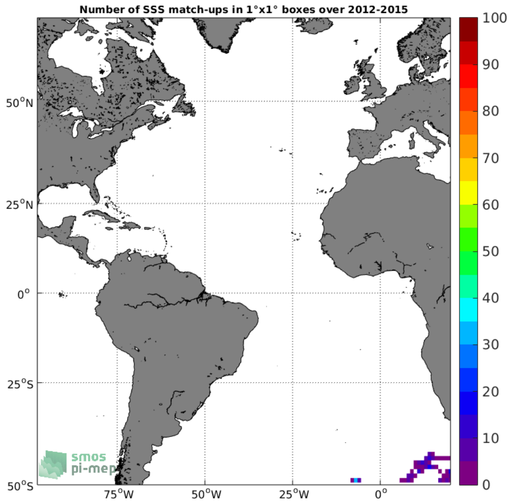
Figure 4: Number of SSS match-ups between Sea mammals SSS and the Aquarius-L3-JPL-V5-MONTHLY SSS product for the Atlantic Ocean Pi-MEP region over 1°x1° boxes and for the full satellite product period.
