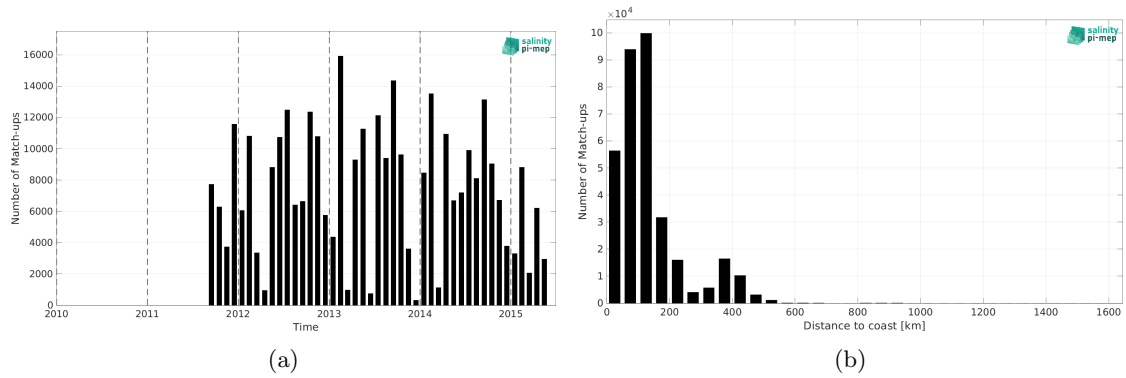
Figure 2: Number of match-ups between ICES and Aquarius SSS L3 CAP v5 - Monthly (JPL) SSS as a function of time (a) and as function of the distance to coast (b) over the Atlantic Ocean Pi-MEP region and for the full satellite product period.
