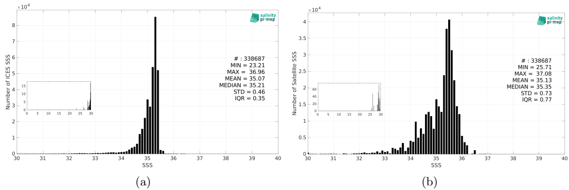
Figure 3: Histograms of SSS from ICES (a) and Aquarius SSS L3 CAP v5 - Monthly (JPL) (b) considering all match-up pairs per bins of 0.1 over the Atlantic Ocean Pi-MEP region and for the full satellite product period.
