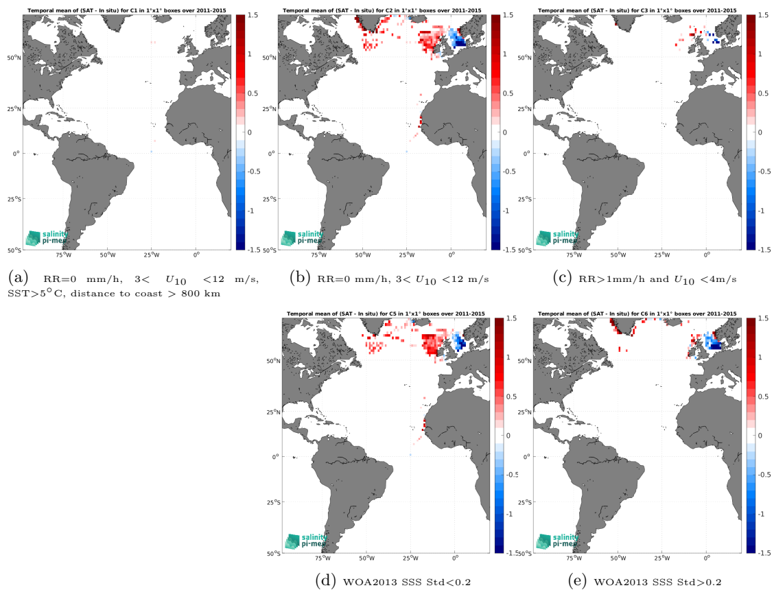
Figure 14: Temporal mean gridded over spatial boxes of size 1^\circ \times 1^\circ of \Delta SSS (Aquarius SSS L3 CAP v5 - Monthly (JPL) - ICES) for 5 different subdatasets corresponding to:RR=0 mm/h, 3 < U_{10} < 12 m/s, SST >5^\circ\text{C} , distance to coast > 800 km (a), RR=0 mm/h, 3 < U_{10} < 12 m/s (b), RR >1 mm/h and U_{10} < 4 m/s (c), WOA2013 SSS Std <0.2 (d), WOA2013 SSS Std >0.2 (e).
