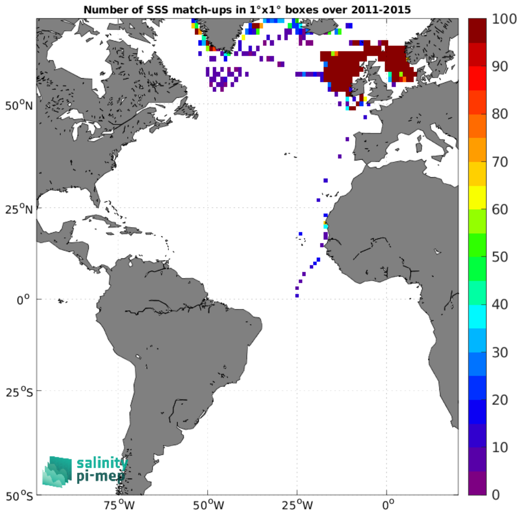
Figure 5: Number of SSS match-ups between ICES SSS and the Aquarius SSS L3 CAP v5 - Monthly (JPL) SSS product for the Atlantic Ocean Pi-MEP region over 1^\circ \times 1^\circ boxes and for the full satellite product period.
