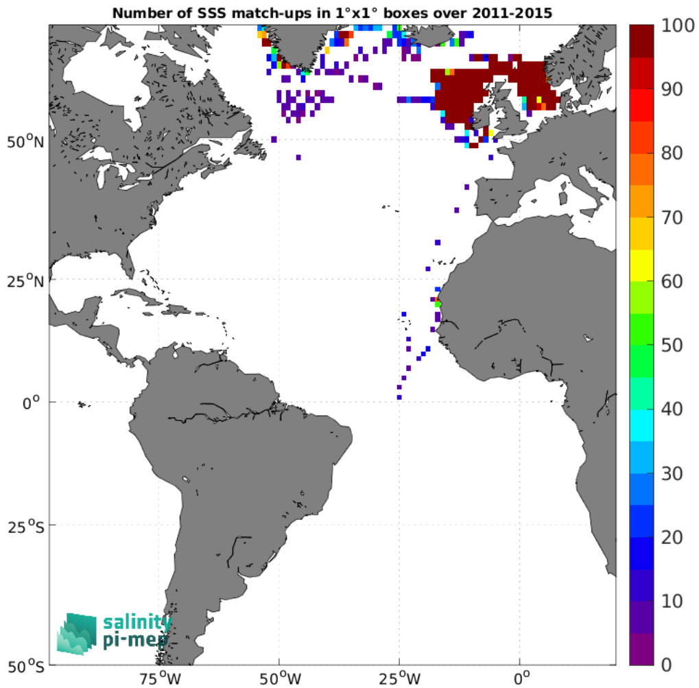
Figure 4: Number of SSS match-ups between ICES SSS and the Aquarius SSS L3 CAP v5 - Monthly (JPL) SSS product for the Atlantic Ocean Pi-MEP region over 1^{\circ} \times 1^{\circ} boxes and for the full satellite product period.
