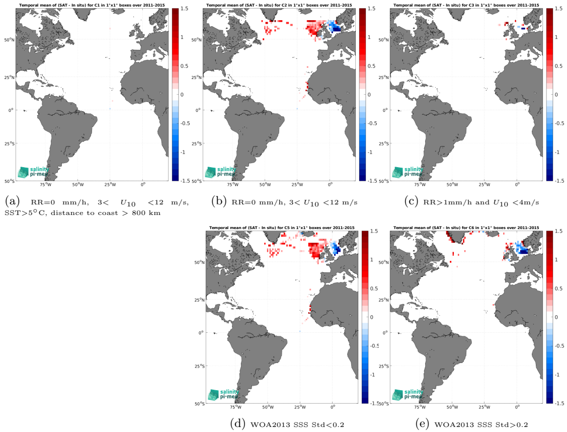
Figure 12: Temporal mean gridded over spatial boxes of size 1^\circ \times 1^\circ of \Delta SSS (Aquarius SSS L3 CAP v5 - Monthly (JPL) - ICES) for 5 different subdatasets corresponding to:RR=0 mm/h, 3 < U_{10} < 12 m/s, SST >5^\circ\text{C} , distance to coast > 800 km (a), RR=0 mm/h, 3 < U_{10} < 12 m/s (b), RR >1 mm/h and U_{10} < 4 m/s (c), WOA2013 SSS Std <0.2 (d), WOA2013 SSS Std >0.2 (e).
