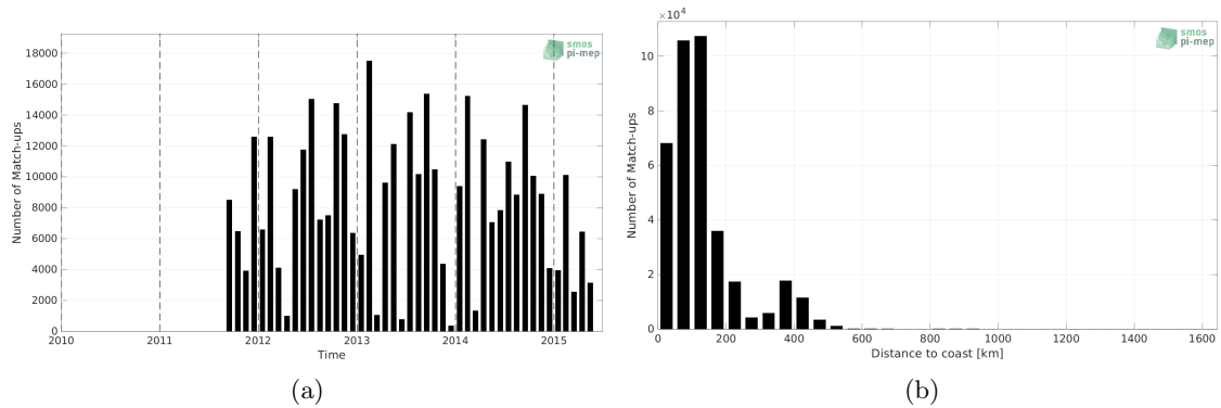
Figure 1: Number of match-ups between ICES and Aquarius SSS L3 CAP v5 - Monthly (JPL) SSS as a function of time (a) and as function of the distance to coast (b) over the Atlantic Ocean Pi-MEP region and for the full satellite product period.
