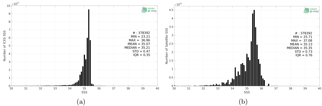
Figure 2: Histograms of SSS from ICES (a) and Aquarius SSS L3 CAP v5 - Monthly (JPL) (b) considering all match-up pairs per bins of 0.1 over the Atlantic Ocean Pi-MEP region and for the full satellite product period.
