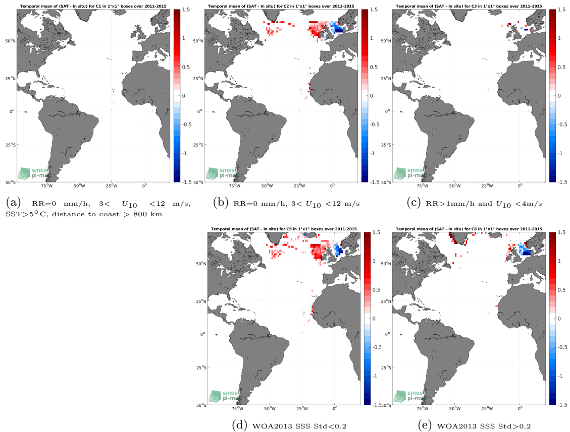
Figure 12: Temporal mean gridded over spatial boxes of size 1^\circ \times 1^\circ of \Delta SSS (Aquarius SSS L3 CAP v5 - Monthly (JPL) - ICES) for 5 different subdatasets corresponding to:RR=0 mm/h, 3 < U_{10} < 12 m/s, SST >5^\circ\text{C} , distance to coast > 800 km (a), RR=0 mm/h, 3 < U_{10} < 12 m/s (b), RR >1 mm/h and U_{10} < 4 m/s (c), WOA2013 SSS Std <0.2 (d), WOA2013 SSS Std >0.2 (e).
