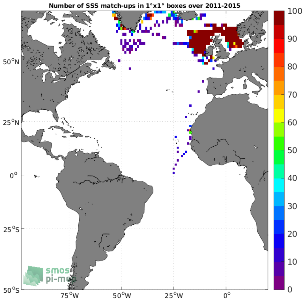
Figure 4: Number of SSS match-ups between ICES SSS and the Aquarius SSS L3 CAP v5 - Monthly (JPL) SSS product for the Atlantic Ocean Pi-MEP region over 1°x1° boxes and for the full satellite product period.
