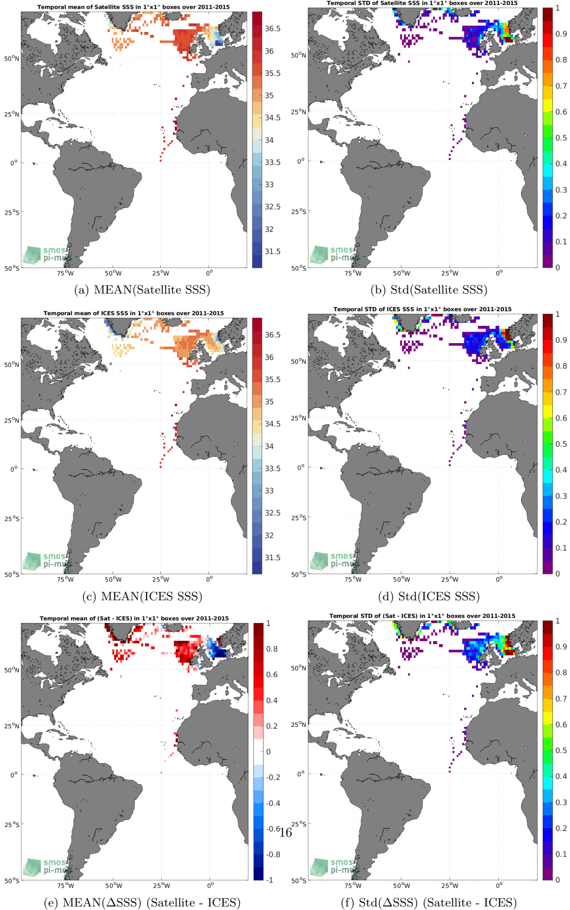
Figure 6: Temporal mean (left) and Std (right) of SSS from Aquarius SSS L3 CAP v5 - Monthly (JPL) (top), ICES (middle), and of \Delta SSS (Satellite - ICES). Only match-up pairs are used to generate these maps.
