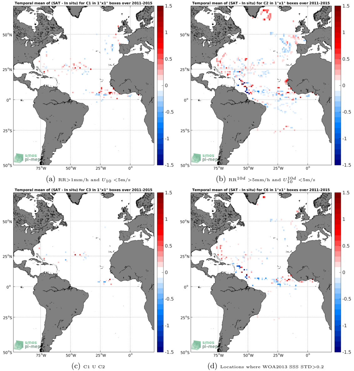
Figure 11: Temporal mean gridded over spatial boxes of size 1^\circ \times 1^\circ of \Delta SSS (Aquarius-L3-JPL-V5-MONTHLY - Surface drifters) for 4 different subdatasets corresponding to:RR >1 mm/h and U_{10} < 5 m/s (a), RR 10d > 5 mm/h and U_{10}^{10d} < 5 m/s (b), C1 U C2 (c),Locations where WOA2013 SSS STD > 0.2 (d).
