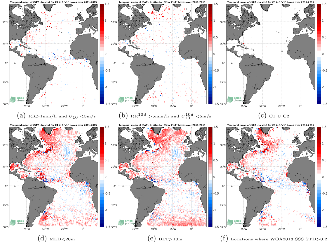
Figure 12: Temporal mean gridded over spatial boxes of size 1^\circ \times 1^\circ of \Delta\text{SSS} (Aquarius-L3-JPL-V5-MONTHLY - Argo) for 6 different subdatasets corresponding to: \text{RR} > 1\text{mm/h} and U_{10} < 5\text{m/s} (a), \text{RR}^{10d} > 5\text{mm/h} and U_{10}^{10d} < 5\text{m/s} (b), C1 U C2 (c), \text{MLD} < 20\text{m} (d), \text{BLT} > 10\text{m} (e), Locations where WOA2013 SSS STD > 0.2 (f).
