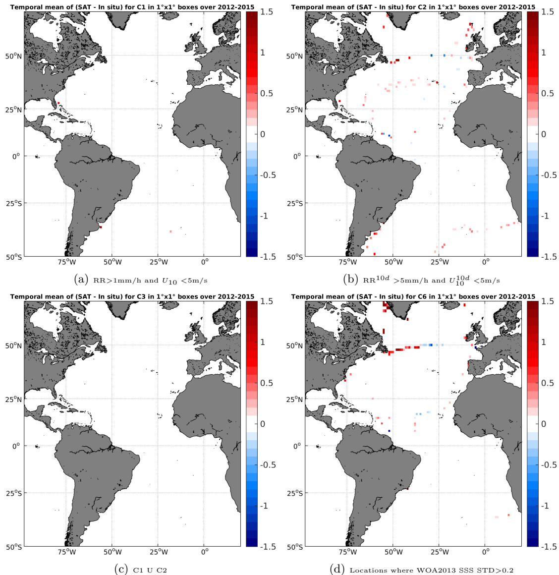
Figure 12: Temporal mean gridded over spatial boxes of size 1^\circ \times 1^\circ of \Delta SSS (Aquarius-L3-JPL-V4-MONTHLY - TSG-GOSUD-Sailing-ship) for 4 different subdatasets corresponding to: RR > 1 mm/h and U_{10} < 5 m/s (a), RR 10d > 5 mm/h and U_{10}^{10d} < 5 m/s (b), C1 U C2 (c), Locations where WOA2013 SSS STD > 0.2 (d).
