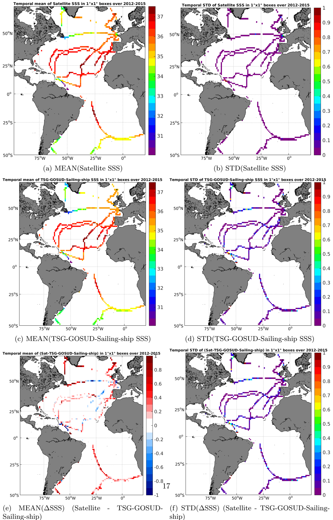
Figure 6: Temporal mean (left) and STD (right) of SSS from Aquarius-L3-JPL-V4-MONTHLY (top), TSG-GOSUD-Sailing-ship (middle), and of \Delta SSS (Satellite - TSG-GOSUD-Sailing-ship). Only match-up pairs are used to generate these maps.
