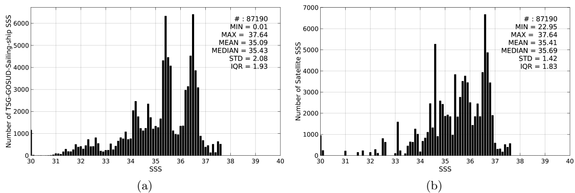
Figure 2: Histograms of SSS from TSG-GOSUD-Sailing-ship (a) and Aquarius-L3-JPL-V4-MONTHLY (b) considering all match-up pairs per bins of 0.1 over the Atlantic Ocean Pi-MEP region and for the full satellite product period.
