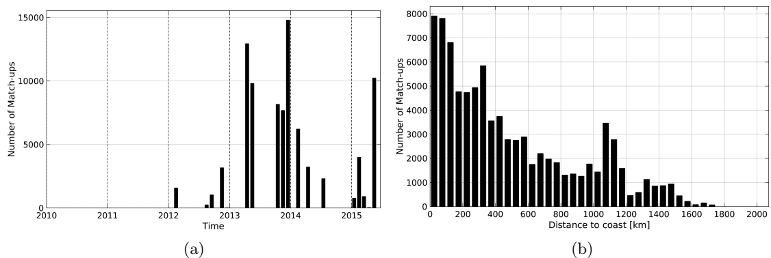
Figure 1: Number of match-ups between TSG-GOSUD-Sailing-ship and Aquarius-L3-JPL-V4-MONTHLY SSS as a function of time (a) and as function of the distance to coast (b) over the Atlantic Ocean Pi-MEP region and for the full satellite product period.
