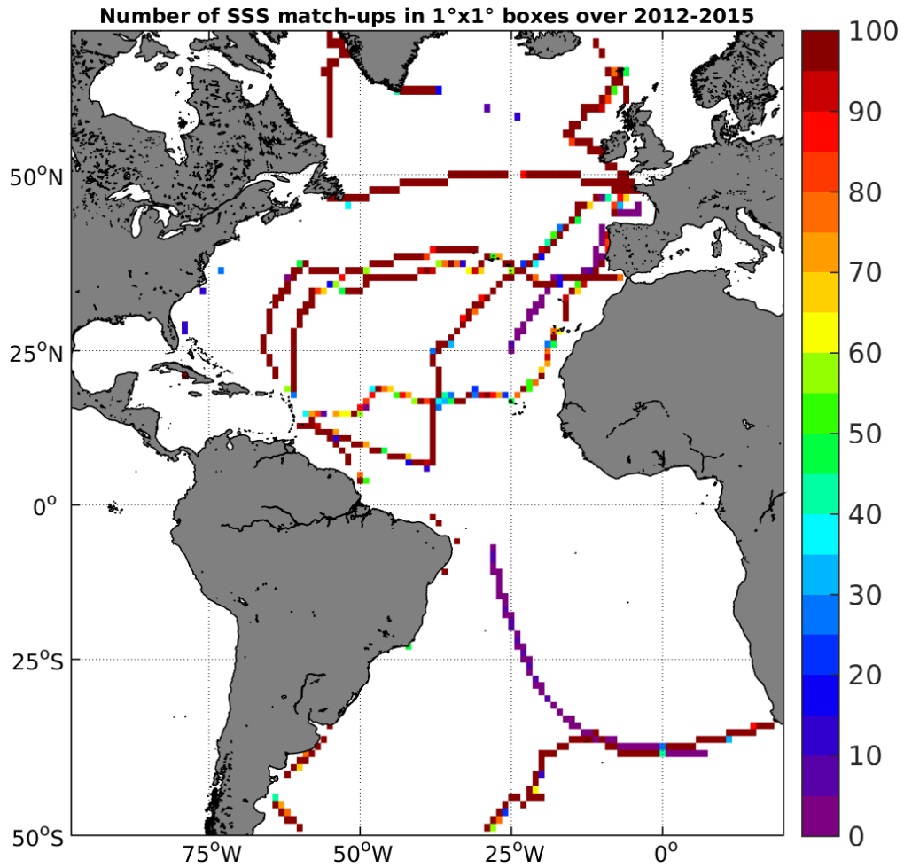
Figure 4: Number of SSS match-ups between TSG-GOSUD-Sailing-ship SSS and the Aquarius-L3-JPL-V4-MONTHLY SSS product for the Atlantic Ocean Pi-MEP region over 1°x1° boxes and for the full satellite product period.
