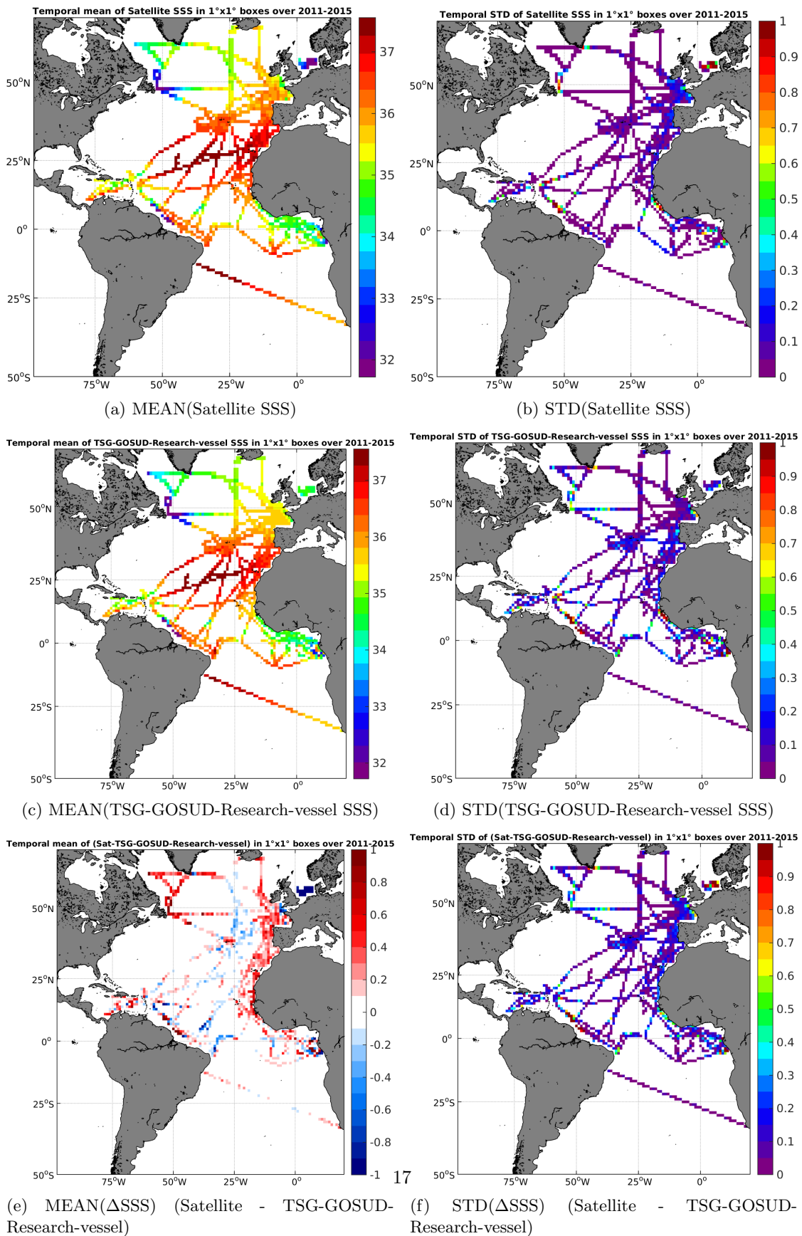
Figure 6: Temporal mean (left) and STD (right) of SSS from Aquarius-L3-JPL-V4-MONTHLY (top), TSG-GOSUD-Research-vessel (middle), and of \Delta SSS (Satellite - TSG-GOSUD-Research-vessel). Only match-up pairs are used to generate these maps.
