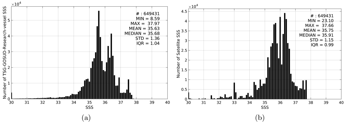
Figure 2: Histograms of SSS from TSG-GOSUD-Research-vessel (a) and Aquarius-L3-JPL-V4-MONTHLY (b) considering all match-up pairs per bins of 0.1 over the Atlantic Ocean Pi-MEP region and for the full satellite product period.
