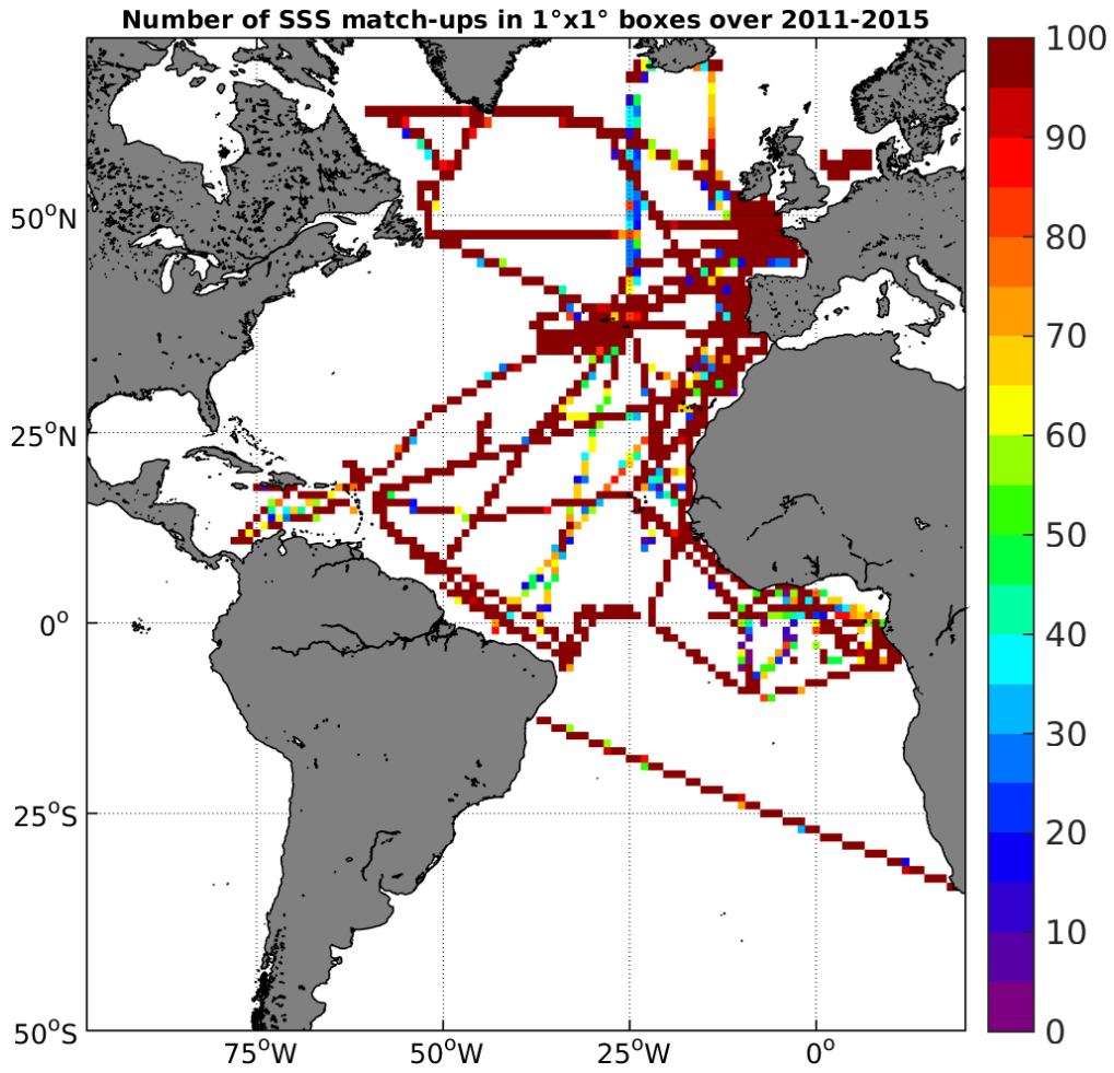
Figure 4: Number of SSS match-ups between TSG-GOSUD-Research-vessel SSS and the Aquarius-L3-JPL-V4-MONTHLY SSS product for the Atlantic Ocean Pi-MEP region over 1°x1° boxes and for the full satellite product period.
