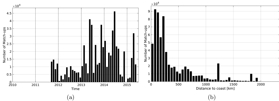
Figure 1: Number of match-ups between TSG-GOSUD-Research-vessel and Aquarius-L3-JPL-V4-MONTHLY SSS as a function of time (a) and as function of the distance to coast (b) over the Atlantic Ocean Pi-MEP region and for the full satellite product period.
