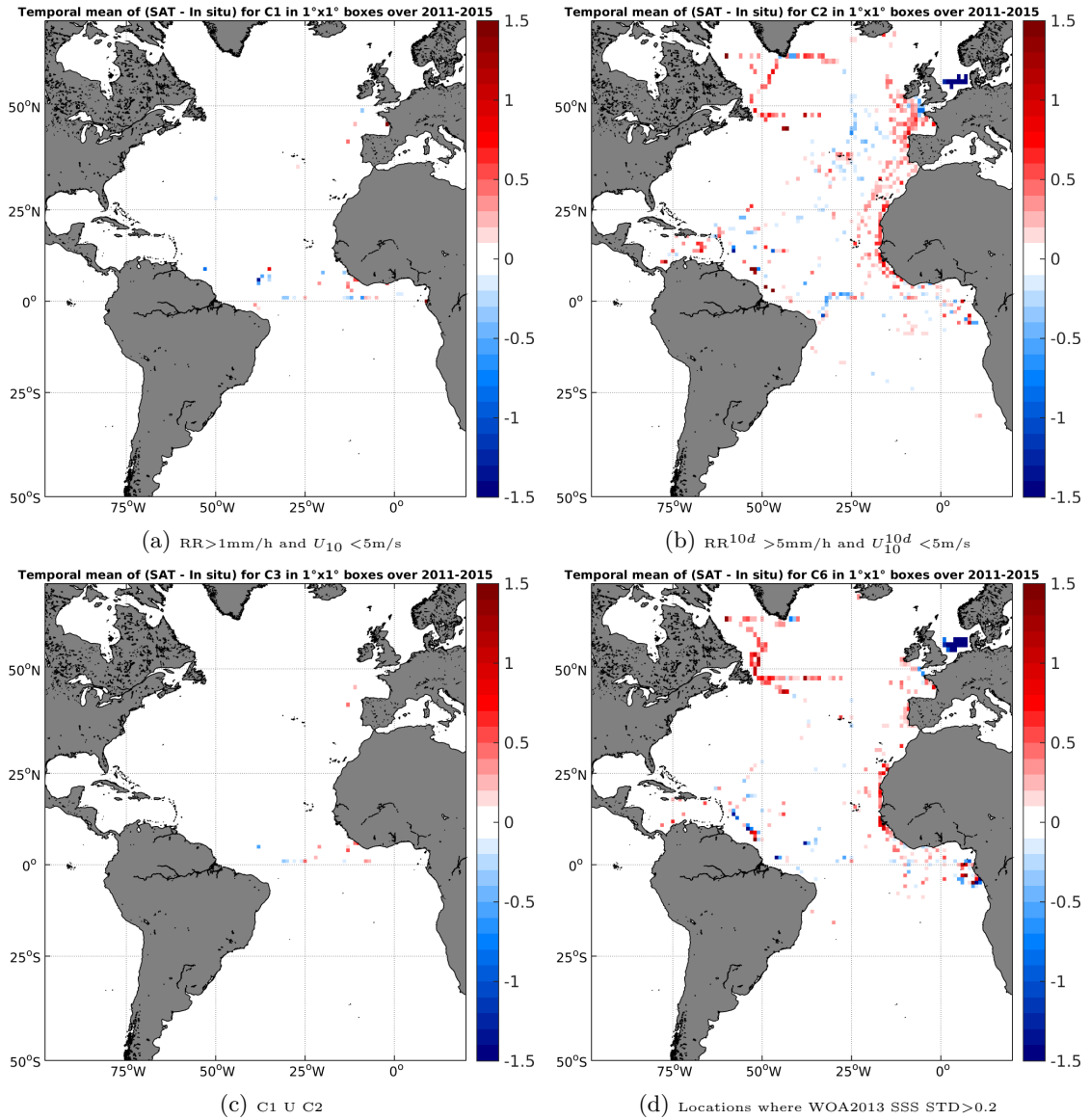
Figure 12: Temporal mean gridded over spatial boxes of size 1°x1° of \Delta\text{SSS} (Aquarius-L3-JPL-V4-MONTHLY - TSG-GOSUD-Research-vessel) for 4 different subdatasets corresponding to: RR > 1\text{mm/h} and U_{10} < 5\text{m/s} (a), RR^{10d} > 5\text{mm/h} and U_{10}^{10d} < 5\text{m/s} (b), C1 U C2 (c), Locations where WOA2013 SSS STD > 0.2 (d).
