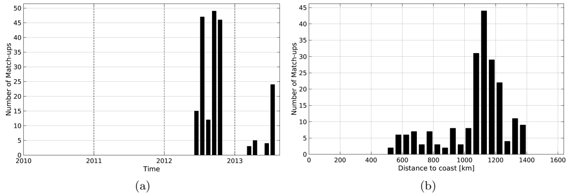
Figure 1: Number of match-ups between Sea mammals and Aquarius-L3-JPL-V4-MONTHLY SSS as a function of time (a) and as function of the distance to coast (b) over the Atlantic Ocean Pi-MEP region and for the full satellite product period.
