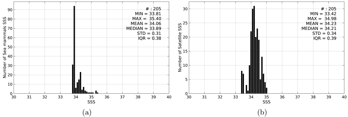
Figure 2: Histograms of SSS from Sea mammals (a) and Aquarius-L3-JPL-V4-MONTHLY (b) considering all match-up pairs per bins of 0.1 over the Atlantic Ocean Pi-MEP region and for the full satellite product period.
