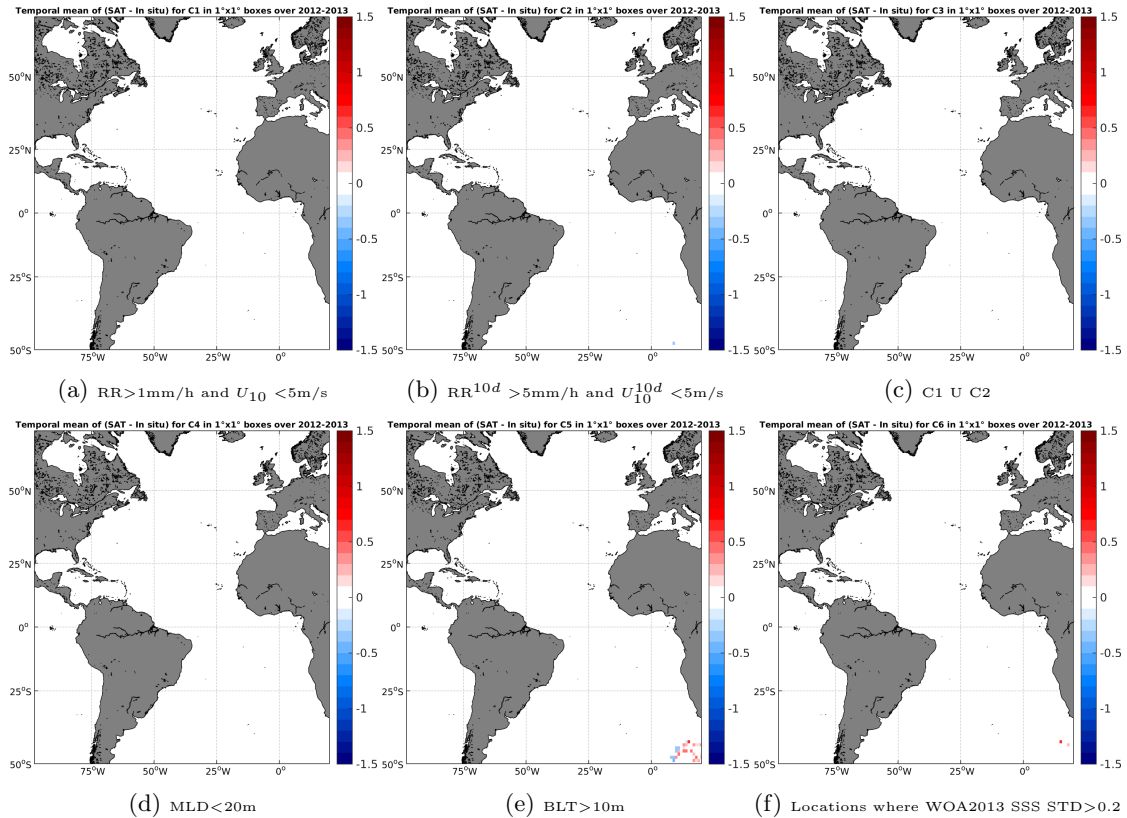
Figure 12: Temporal mean gridded over spatial boxes of size 1^\circ \times 1^\circ of \Delta SSS (Aquarius-L3-JPL-V4-MONTHLY - Sea mammals) for 6 different subdatasets corresponding to: RR > 1mm/h and U_{10} < 5\text{m/s} (a), RR^{10d} > 5\text{mm/h} and U_{10}^{10d} < 5\text{m/s} (b), C1 U C2 (c), MLD < 20m (d), BLT > 10m (e), Locations where WOA2013 SSS STD > 0.2 (f).
