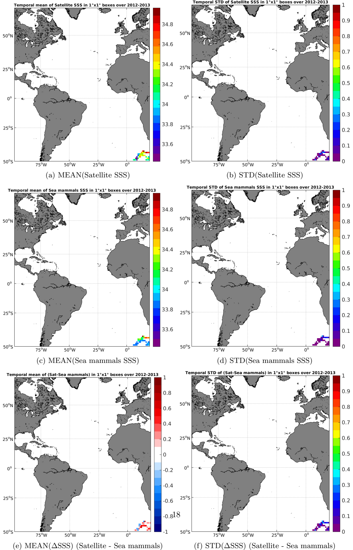
Figure 6: Temporal mean (left) and STD (right) of SSS from Aquarius-L3-JPL-V4-MONTHLY (top), Sea mammals (middle), and of \Delta SSS (Satellite - Sea mammals). Only match-up pairs are used to generate these maps.
