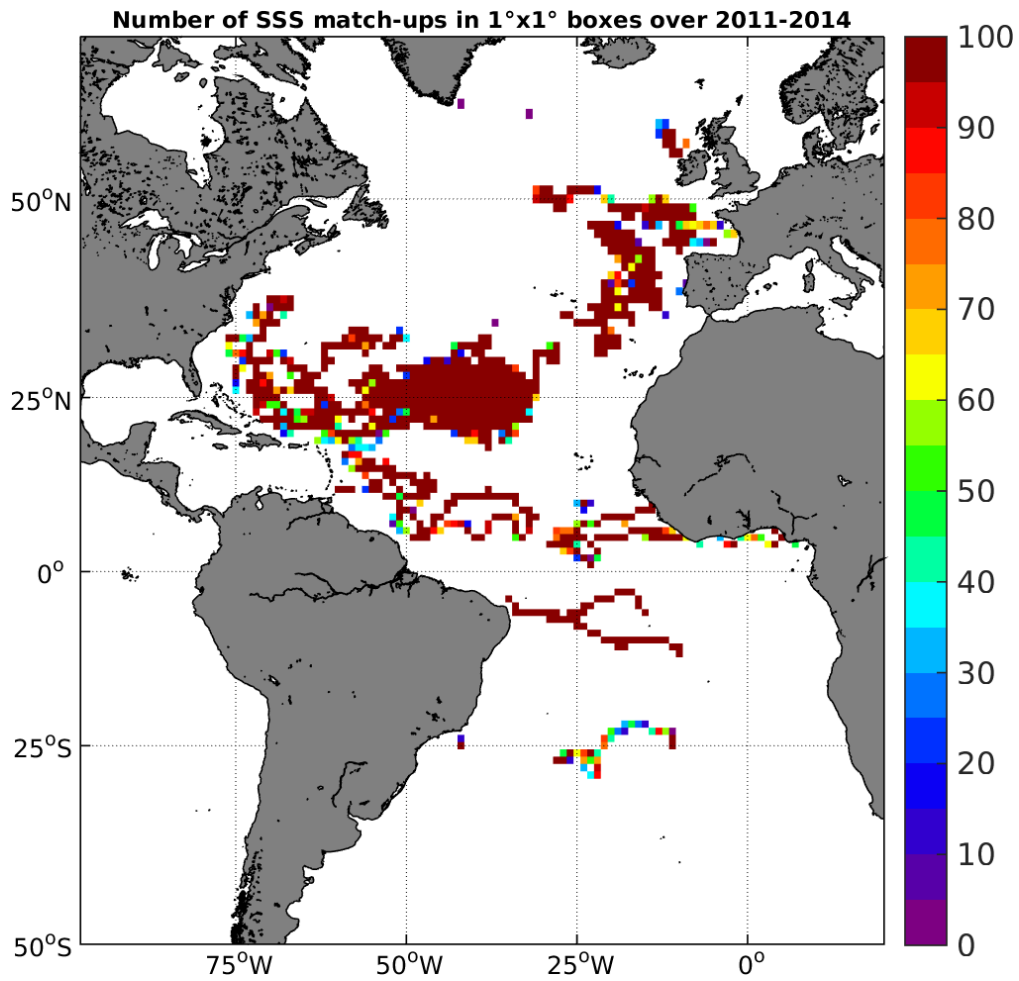
Figure 3: Number of SSS match-ups between Surface drifters SSS and the Aquarius-L3-JPL-V4-MONTHLY SSS product for the Atlantic Ocean Pi-MEP region over 1°x1° boxes and for the full satellite product period.
