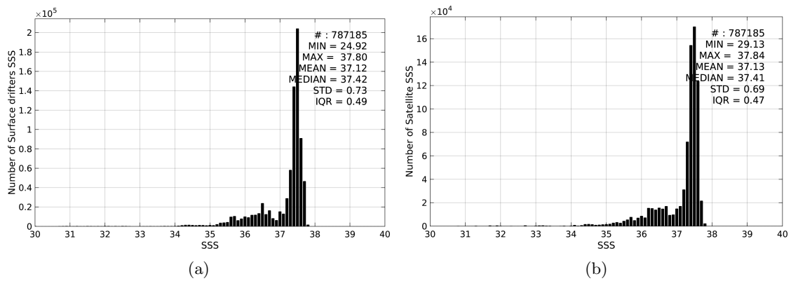
Figure 2: Histograms of SSS from Surface drifters (a) and Aquarius-L3-JPL-V4-MONTHLY (b) considering all match-up pairs per bins of 0.1 over the Atlantic Ocean Pi-MEP region and for the full satellite product period.
