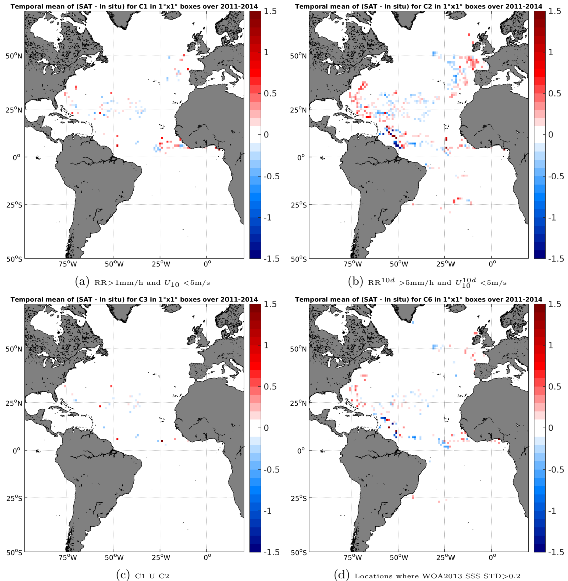
Figure 11: Temporal mean gridded over spatial boxes of size 1^\circ \times 1^\circ of \Delta SSS (Aquarius-L3-JPL-V4-MONTHLY - Surface drifters) for 4 different subdatasets corresponding to:RR >1 mm/h and U_{10} < 5 m/s (a), RR 10d > 5 mm/h and U_{10}^{10d} < 5 m/s (b), C1 U C2 (c),Locations where WOA2013 SSS STD > 0.2 (d).
