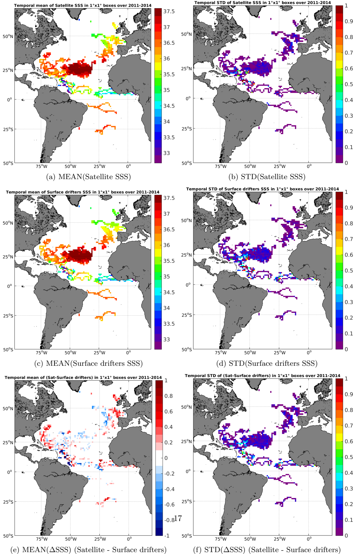
Figure 5: Temporal mean (left) and STD (right) of SSS from Aquarius-L3-JPL-V4-MONTHLY (top), Surface drifters (middle), and of \Delta SSS (Satellite - Surface drifters). Only match-up pairs are used to generate these maps.
