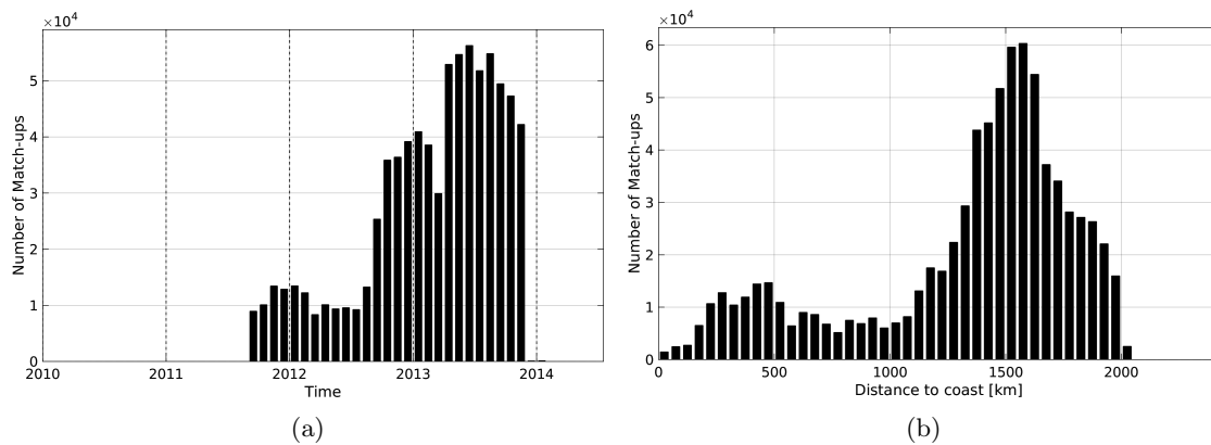
Figure 1: Number of match-ups between Surface drifters and Aquarius-L3-JPL-V4-MONTHLY SSS as a function of time (a) and as function of the distance to coast (b) over the Atlantic Ocean Pi-MEP region and for the full satellite product period.
