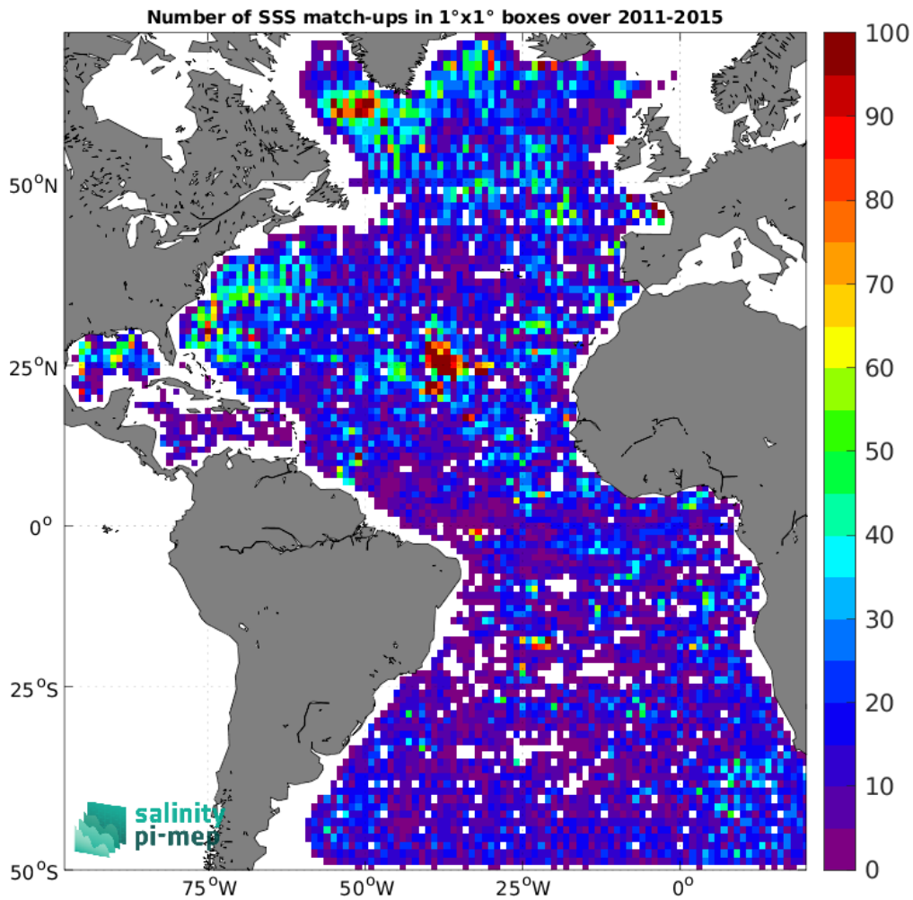
Figure 4: Number of SSS match-ups between Argo SSS and the Aquarius SSS L2-AVERAGED OR v5 (NASA-GSFC) SSS product for the Atlantic Ocean Pi-MEP region over 1^\circ \times 1^\circ boxes and for the full satellite product period.
