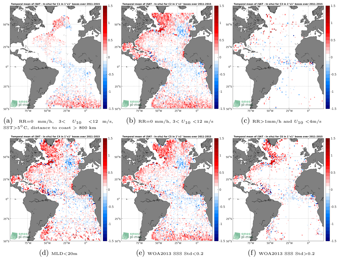
Figure 12: Temporal mean gridded over spatial boxes of size 1^\circ \times 1^\circ of \Delta SSS (Aquarius SSS L2-AVERAGED CAP v5 (JPL) - Argo) for 6 different subdatasets corresponding to:RR=0 mm/h, 3 < U_{10} < 12 m/s, SST >5^\circ C, distance to coast > 800 km (a), RR=0 mm/h, 3 < U_{10} < 12 m/s (b), RR >1 mm/h and U_{10} < 4 m/s (c),MLD <20 m (d),WOA2013 SSS Std <0.2 (e),WOA2013 SSS Std >0.2 (f).
