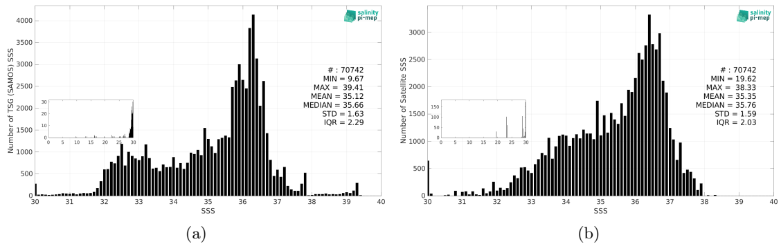
Figure 3: Histograms of SSS from TSG (SAMOS) (a) and Aquarius SSS L2 OR v5 (NASA-GSFC) (b) considering all match-up pairs per bins of 0.1 over the Atlantic Ocean Pi-MEP region and for the full satellite product period.
