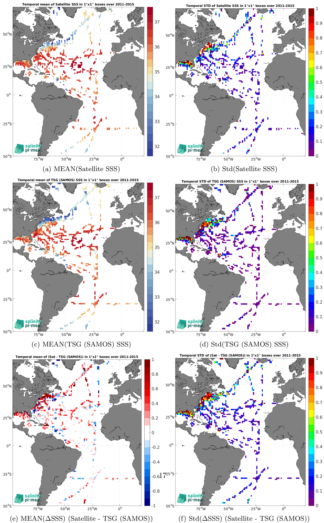
Figure 7: Temporal mean (left) and Std (right) of SSS from Aquarius SSS L2 OR v5 (NASA-GSFC) (top), TSG (SAMOS) (middle), and of \Delta SSS (Satellite - TSG (SAMOS)). Only match-up pairs are used to generate these maps.
