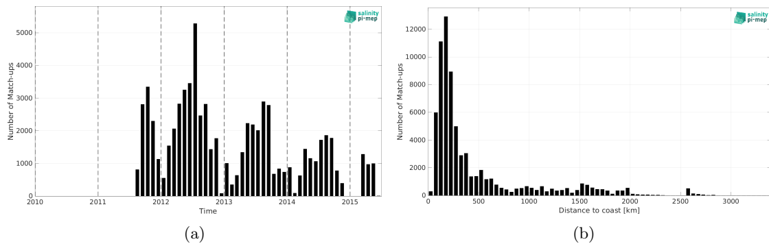
Figure 2: Number of match-ups between TSG (SAMOS) and Aquarius SSS L2 OR v5 (NASA-GSFC) SSS as a function of time (a) and as function of the distance to coast (b) over the Atlantic Ocean Pi-MEP region and for the full satellite product period.
