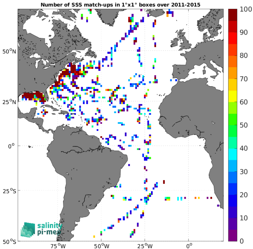
Figure 5: Number of SSS match-ups between TSG (SAMOS) SSS and the Aquarius SSS L2 OR v5 (NASA-GSFC) SSS product for the Atlantic Ocean Pi-MEP region over 1^\circ \times 1^\circ boxes and for the full satellite product period.
