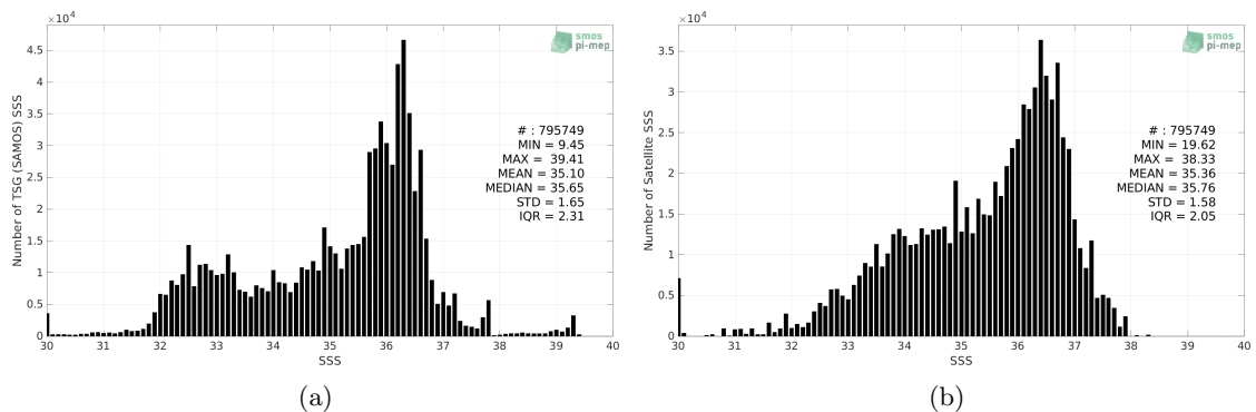
Figure 2: Histograms of SSS from TSG (SAMOS) (a) and Aquarius SSS L2 OR v5 (NASA-GSFC) (b) considering all match-up pairs per bins of 0.1 over the Atlantic Ocean Pi-MEP region and for the full satellite product period.
