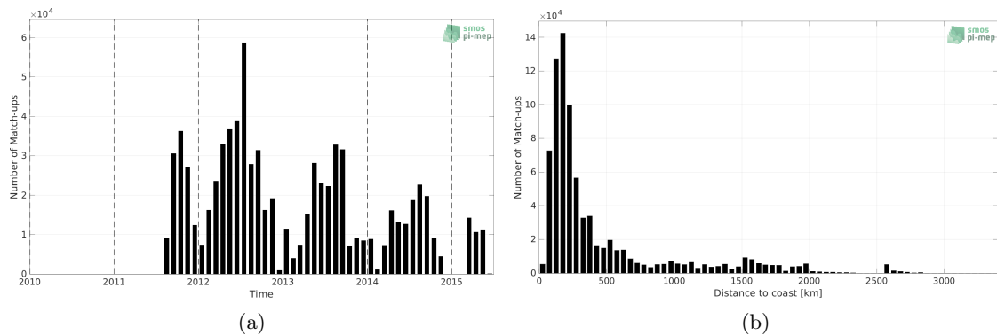
Figure 1: Number of match-ups between TSG (SAMOS) and Aquarius SSS L2 OR v5 (NASA-GSFC) SSS as a function of time (a) and as function of the distance to coast (b) over the Atlantic Ocean Pi-MEP region and for the full satellite product period.
