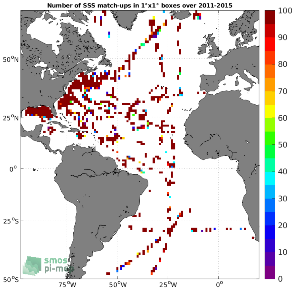
Figure 4: Number of SSS match-ups between TSG (SAMOS) SSS and the Aquarius SSS L2 OR v5 (NASA-GSFC) SSS product for the Atlantic Ocean Pi-MEP region over 1°x1° boxes and for the full satellite product period.
