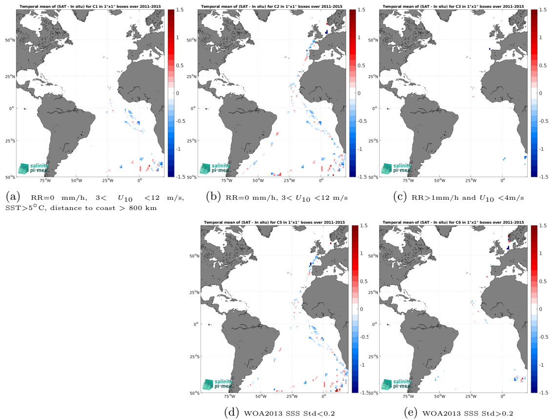
Figure 14: Temporal mean gridded over spatial boxes of size 1^\circ \times 1^\circ of \Delta\text{SSS} (Aquarius SSS L2 OR v5 (NASA-GSFC) - TSG (Polarstern)) for 5 different subdatasets corresponding to:RR=0 mm/h, 3 < U_{10} < 12 m/s, SST >5^\circ\text{C} , distance to coast > 800 km (a), RR=0 mm/h, 3 < U_{10} < 12 m/s (b), RR >1 mm/h and U_{10} < 4 m/s (c), WOA2013 SSS Std <0.2 (d), WOA2013 SSS Std >0.2 (e).
