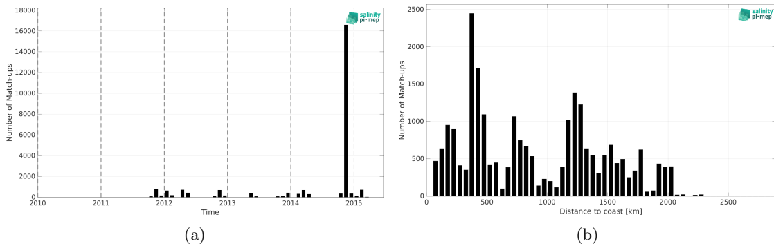
Figure 2: Number of match-ups between TSG (Polarstern) and Aquarius SSS L2 OR v5 (NASA-GSFC) SSS as a function of time (a) and as function of the distance to coast (b) over the Atlantic Ocean Pi-MEP region and for the full satellite product period.
