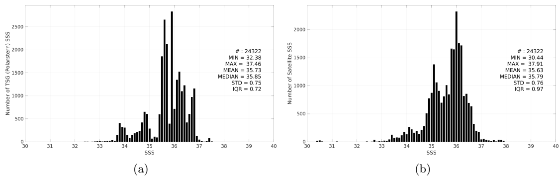
Figure 3: Histograms of SSS from TSG (Polarstern) (a) and Aquarius SSS L2 OR v5 (NASA-GSFC) (b) considering all match-up pairs per bins of 0.1 over the Atlantic Ocean Pi-MEP region and for the full satellite product period.
