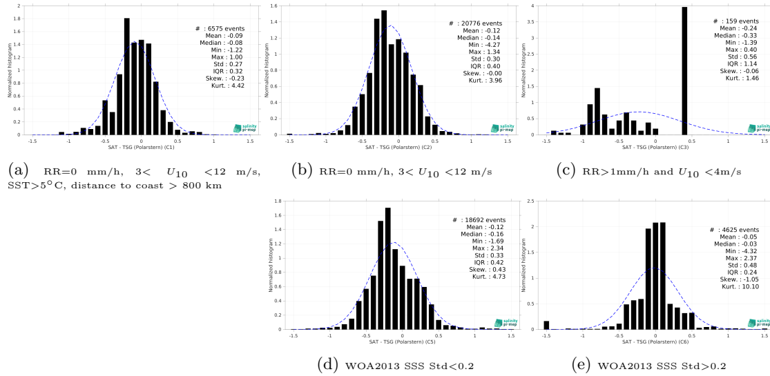
Figure 15: Normalized histogram of \Delta SSS (Aquarius SSS L2 OR v5 (NASA-GSFC) - TSG (Polarstern)) for 5 different subdatasets corresponding to: RR=0 mm/h, 3 < U_{10} < 12 m/s, SST>5°C, distance to coast > 800 km (a), RR=0 mm/h, 3 < U_{10} < 12 m/s (b), RR>1mm/h and U_{10} < 4 m/s (c), WOA2013 SSS Std<0.2 (d), WOA2013 SSS Std>0.2 (e).
