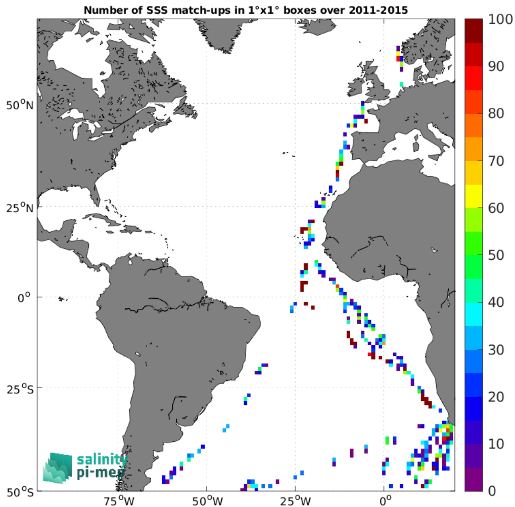
Figure 5: Number of SSS match-ups between TSG (Polarstern) SSS and the Aquarius SSS L2 OR v5 (NASA-GSFC) SSS product for the Atlantic Ocean Pi-MEP region over 1°×1° boxes and for the full satellite product period.
