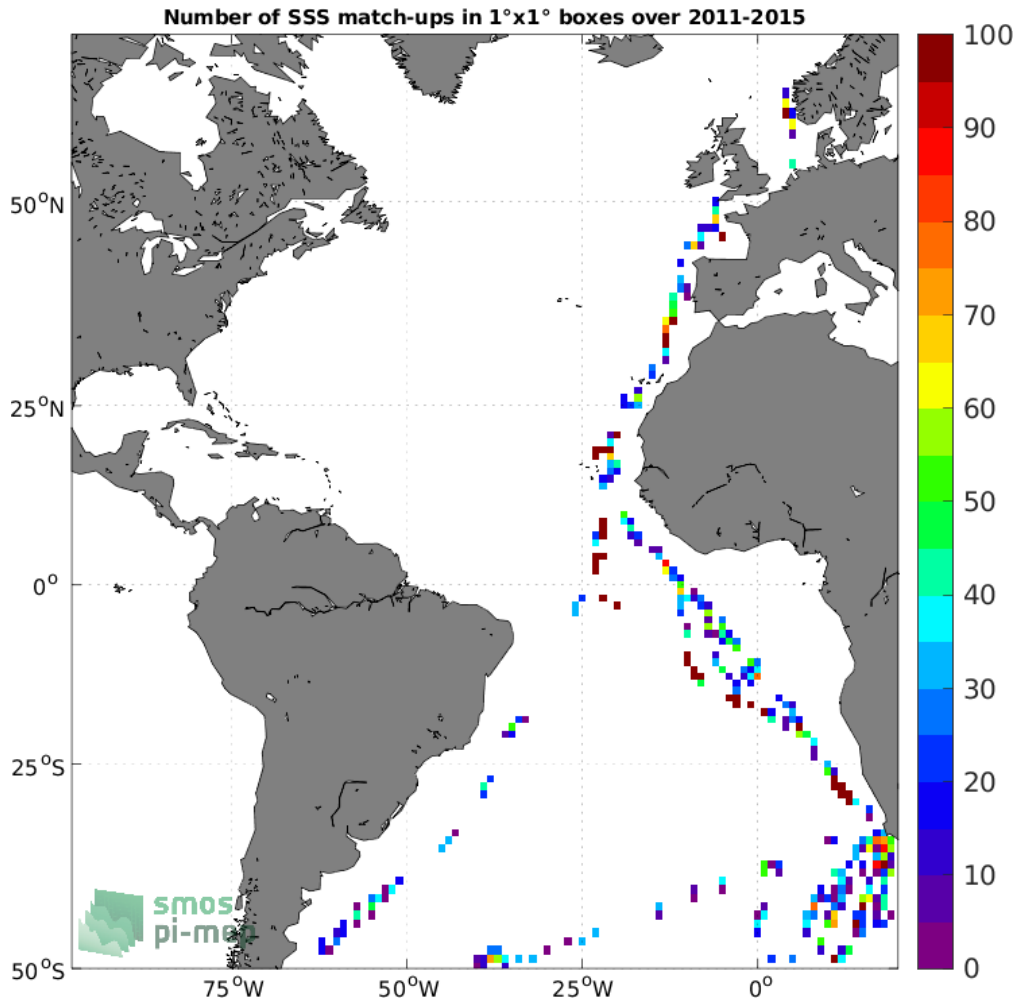
Figure 4: Number of SSS match-ups between TSG (Polarstern) SSS and the Aquarius SSS L2 OR v5 (NASA-GSFC) SSS product for the Atlantic Ocean Pi-MEP region over 1^\circ \times 1^\circ boxes and for the full satellite product period.
