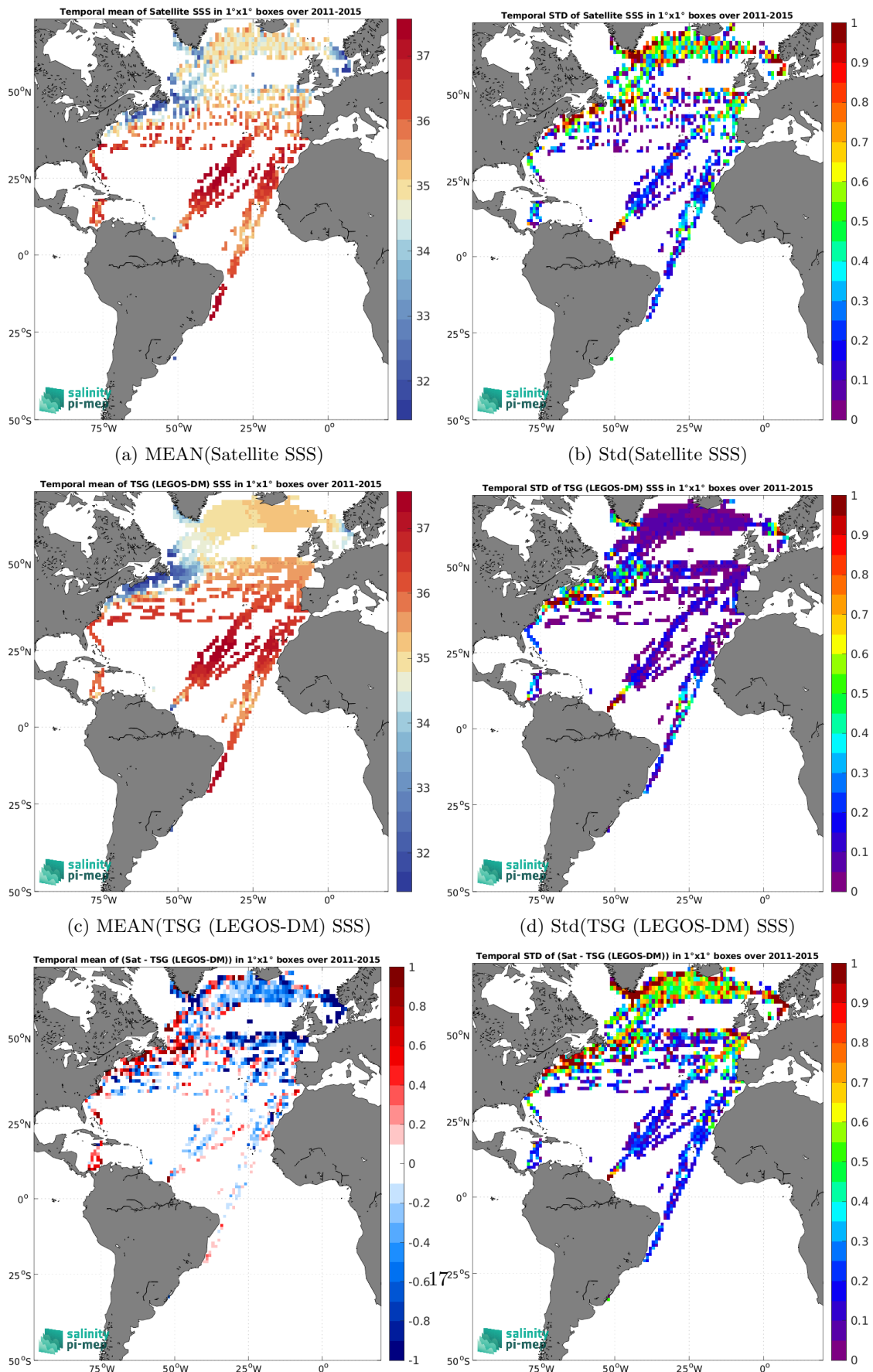
(e) MEAN( \Delta SSS) (Satellite - TSG (LEGOS-DM)) (f) Std( \Delta SSS) (Satellite - TSG (LEGOS-DM)) Figure 7: Temporal mean (left) and Std (right) of SSS from Aquarius SSS L2 OR v5 (NASA-GSFC) (top), TSG (LEGOS-DM) (middle), and of \Delta SSS (Satellite - TSG (LEGOS-DM)). Only match-up pairs are used to generate these maps.
