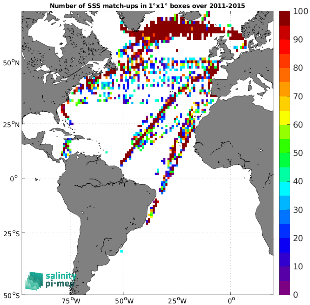
Figure 5: Number of SSS match-ups between TSG (LEGOS-DM) SSS and the Aquarius SSS L2 OR v5 (NASA-GSFC) SSS product for the Atlantic Ocean Pi-MEP region over 1°×1° boxes and for the full satellite product period.
