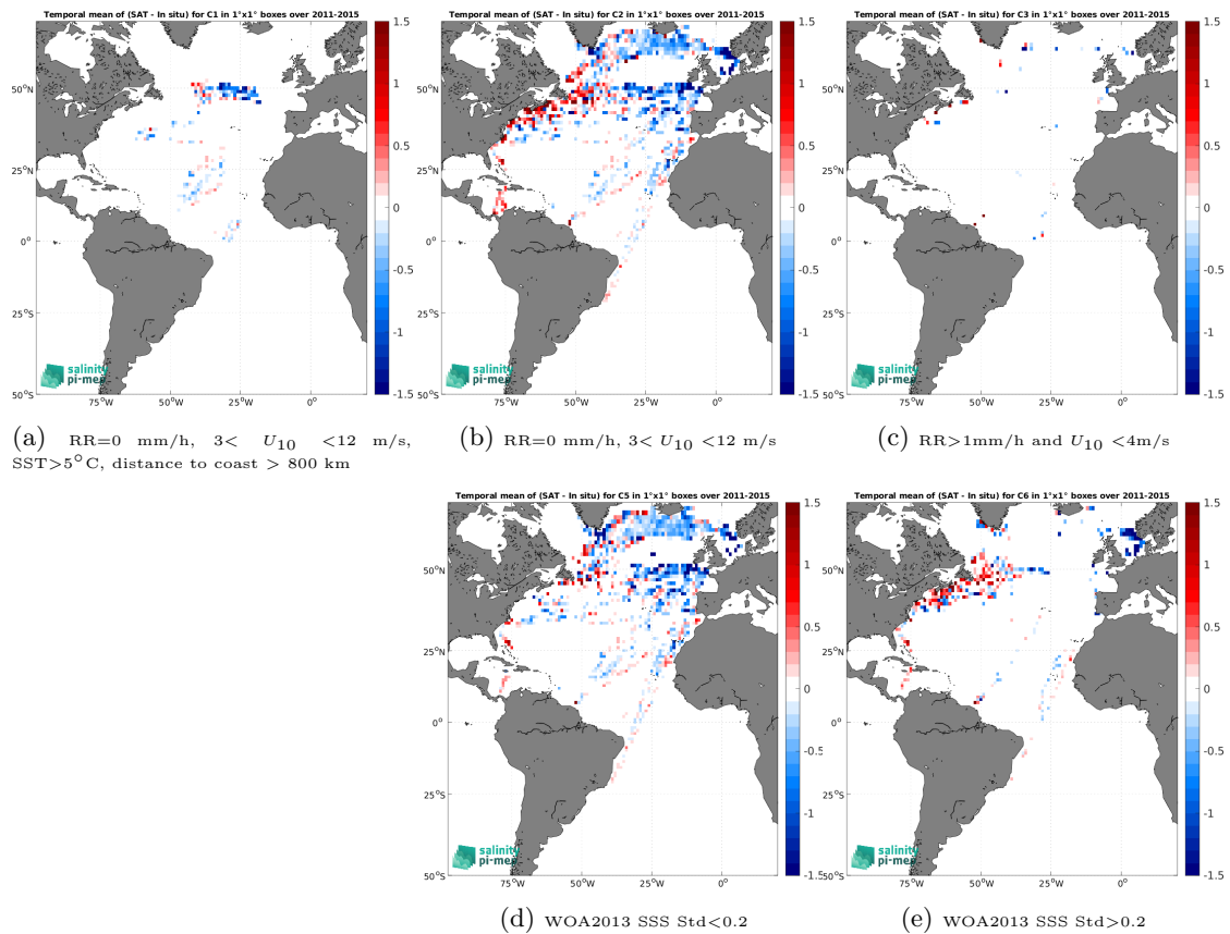
Figure 14: Temporal mean gridded over spatial boxes of size 1^\circ \times 1^\circ of \Delta\text{SSS} (Aquarius SSS L2 OR v5 (NASA-GSFC) - TSG (LEGOS-DM)) for 5 different subdatasets corresponding to:RR=0 mm/h, 3 < U_{10} < 12 m/s, SST >5^\circ\text{C} , distance to coast > 800 km (a), RR=0 mm/h, 3 < U_{10} < 12 m/s (b), RR >1 mm/h and U_{10} < 4 m/s (c), WOA2013 SSS Std <0.2 (d), WOA2013 SSS Std >0.2 (e).
