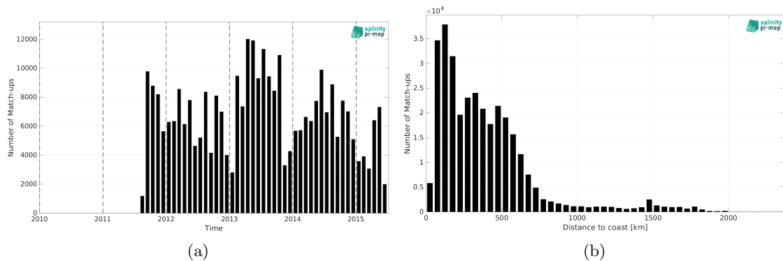
Figure 2: Number of match-ups between TSG (LEGOS-DM) and Aquarius SSS L2 OR v5 (NASA-GSFC) SSS as a function of time (a) and as function of the distance to coast (b) over the Atlantic Ocean Pi-MEP region and for the full satellite product period.
