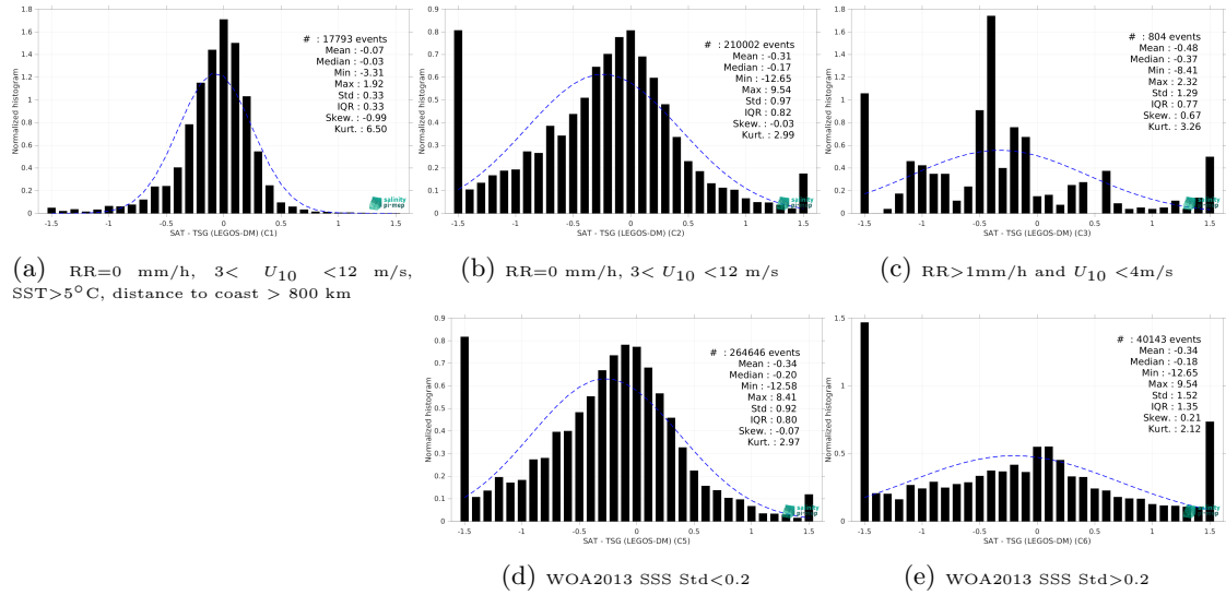
Figure 15: Normalized histogram of \Delta\text{SSS} (Aquarius SSS L2 OR v5 (NASA-GSFC) - TSG (LEGOS-DM)) for 5 different subdatasets corresponding to: RR=0 mm/h, 3 < U_{10} < 12 m/s, SST > 5°C, distance to coast > 800 km (a), RR=0 mm/h, 3 < U_{10} < 12 m/s (b), RR > 1mm/h and U_{10} < 4 m/s (c), WOA2013 SSS Std < 0.2 (d), WOA2013 SSS Std > 0.2 (e).
