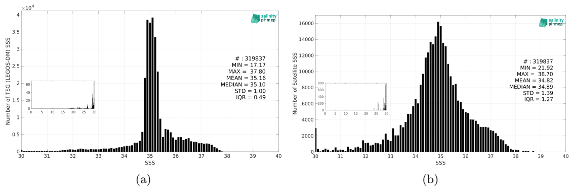
Figure 3: Histograms of SSS from TSG (LEGOS-DM) (a) and Aquarius SSS L2 OR v5 (NASA-GSFC) (b) considering all match-up pairs per bins of 0.1 over the Atlantic Ocean Pi-MEP region and for the full satellite product period.
