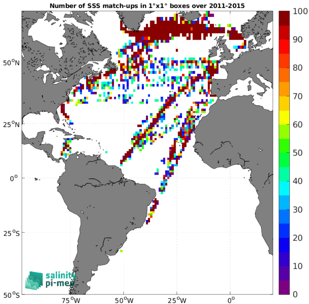
Figure 4: Number of SSS match-ups between TSG (LEGOS-DM) SSS and the Aquarius SSS L2 OR v5 (NASA-GSFC) SSS product for the Atlantic Ocean Pi-MEP region over 1^{\circ} \times 1^{\circ} boxes and for the full satellite product period.
