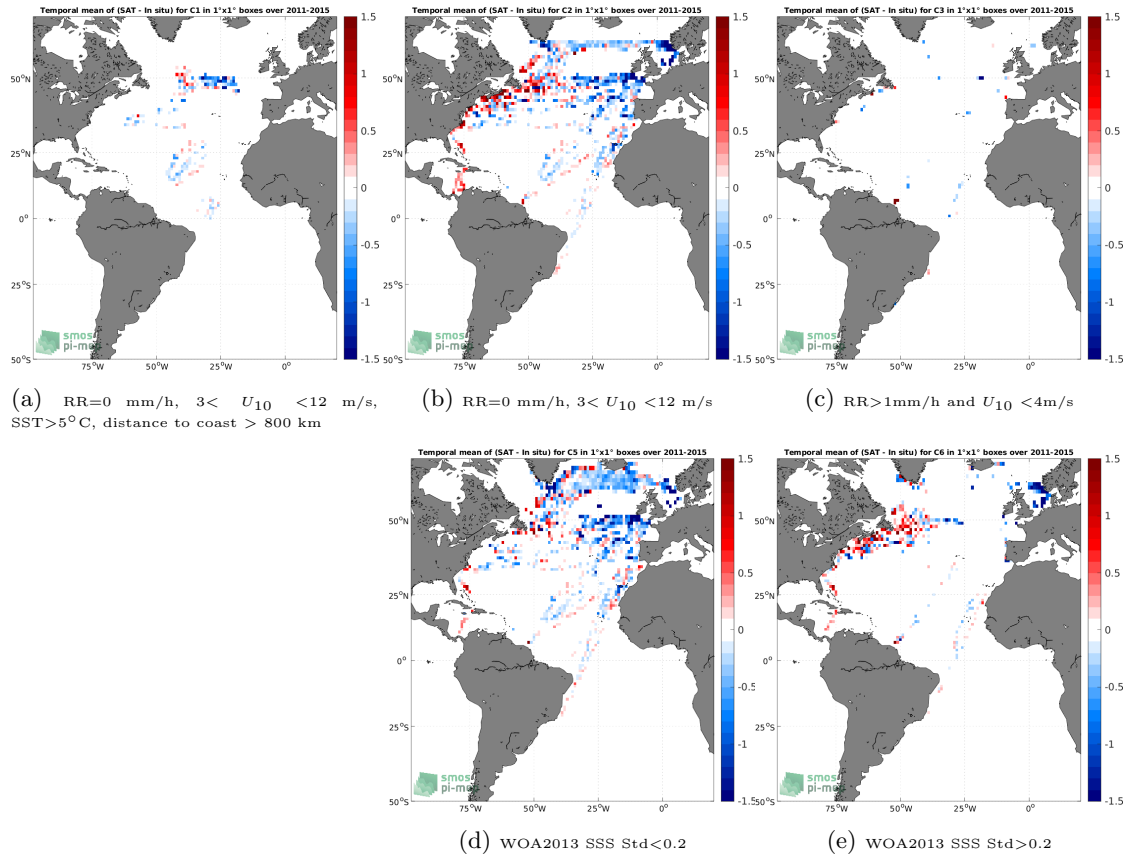
Figure 12: Temporal mean gridded over spatial boxes of size 1^\circ \times 1^\circ of \Delta SSS (Aquarius SSS L2 OR v5 (NASA-GSFC) - TSG (LEGOS-DM)) for 5 different subdatasets corresponding to:RR=0 mm/h, 3 < U_{10} < 12 m/s, SST >5^\circ\text{C} , distance to coast > 800 km (a), RR=0 mm/h, 3 < U_{10} < 12 m/s (b), RR >1 mm/h and U_{10} < 4 m/s (c), WOA2013 SSS Std <0.2 (d), WOA2013 SSS Std >0.2 (e).
