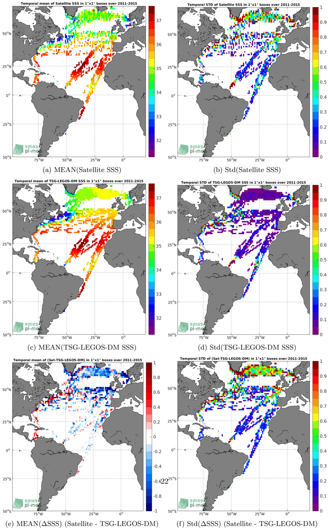
Figure 6: Temporal mean (left) and Std (right) of SSS from Aquarius-L2-OR-V5 (top), TSG-LEGOS-DM (middle), and of \Delta SSS (Satellite - TSG-LEGOS-DM). Only match-up pairs are used to generate these maps.
