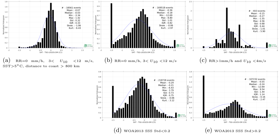
Figure 13: Normalized histogram of \Delta\text{SSS} (Aquarius-L2-OR-V5 - TSG-LEGOS-DM) for 5 different subdatasets corresponding to: RR=0 mm/h, 3 < U_{10} < 12 m/s, SST > 5^\circ\text{C} , distance to coast > 800 km (a), RR=0 mm/h, 3 < U_{10} < 12 m/s (b), RR > 1 mm/h and U_{10} < 4 m/s (c), WOA2013 SSS Std < 0.2 (d), WOA2013 SSS Std > 0.2 (e).
