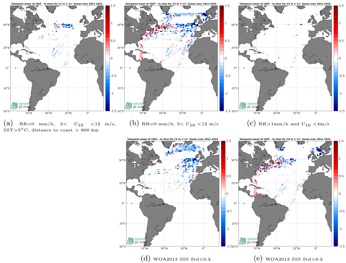
Figure 12: Temporal mean gridded over spatial boxes of size 1^\circ \times 1^\circ of \Delta SSS (Aquarius-L2-OR-V5 - TSG-LEGOS-DM) for 5 different subdatasets corresponding to:RR=0 mm/h, 3 < U_{10} < 12 m/s, SST >5^\circ\text{C} , distance to coast > 800 km (a), RR=0 mm/h, 3 < U_{10} < 12 m/s (b), RR >1 mm/h and U_{10} < 4 m/s (c), WOA2013 SSS Std <0.2 (d), WOA2013 SSS Std >0.2 (e).
