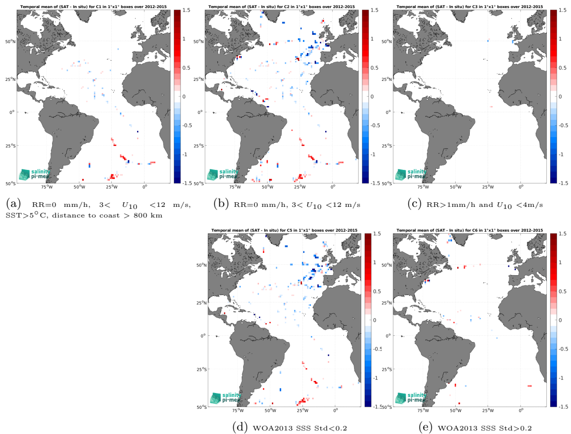
Figure 14: Temporal mean gridded over spatial boxes of size 1^\circ \times 1^\circ of \Delta\text{SSS} (Aquarius SSS L2 OR v5 (NASA-GSFC) - TSG (GOSUD-Sailing-ship)) for 5 different subdatasets corresponding to:RR=0 mm/h, 3 < U_{10} < 12 m/s, SST>5°C, distance to coast > 800 km (a), RR=0 mm/h, 3 < U_{10} < 12 m/s (b), RR>1mm/h and U_{10} < 4 m/s (c), WOA2013 SSS Std<0.2 (d), WOA2013 SSS Std>0.2 (e).
