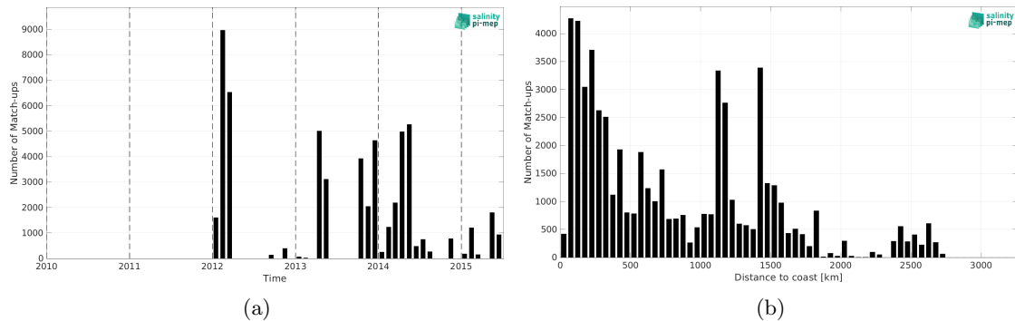
Figure 2: Number of match-ups between TSG (GOSUD-Sailing-ship) and Aquarius SSS L2 OR v5 (NASA-GSFC) SSS as a function of time (a) and as function of the distance to coast (b) over the Atlantic Ocean Pi-MEP region and for the full satellite product period.
