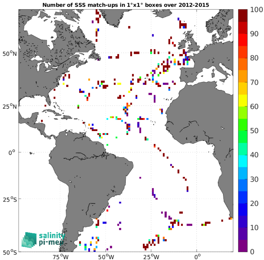
Figure 5: Number of SSS match-ups between TSG (GOSUD-Sailing-ship) SSS and the Aquarius SSS L2 OR v5 (NASA-GSFC) SSS product for the Atlantic Ocean Pi-MEP region over 1^\circ \times 1^\circ boxes and for the full satellite product period.
