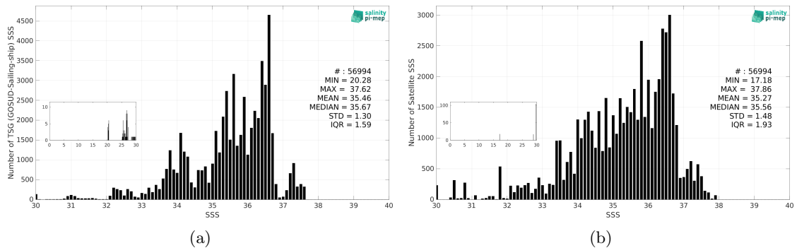
Figure 3: Histograms of SSS from TSG (GOSUD-Sailing-ship) (a) and Aquarius SSS L2 OR v5 (NASA-GSFC) (b) considering all match-up pairs per bins of 0.1 over the Atlantic Ocean Pi-MEP region and for the full satellite product period.
