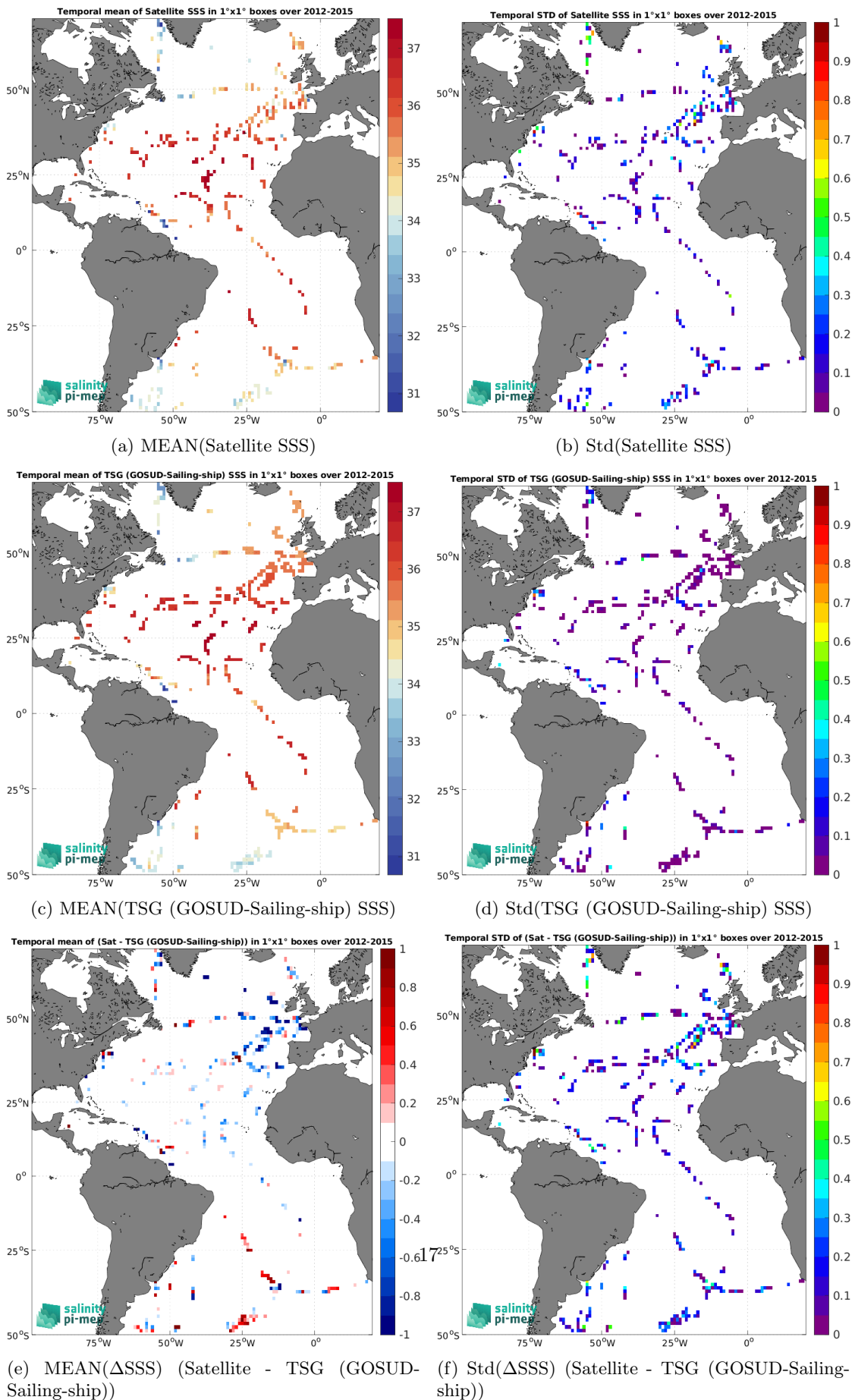
Figure 7: Temporal mean (left) and Std (right) of SSS from Aquarius SSS L2 OR v5 (NASA-GSFC) (top), TSG (GOSUD-Sailing-ship) (middle), and of \Delta SSS (Satellite - TSG (GOSUD-Sailing-ship)). Only match-up pairs are used to generate these maps.
