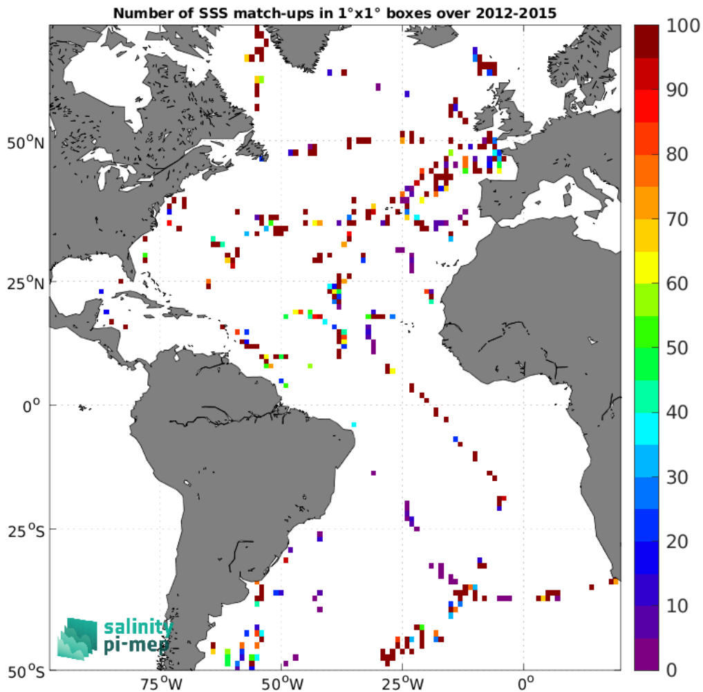
Figure 4: Number of SSS match-ups between TSG (GOSUD-Sailing-ship) SSS and the Aquarius SSS L2 OR v5 (NASA-GSFC) SSS product for the Atlantic Ocean Pi-MEP region over 1°x1° boxes and for the full satellite product period.
