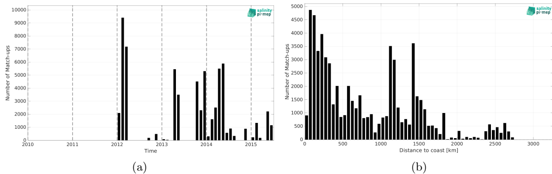
Figure 1: Number of match-ups between TSG (GOSUD-Sailing-ship) and Aquarius SSS L2 OR v5 (NASA-GSFC) SSS as a function of time (a) and as function of the distance to coast (b) over the Atlantic Ocean Pi-MEP region and for the full satellite product period.
