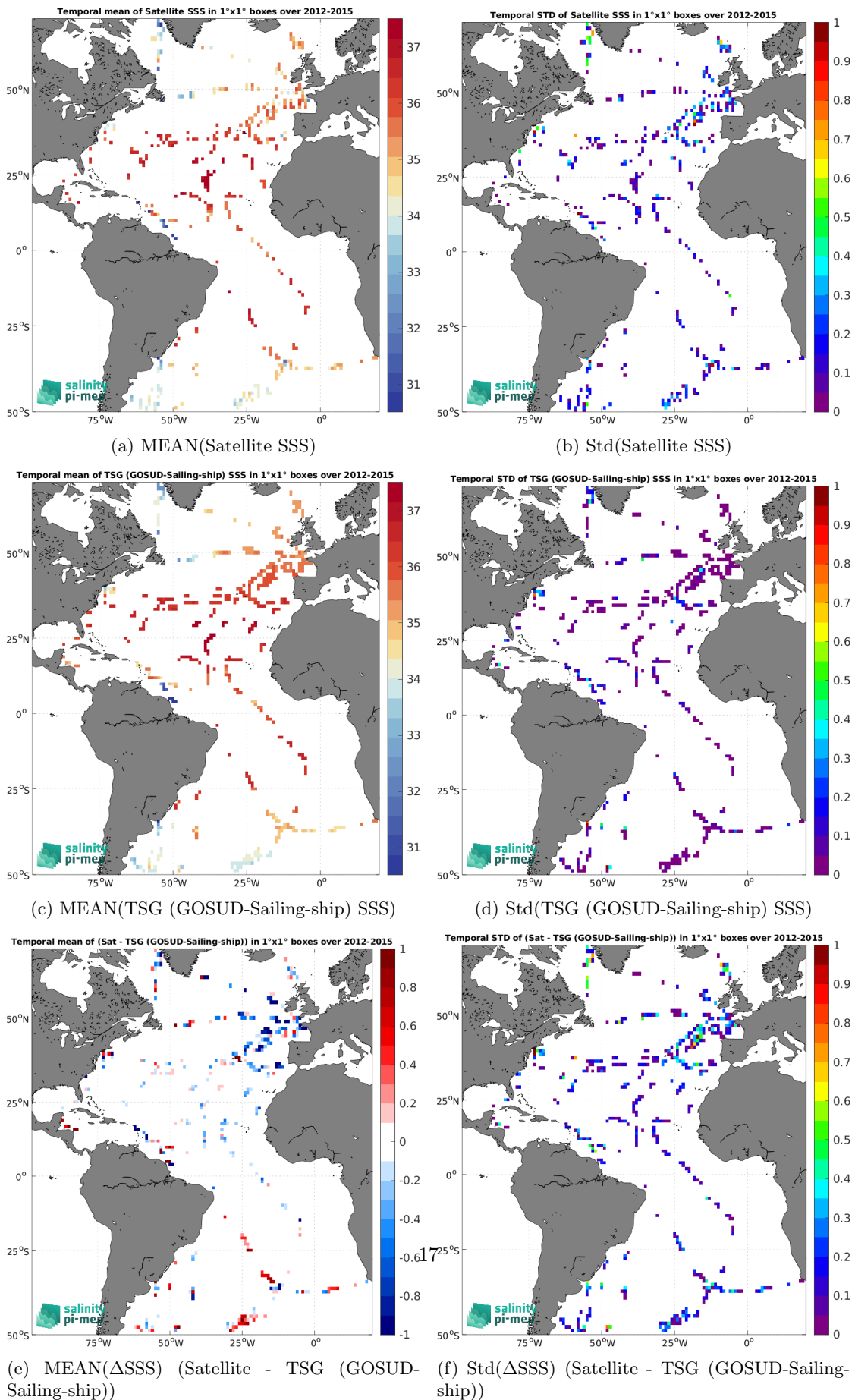
Figure 6: Temporal mean (left) and Std (right) of SSS from Aquarius SSS L2 OR v5 (NASA-GSFC) (top), TSG (GOSUD-Sailing-ship) (middle), and of \Delta SSS (Satellite - TSG (GOSUD-Sailing-ship)). Only match-up pairs are used to generate these maps.
