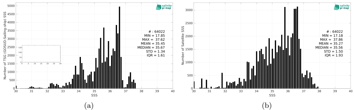
Figure 2: Histograms of SSS from TSG (GOSUD-Sailing-ship) (a) and Aquarius SSS L2 OR v5 (NASA-GSFC) (b) considering all match-up pairs per bins of 0.1 over the Atlantic Ocean Pi-MEP region and for the full satellite product period.
