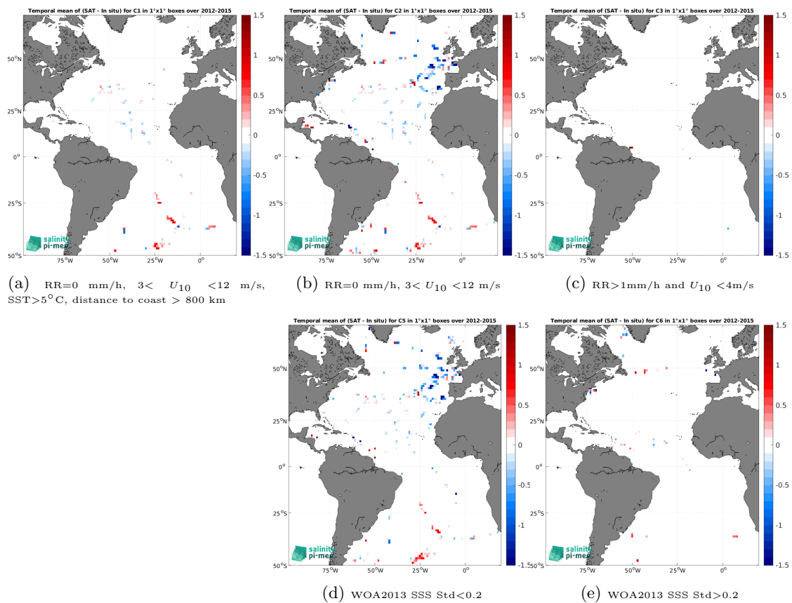
Figure 12: Temporal mean gridded over spatial boxes of size 1^\circ \times 1^\circ of \Delta\text{SSS} (Aquarius SSS L2 OR v5 (NASA-GSFC) - TSG (GOSUD-Sailing-ship)) for 5 different subdatasets corresponding to:RR=0 mm/h, 3 < U_{10} < 12 m/s, SST>5°C, distance to coast > 800 km (a), RR=0 mm/h, 3 < U_{10} < 12 m/s (b), RR>1mm/h and U_{10} < 4 m/s (c), WOA2013 SSS Std<0.2 (d), WOA2013 SSS Std>0.2 (e).
