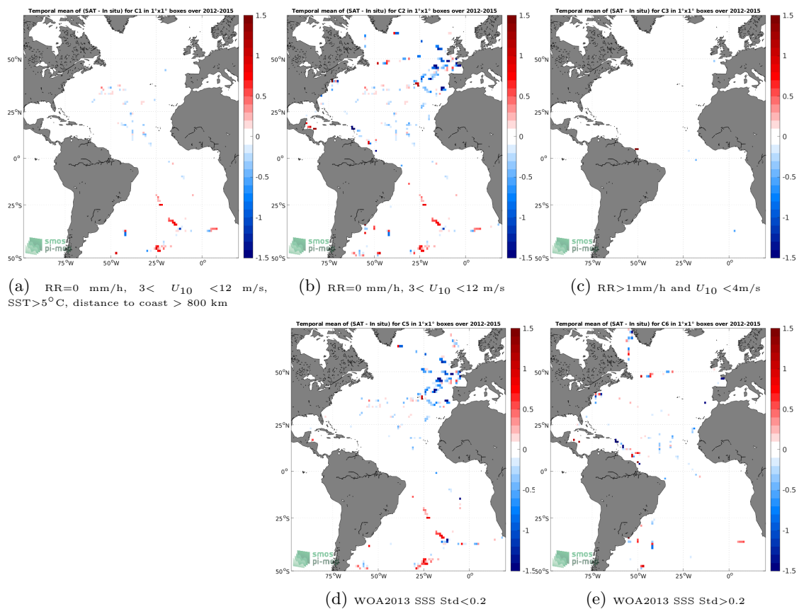
Figure 12: Temporal mean gridded over spatial boxes of size 1^\circ \times 1^\circ of \Delta SSS (Aquarius SSS L2 OR v5 (NASA-GSFC) - TSG (GOSUD-Sailing-ship)) for 5 different subdatasets corresponding to:RR=0 mm/h, 3 < U_{10} < 12 m/s, SST>5°C, distance to coast > 800 km (a), RR=0 mm/h, 3 < U_{10} < 12 m/s (b), RR>1mm/h and U_{10} < 4 m/s (c), WOA2013 SSS Std<0.2 (d), WOA2013 SSS Std>0.2 (e).
