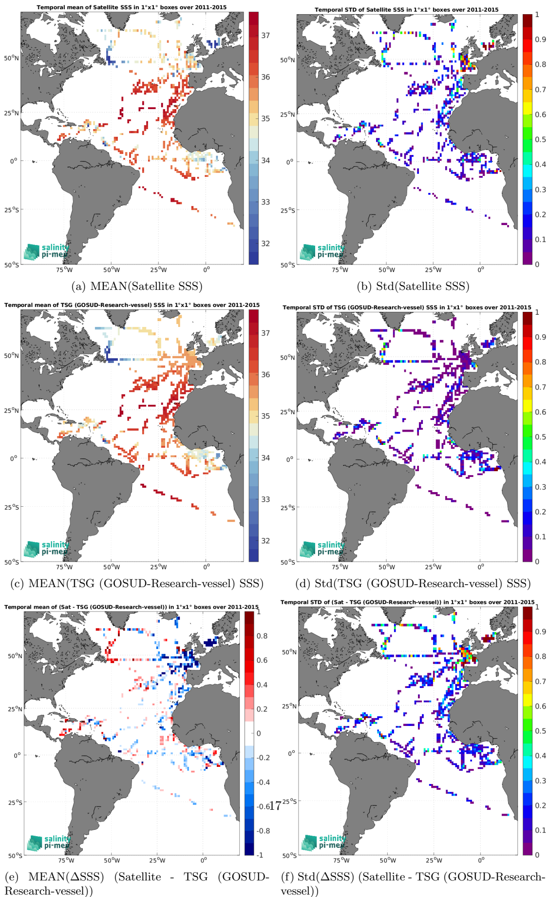
Figure 6: Temporal mean (left) and Std (right) of SSS from Aquarius SSS L2 OR v5 (NASA-GSFC) (top), TSG (GOSUD-Research-vessel) (middle), and of \Delta SSS (Satellite - TSG (GOSUD-Research-vessel)). Only match-up pairs are used to generate these maps.
