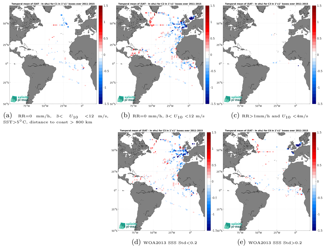
Figure 12: Temporal mean gridded over spatial boxes of size 1^\circ \times 1^\circ of \Delta\text{SSS} (Aquarius SSS L2 OR v5 (NASA-GSFC) - TSG (GOSUD-Research-vessel)) for 5 different subdatasets corresponding to:RR=0 mm/h, 3 < U_{10} < 12 m/s, SST>5°C, distance to coast > 800 km (a), RR=0 mm/h, 3 < U_{10} < 12 m/s (b), RR>1mm/h and U_{10} < 4 m/s (c), WOA2013 SSS Std<0.2 (d), WOA2013 SSS Std>0.2 (e).
