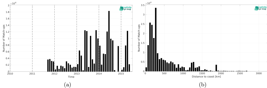
Figure 1: Number of match-ups between TSG (GOSUD-Research-vessel) and Aquarius SSS L2 OR v5 (NASA-GSFC) SSS as a function of time (a) and as function of the distance to coast (b) over the Atlantic Ocean Pi-MEP region and for the full satellite product period.
