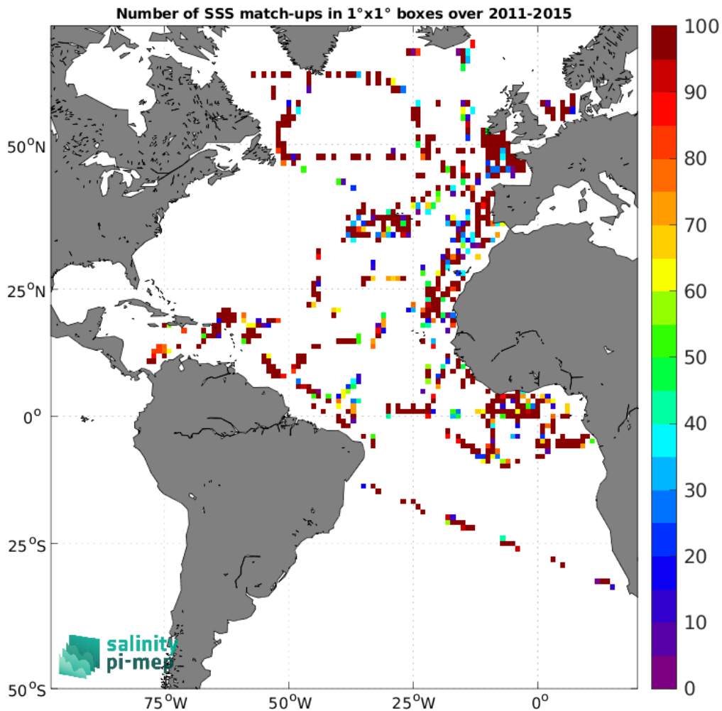
Figure 4: Number of SSS match-ups between TSG (GOSUD-Research-vessel) SSS and the Aquarius SSS L2 OR v5 (NASA-GSFC) SSS product for the Atlantic Ocean Pi-MEP region over 1^{\circ} \times 1^{\circ} boxes and for the full satellite product period.
