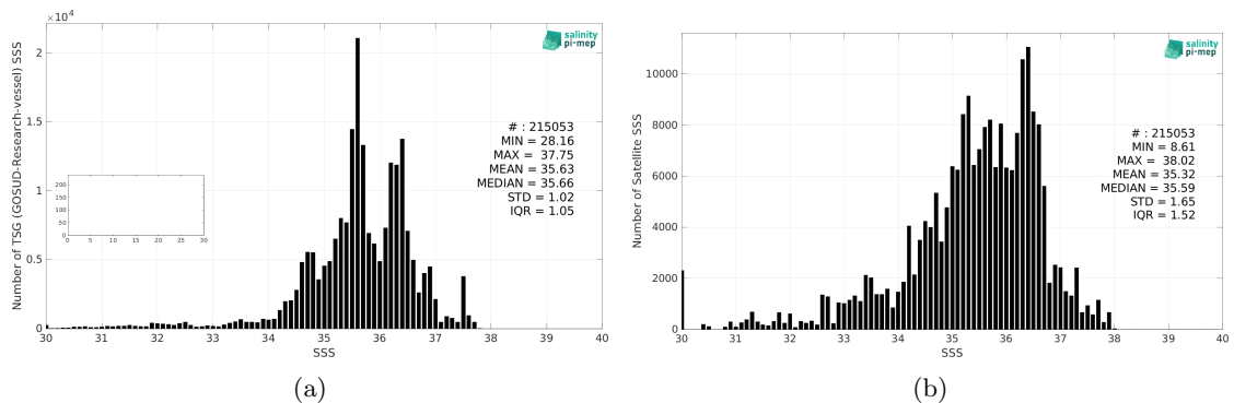
Figure 2: Histograms of SSS from TSG (GOSUD-Research-vessel) (a) and Aquarius SSS L2 OR v5 (NASA-GSFC) (b) considering all match-up pairs per bins of 0.1 over the Atlantic Ocean Pi-MEP region and for the full satellite product period.
