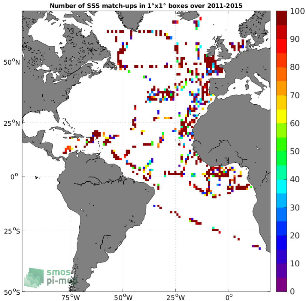
Figure 4: Number of SSS match-ups between TSG (GOSUD-Research-vessel) SSS and the Aquarius SSS L2 OR v5 (NASA-GSFC) SSS product for the Atlantic Ocean Pi-MEP region over 1°x1° boxes and for the full satellite product period.
