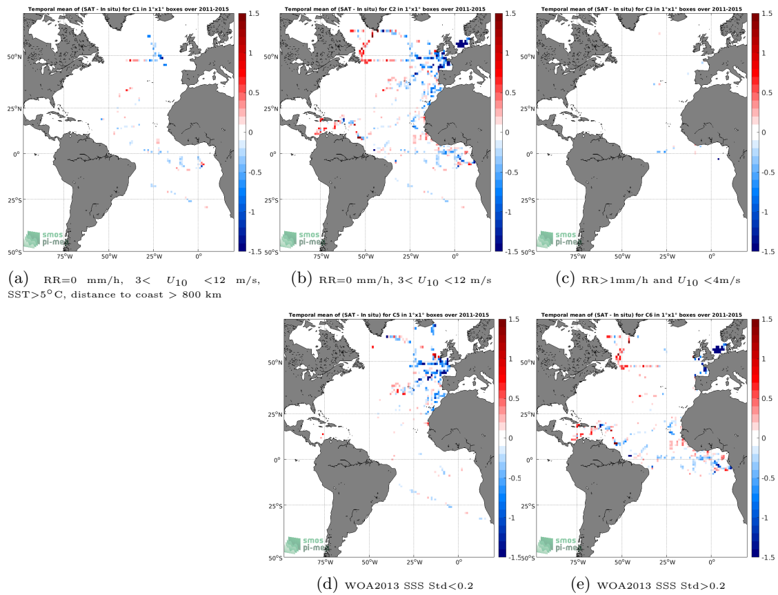
Figure 12: Temporal mean gridded over spatial boxes of size 1^\circ \times 1^\circ of \Delta SSS (Aquarius SSS L2 OR v5 (NASA-GSFC) - TSG (GOSUD-Research-vessel)) for 5 different subdatasets corresponding to:RR=0 mm/h, 3 < U_{10} < 12 m/s, SST>5°C, distance to coast > 800 km (a), RR=0 mm/h, 3 < U_{10} < 12 m/s (b), RR>1mm/h and U_{10} < 4 m/s (c), WOA2013 SSS Std<0.2 (d), WOA2013 SSS Std>0.2 (e).
