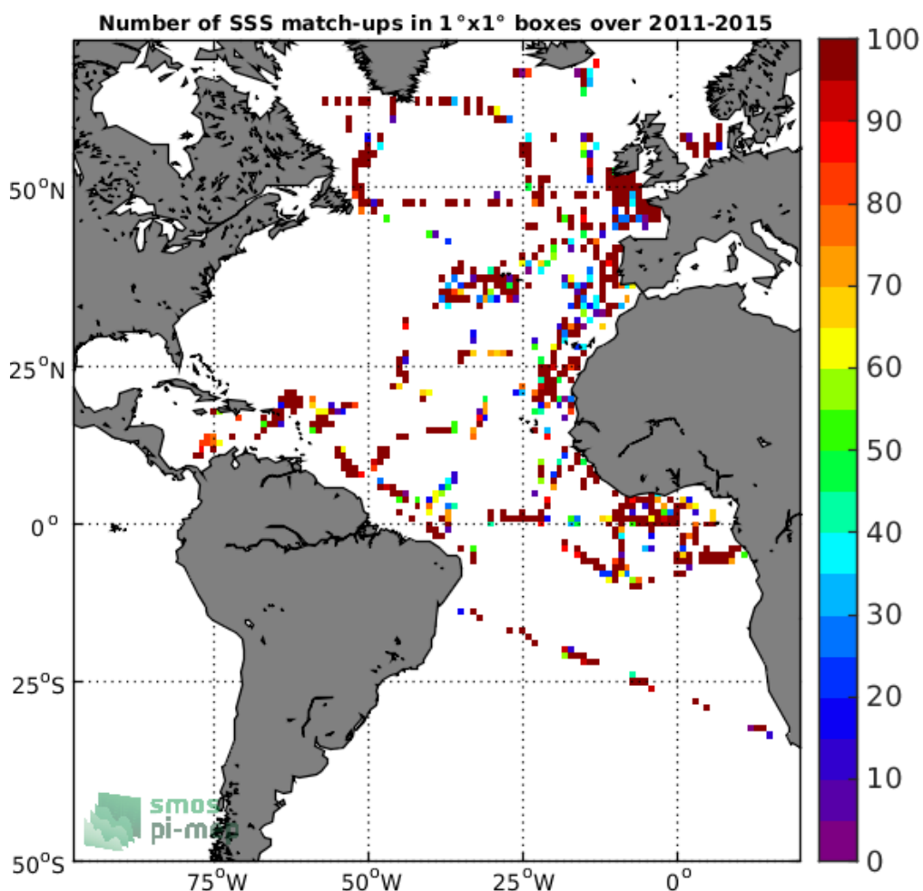
Figure 4: Number of SSS match-ups between TSG-GOSUD-Research-vessel SSS and the Aquarius-L2-OR-V5 SSS product for the Atlantic Ocean Pi-MEP region over 1°x1° boxes and for the full satellite product period.
