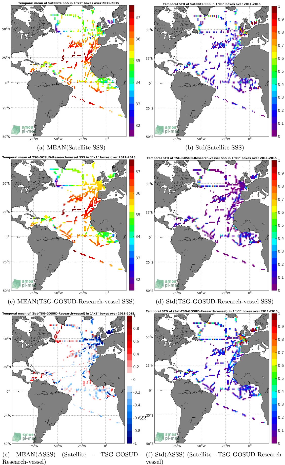
Figure 6: Temporal mean (left) and Std (right) of SSS from Aquarius-L2-OR-V5 (top), TSG-GOSUD-Research-vessel (middle), and of \Delta SSS (Satellite - TSG-GOSUD-Research-vessel). Only match-up pairs are used to generate these maps.
