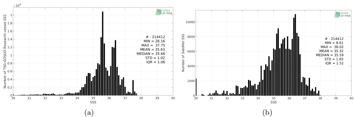
Figure 2: Histograms of SSS from TSG-GOSUD-Research-vessel (a) and Aquarius-L2-OR-V5 (b) considering all match-up pairs per bins of 0.1 over the Atlantic Ocean Pi-MEP region and for the full satellite product period.
