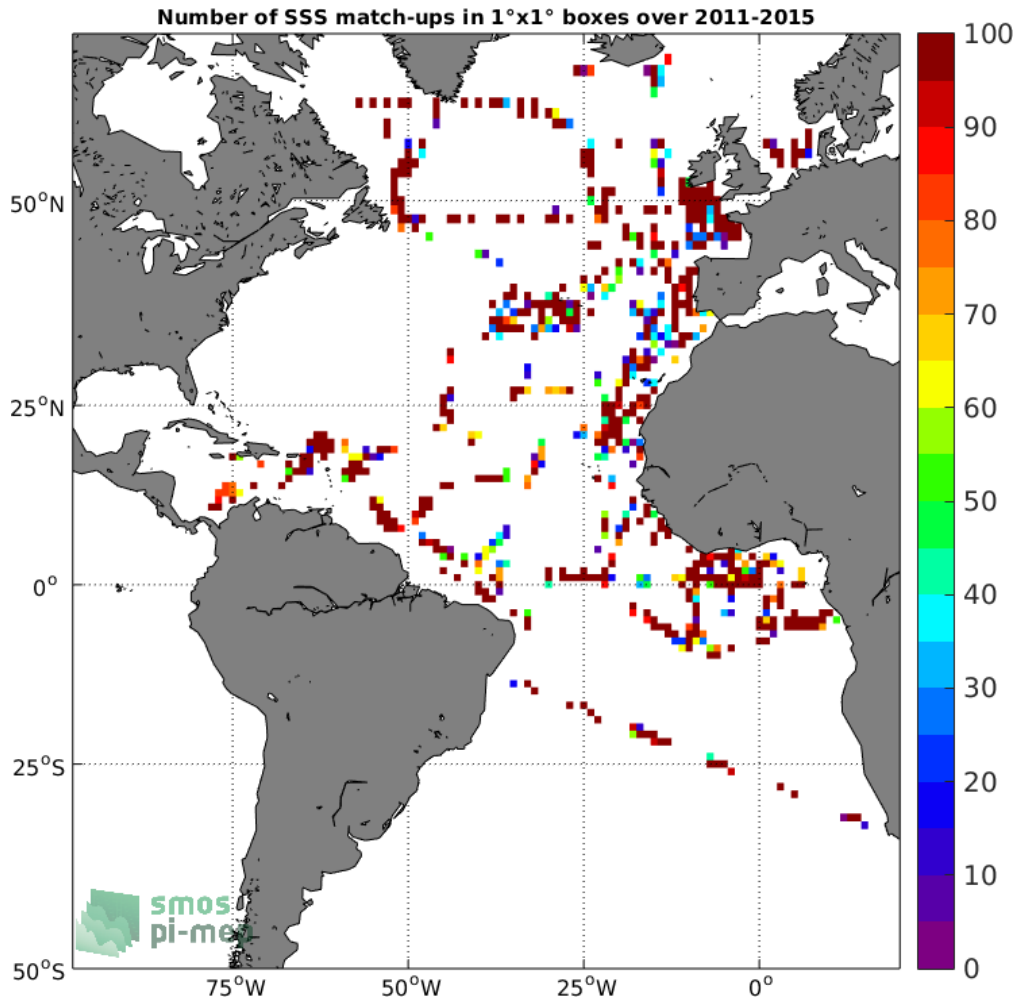
Figure 4: Number of SSS match-ups between TSG-GOSUD-Research-vessel SSS and the Aquarius-L2-OR-V5 SSS product for the Atlantic Ocean Pi-MEP region over 1°x1° boxes and for the full satellite product period.
