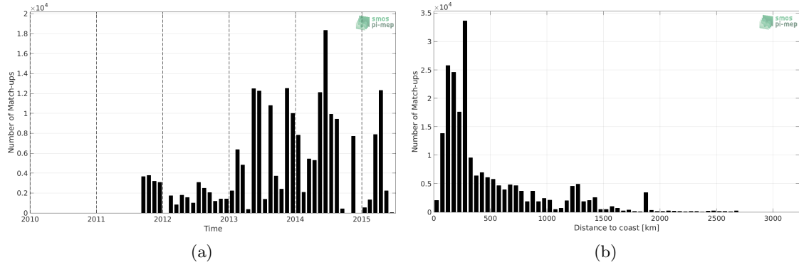
Figure 1: Number of match-ups between TSG-GOSUD-Research-vessel and Aquarius-L2-OR-V5 SSS as a function of time (a) and as function of the distance to coast (b) over the Atlantic Ocean Pi-MEP region and for the full satellite product period.
