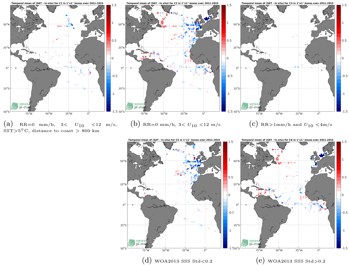
Figure 12: Temporal mean gridded over spatial boxes of size 1^\circ \times 1^\circ of \Delta SSS (Aquarius-L2-OR-V5 - TSG-GOSUD-Research-vessel) for 5 different subdatasets corresponding to:RR=0 mm/h, 3 < U_{10} < 12 m/s, SST >5^\circ C, distance to coast > 800 km (a), RR=0 mm/h, 3 < U_{10} < 12 m/s (b), RR >1 mm/h and U_{10} < 4 m/s (c), WOA2013 SSS Std <0.2 (d), WOA2013 SSS Std >0.2 (e).
