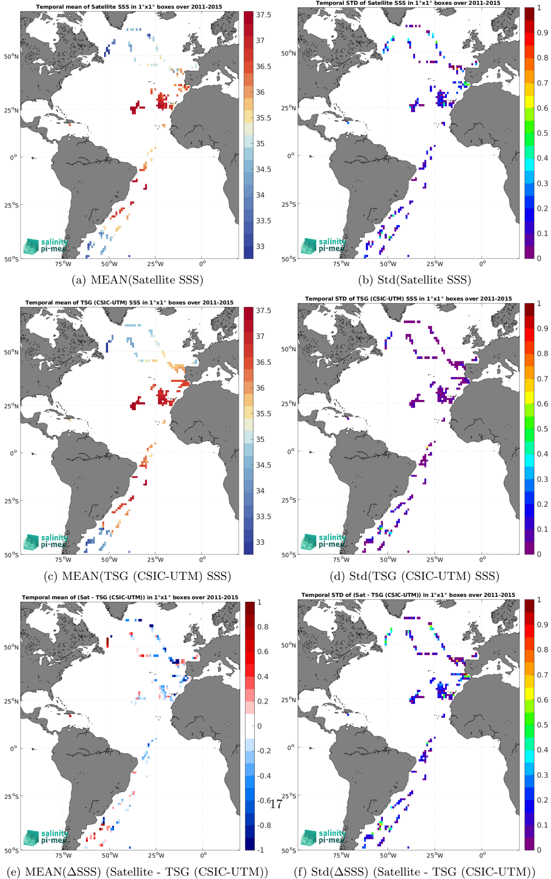
Figure 7: Temporal mean (left) and Std (right) of SSS from Aquarius SSS L2 OR v5 (NASA-GSFC) (top), TSG (CSIC-UTM) (middle), and of \Delta SSS (Satellite - TSG (CSIC-UTM)). Only match-up pairs are used to generate these maps.
