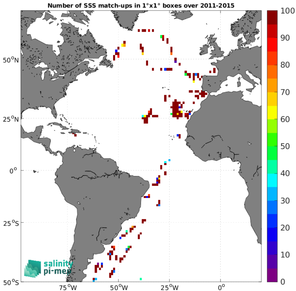
Figure 5: Number of SSS match-ups between TSG (CSIC-UTM) SSS and the Aquarius SSS L2 OR v5 (NASA-GSFC) SSS product for the Atlantic Ocean Pi-MEP region over 1°×1° boxes and for the full satellite product period.
