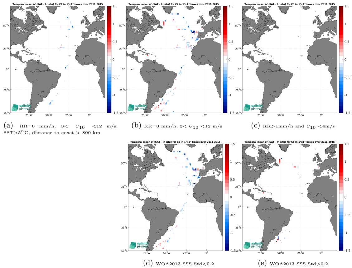
Figure 14: Temporal mean gridded over spatial boxes of size 1^\circ \times 1^\circ of \Delta SSS (Aquarius SSS L2 OR v5 (NASA-GSFC) - TSG (CSIC-UTM)) for 5 different subdatasets corresponding to:RR=0 mm/h, 3 < U_{10} < 12 m/s, SST>5°C, distance to coast > 800 km (a), RR=0 mm/h, 3 < U_{10} < 12 m/s (b), RR>1mm/h and U_{10} < 4 m/s (c), WOA2013 SSS Std<0.2 (d), WOA2013 SSS Std>0.2 (e).
