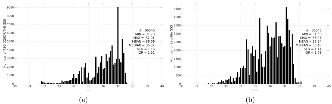
Figure 3: Histograms of SSS from TSG (CSIC-UTM) (a) and Aquarius SSS L2 OR v5 (NASA-GSFC) (b) considering all match-up pairs per bins of 0.1 over the Atlantic Ocean Pi-MEP region and for the full satellite product period.
