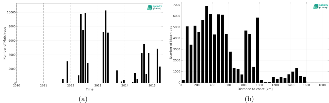
Figure 2: Number of match-ups between TSG (CSIC-UTM) and Aquarius SSS L2 OR v5 (NASA-GSFC) SSS as a function of time (a) and as function of the distance to coast (b) over the Atlantic Ocean Pi-MEP region and for the full satellite product period.
