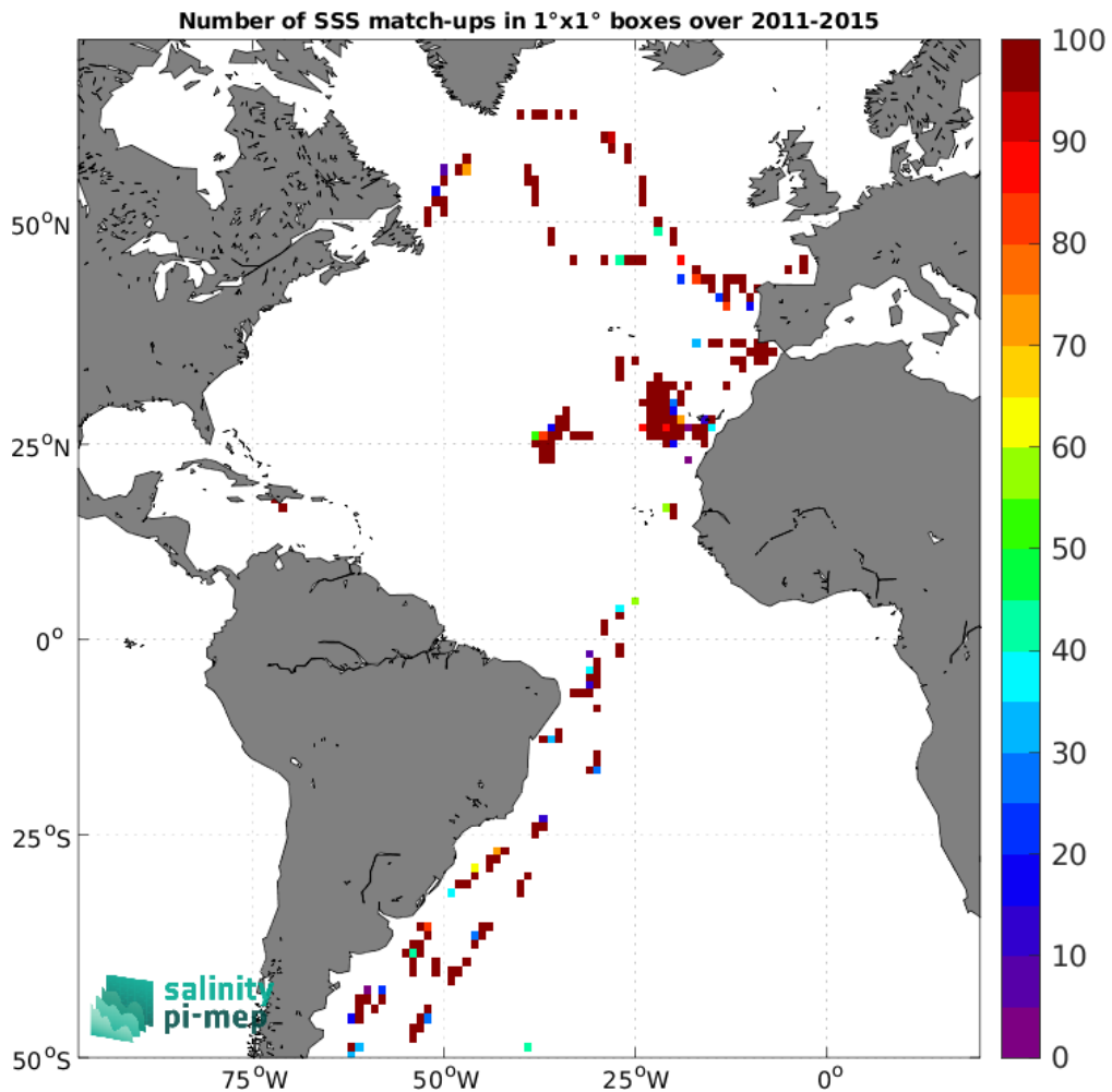
Figure 4: Number of SSS match-ups between TSG (CSIC-UTM) SSS and the Aquarius SSS L2 OR v5 (NASA-GSFC) SSS product for the Atlantic Ocean Pi-MEP region over 1^{\circ} \times 1^{\circ} boxes and for the full satellite product period.
