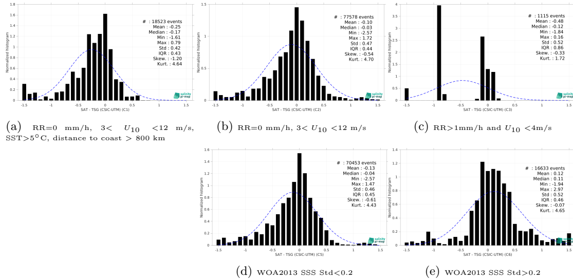
Figure 13: Normalized histogram of \Delta SSS (Aquarius SSS L2 OR v5 (NASA-GSFC) - TSG (CSIC-UTM)) for 5 different subdatasets corresponding to: RR=0 mm/h, 3 < U_{10} < 12 m/s, SST>5°C, distance to coast > 800 km (a), RR=0 mm/h, 3 < U_{10} < 12 m/s (b), RR>1mm/h and U_{10} < 4 m/s (c), WOA2013 SSS Std<0.2 (d), WOA2013 SSS Std>0.2 (e).
