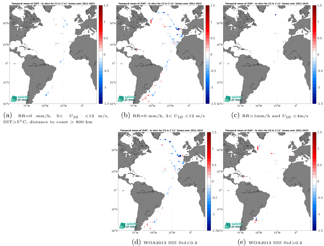
Figure 12: Temporal mean gridded over spatial boxes of size 1^\circ \times 1^\circ of \Delta SSS (Aquarius SSS L2 OR v5 (NASA-GSFC) - TSG (CSIC-UTM)) for 5 different subdatasets corresponding to:RR=0 mm/h, 3 < U_{10} < 12 m/s, SST >5^\circ\text{C} , distance to coast > 800 km (a), RR=0 mm/h, 3 < U_{10} < 12 m/s (b), RR >1 mm/h and U_{10} < 4 m/s (c), WOA2013 SSS Std <0.2 (d), WOA2013 SSS Std >0.2 (e).
