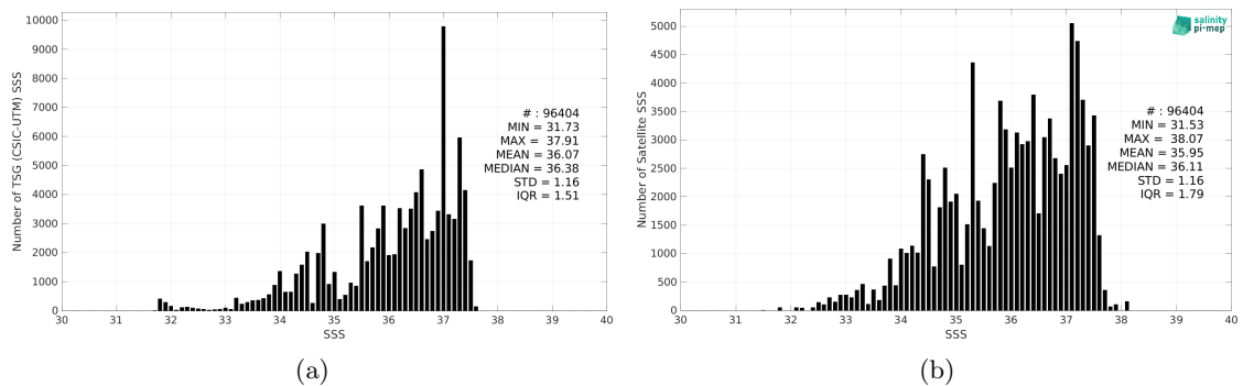
Figure 2: Histograms of SSS from TSG (CSIC-UTM) (a) and Aquarius SSS L2 OR v5 (NASA-GSFC) (b) considering all match-up pairs per bins of 0.1 over the Atlantic Ocean Pi-MEP region and for the full satellite product period.
