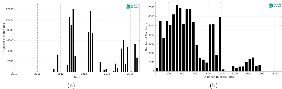
Figure 1: Number of match-ups between TSG (CSIC-UTM) and Aquarius SSS L2 OR v5 (NASA-GSFC) SSS as a function of time (a) and as function of the distance to coast (b) over the Atlantic Ocean Pi-MEP region and for the full satellite product period.
