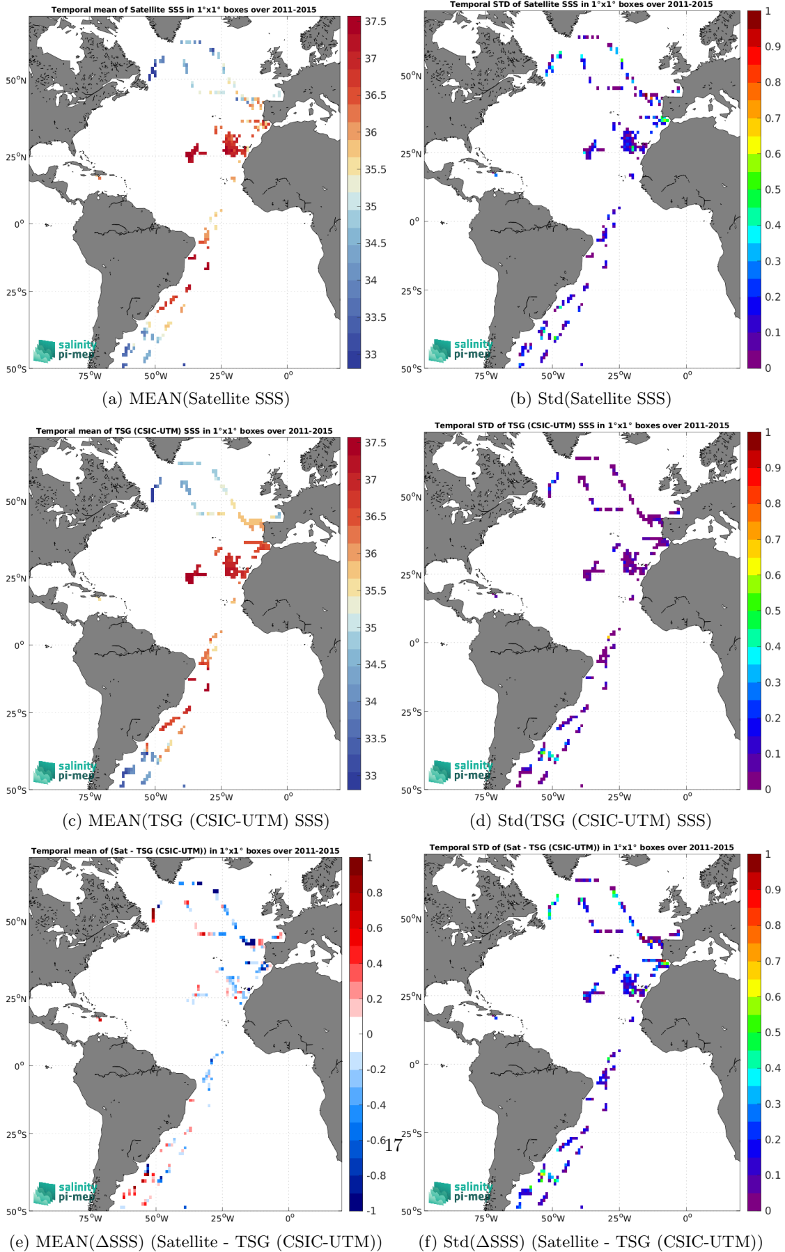
Figure 6: Temporal mean (left) and Std (right) of SSS from Aquarius SSS L2 OR v5 (NASA-GSFC) (top), TSG (CSIC-UTM) (middle), and of \Delta SSS (Satellite - TSG (CSIC-UTM)). Only match-up pairs are used to generate these maps.
