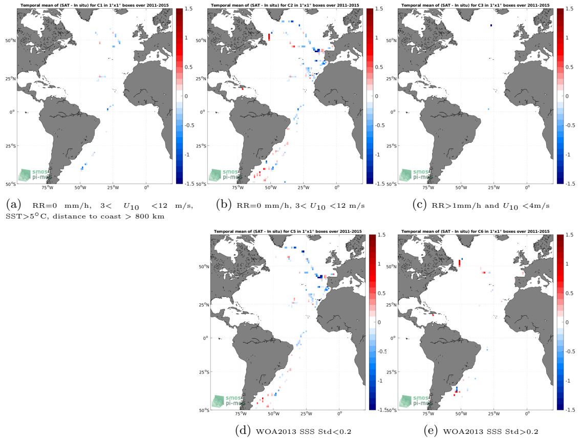
Figure 12: Temporal mean gridded over spatial boxes of size 1^\circ \times 1^\circ of \Delta SSS (Aquarius SSS L2 OR v5 (NASA-GSFC) - TSG (CSIC-UTM)) for 5 different subdatasets corresponding to:RR=0 mm/h, 3 < U_{10} < 12 m/s, SST >5^\circ\text{C} , distance to coast > 800 km (a), RR=0 mm/h, 3 < U_{10} < 12 m/s (b), RR >1 mm/h and U_{10} < 4 m/s (c), WOA2013 SSS Std <0.2 (d), WOA2013 SSS Std >0.2 (e).
