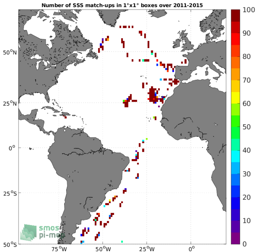
Figure 4: Number of SSS match-ups between TSG (CSIC-UTM) SSS and the Aquarius SSS L2 OR v5 (NASA-GSFC) SSS product for the Atlantic Ocean Pi-MEP region over 1°x1° boxes and for the full satellite product period.
