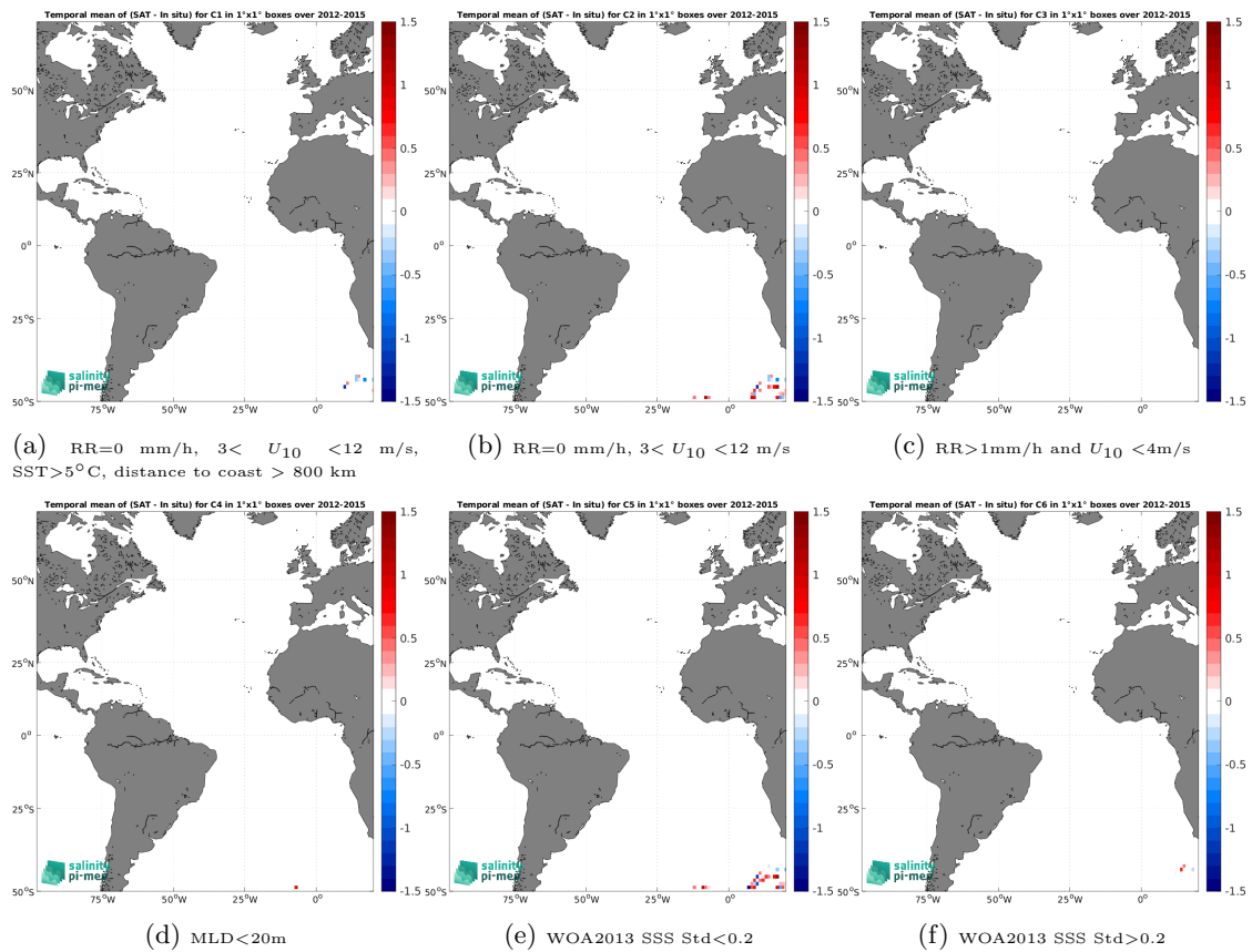
Figure 12: Temporal mean gridded over spatial boxes of size 1^{\circ} \times 1^{\circ} of \Delta SSS (Aquarius SSS L2 OR v5 (NASA-GSFC) - Marine mammals) for 6 different subdatasets corresponding to: RR=0 mm/h, 3 < U_{10} < 12 m/s, SST > 5^{\circ}C , distance to coast > 800 km (a), RR=0 mm/h, 3 < U_{10} < 12 m/s (b), RR > 1 mm/h and U_{10} < 4 m/s (c), MLD < 20 m (d), WOA2013 SSS Std < 0.2 (e), WOA2013 SSS Std > 0.2 (f).
