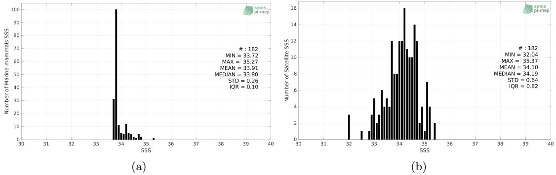
Figure 2: Histograms of SSS from Marine mammals (a) and Aquarius SSS L2 OR v5 (NASA-GSFC) (b) considering all match-up pairs per bins of 0.1 over the Atlantic Ocean Pi-MEP region and for the full satellite product period.
