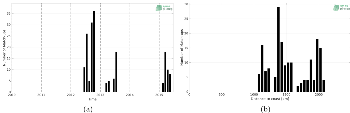
Figure 1: Number of match-ups between Marine mammals and Aquarius SSS L2 OR v5 (NASA-GSFC) SSS as a function of time (a) and as function of the distance to coast (b) over the Atlantic Ocean Pi-MEP region and for the full satellite product period.
