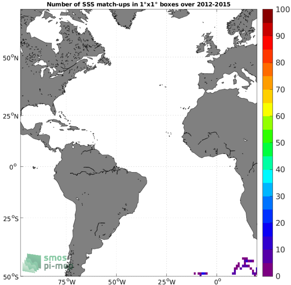
Figure 4: Number of SSS match-ups between Marine mammals SSS and the Aquarius SSS L2 OR v5 (NASA-GSFC) SSS product for the Atlantic Ocean Pi-MEP region over 1^\circ \times 1^\circ boxes and for the full satellite product period.
