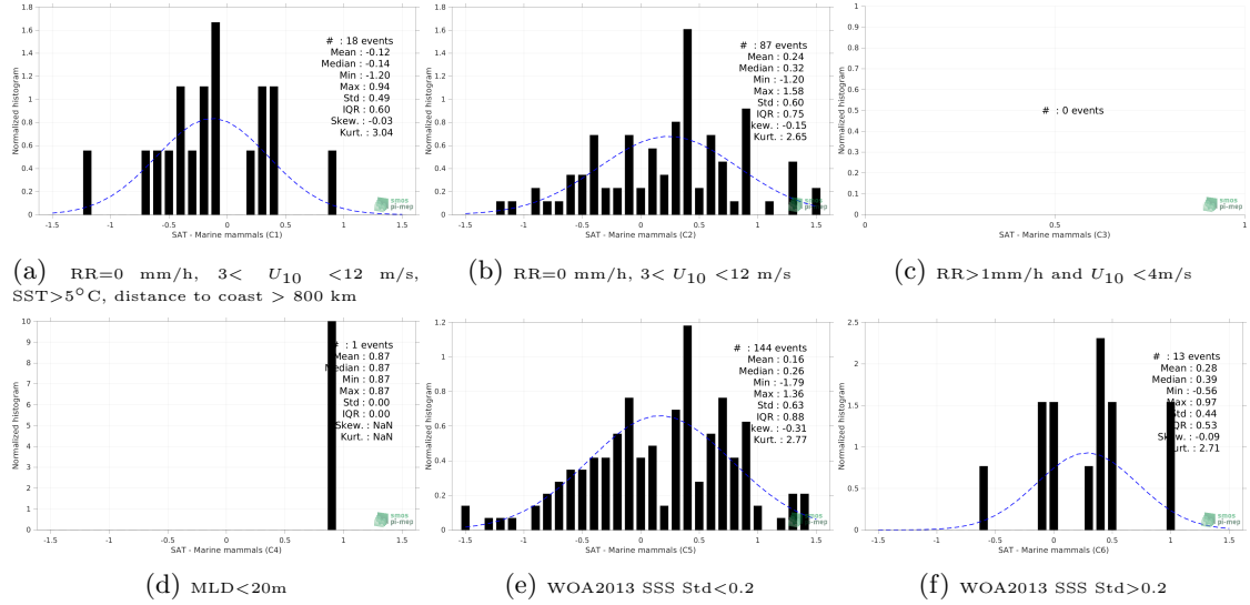
Figure 13: Normalized histogram of \Delta SSS (Aquarius SSS L2 OR v5 (NASA-GSFC) - Marine mammals) for 6 different subdatasets corresponding to: RR=0 mm/h, 3 < U_{10} < 12 m/s, SST>5°C, distance to coast > 800 km (a), RR=0 mm/h, 3 < U_{10} < 12 m/s (b), RR>1mm/h and U_{10} < 4 m/s (c), MLD<20m (d), WOA2013 SSS Std<0.2 (e), WOA2013 SSS Std>0.2 (f).
