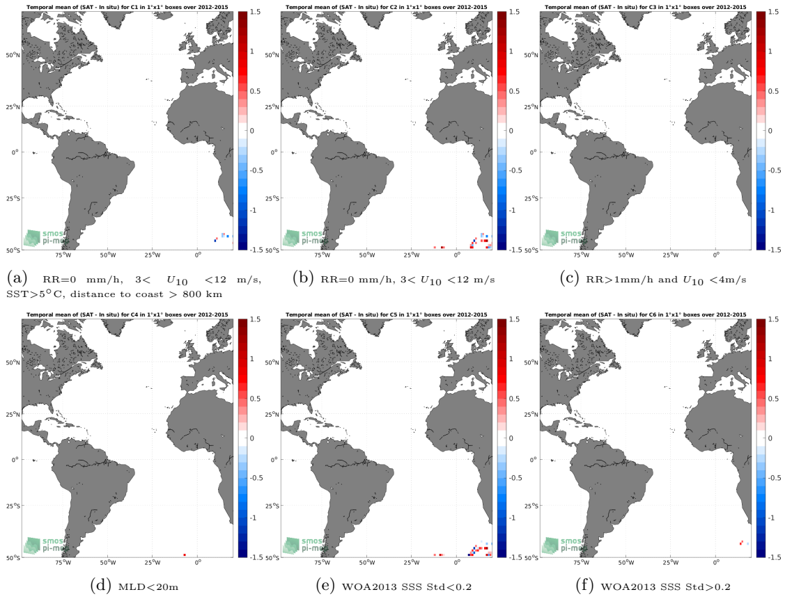
Figure 12: Temporal mean gridded over spatial boxes of size 1^\circ \times 1^\circ of \Delta SSS (Aquarius SSS L2 OR v5 (NASA-GSFC) - Marine mammals) for 6 different subdatasets corresponding to:RR=0 mm/h, 3 < U_{10} < 12 m/s, SST>5°C, distance to coast > 800 km (a), RR=0 mm/h, 3 < U_{10} < 12 m/s (b), RR>1mm/h and U_{10} < 4 m/s (c),MLD<20m (d),WOA2013 SSS Std<0.2 (e),WOA2013 SSS Std>0.2 (f).
