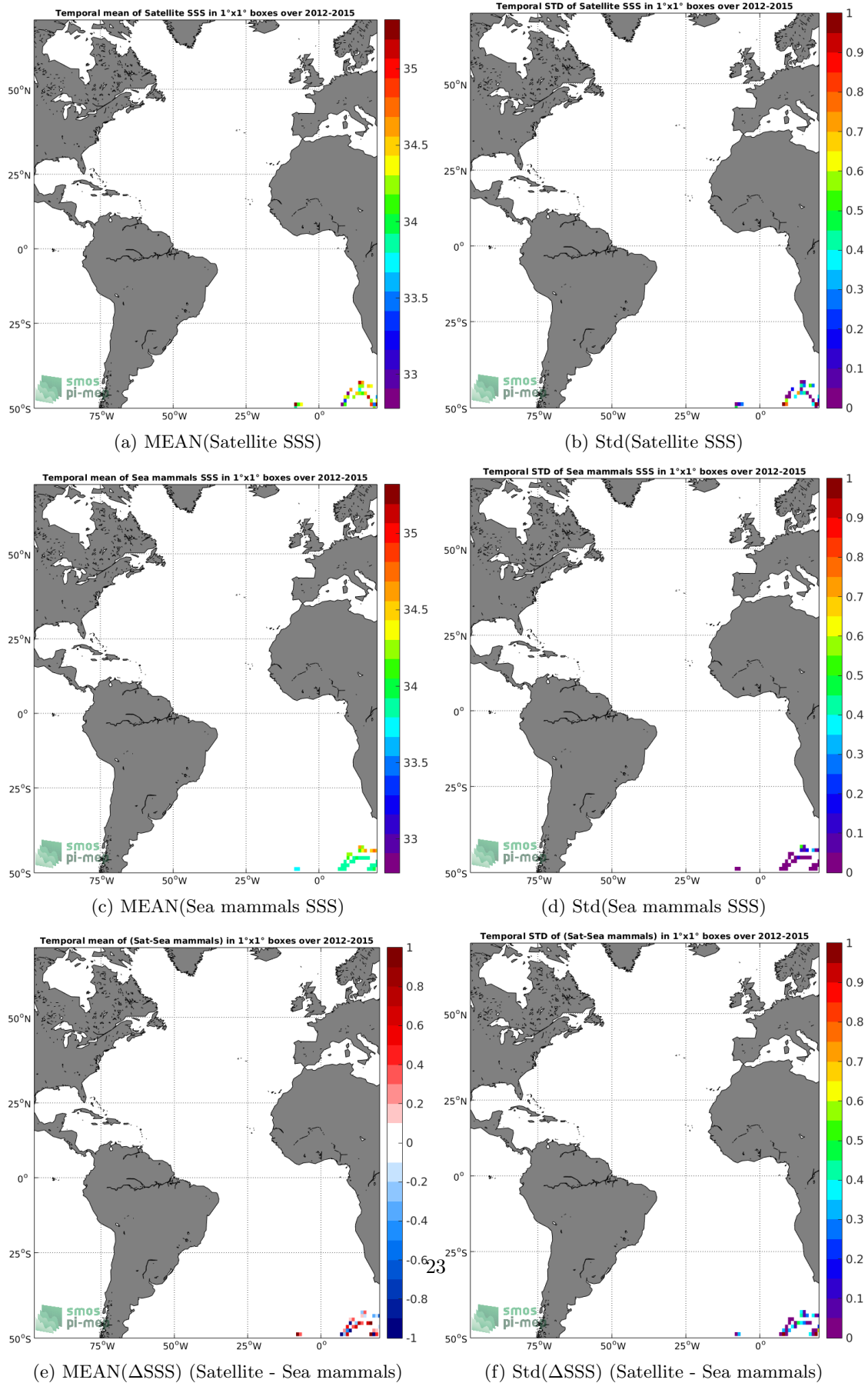
Figure 6: Temporal mean (left) and Std (right) of SSS from Aquarius-L2-OR-V5 (top), Sea mammals (middle), and of \Delta SSS (Satellite - Sea mammals). Only match-up pairs are used to generate these maps.
