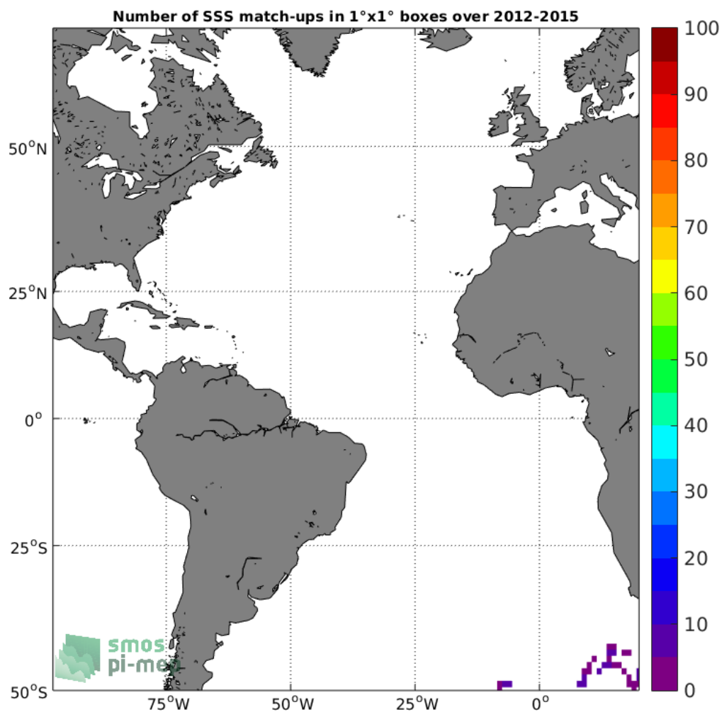
Figure 4: Number of SSS match-ups between Sea mammals SSS and the Aquarius-L2-OR-V5 SSS product for the Atlantic Ocean Pi-MEP region over 1°x1° boxes and for the full satellite product period.
