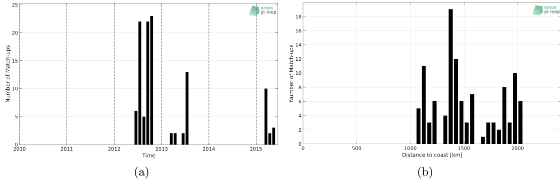
Figure 1: Number of match-ups between Sea mammals and Aquarius-L2-OR-V5 SSS as a function of time (a) and as function of the distance to coast (b) over the Atlantic Ocean Pi-MEP region and for the full satellite product period.
