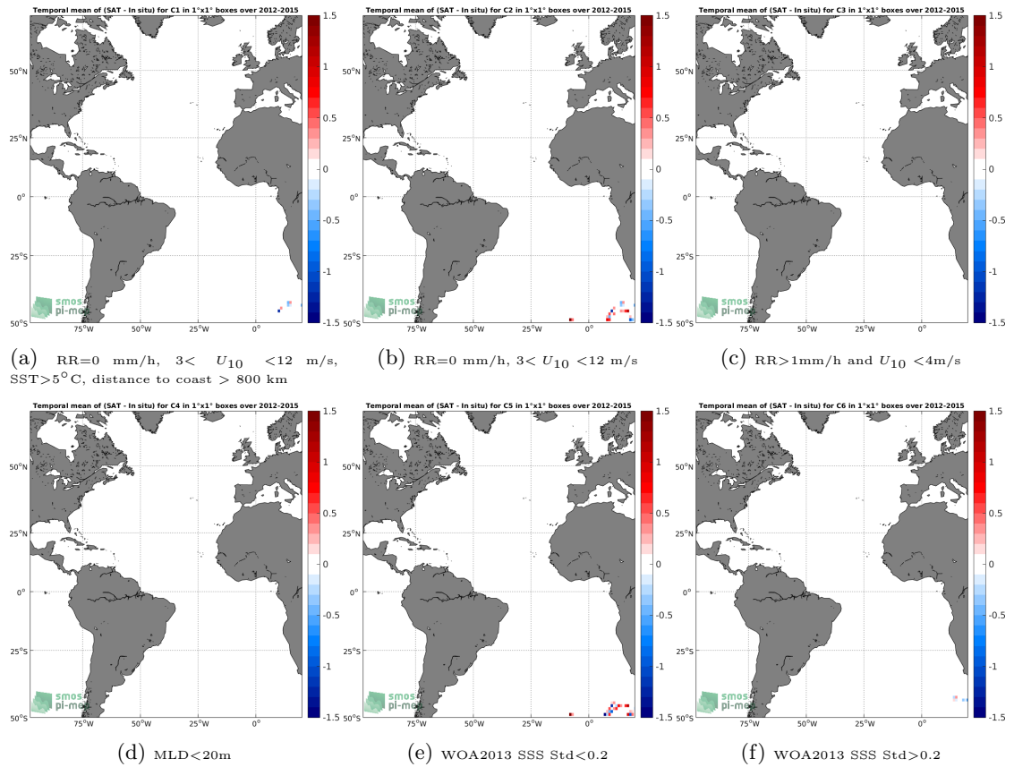
Figure 12: Temporal mean gridded over spatial boxes of size 1^\circ \times 1^\circ of \Delta SSS (Aquarius-L2-OR-V5 - Sea mammals) for 6 different subdatasets corresponding to:RR=0 mm/h, 3 < U_{10} < 12 m/s, SST >5^\circ C, distance to coast > 800 km (a), RR=0 mm/h, 3 < U_{10} < 12 m/s (b), RR >1 mm/h and U_{10} < 4 m/s (c),MLD <20 m (d),WOA2013 SSS Std <0.2 (e),WOA2013 SSS Std >0.2 (f).
