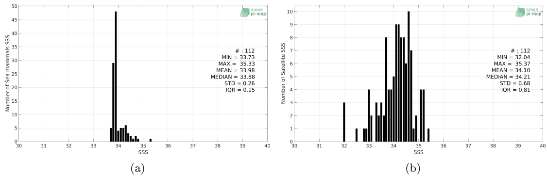
Figure 2: Histograms of SSS from Sea mammals (a) and Aquarius-L2-OR-V5 (b) considering all match-up pairs per bins of 0.1 over the Atlantic Ocean Pi-MEP region and for the full satellite product period.
