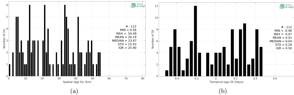
Figure 5: Histograms of the spatial (a) and temporal (b) lags between the time of the Sea mammals measurements and the date of the corresponding Aquarius-L2-OR-V5 SSS product.
