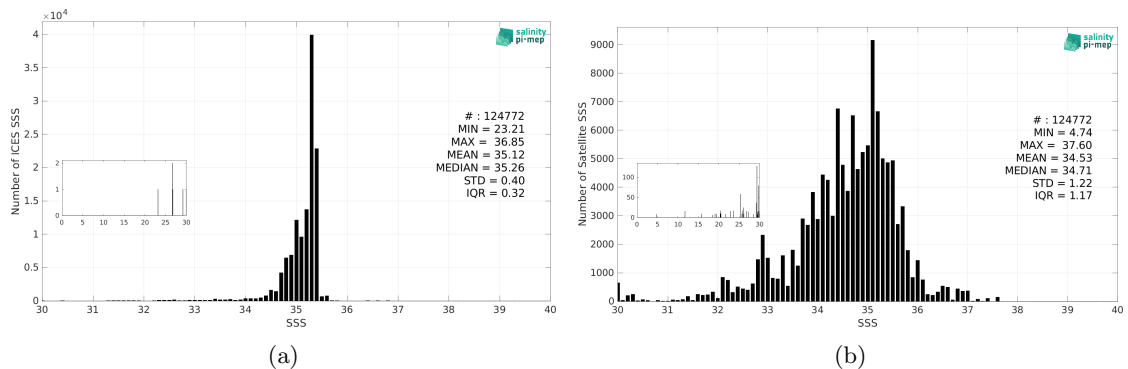
Figure 3: Histograms of SSS from ICES (a) and Aquarius SSS L2 OR v5 (NASA-GSFC) (b) considering all match-up pairs per bins of 0.1 over the Atlantic Ocean Pi-MEP region and for the full satellite product period.
