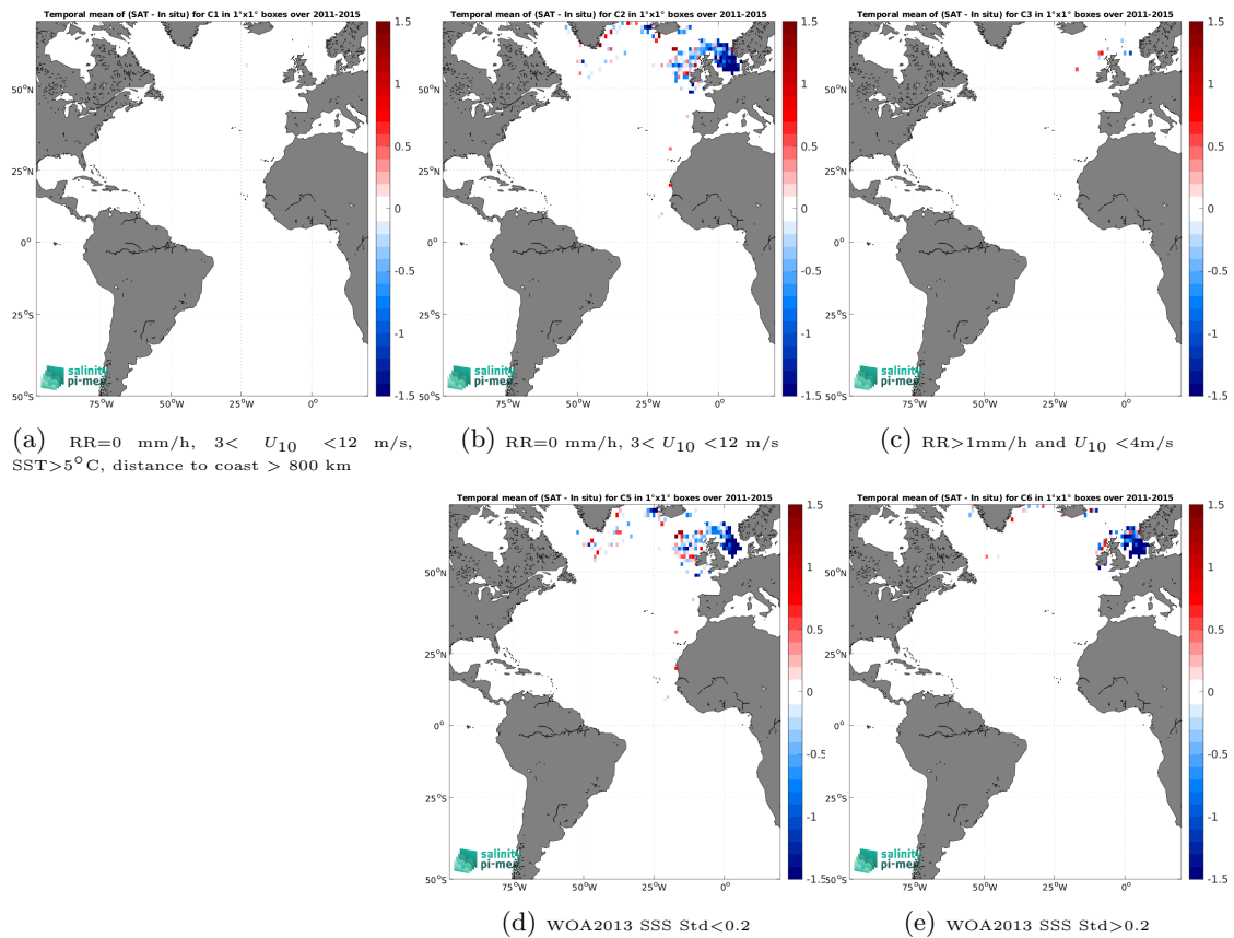
Figure 14: Temporal mean gridded over spatial boxes of size 1^\circ \times 1^\circ of \Delta\text{SSS} (Aquarius SSS L2 OR v5 (NASA-GSFC) - ICES) for 5 different subdatasets corresponding to:RR=0 mm/h, 3 < U_{10} < 12 m/s, SST >5^\circ\text{C} , distance to coast > 800 km (a), RR=0 mm/h, 3 < U_{10} < 12 m/s (b), RR >1 mm/h and U_{10} < 4 m/s (c), WOA2013 SSS Std <0.2 (d), WOA2013 SSS Std >0.2 (e).
