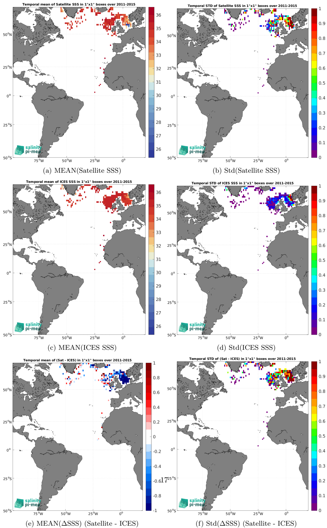
Figure 7: Temporal mean (left) and Std (right) of SSS from Aquarius SSS L2 OR v5 (NASA-GSFC) (top), ICES (middle), and of \Delta SSS (Satellite - ICES). Only match-up pairs are used to generate these maps.
