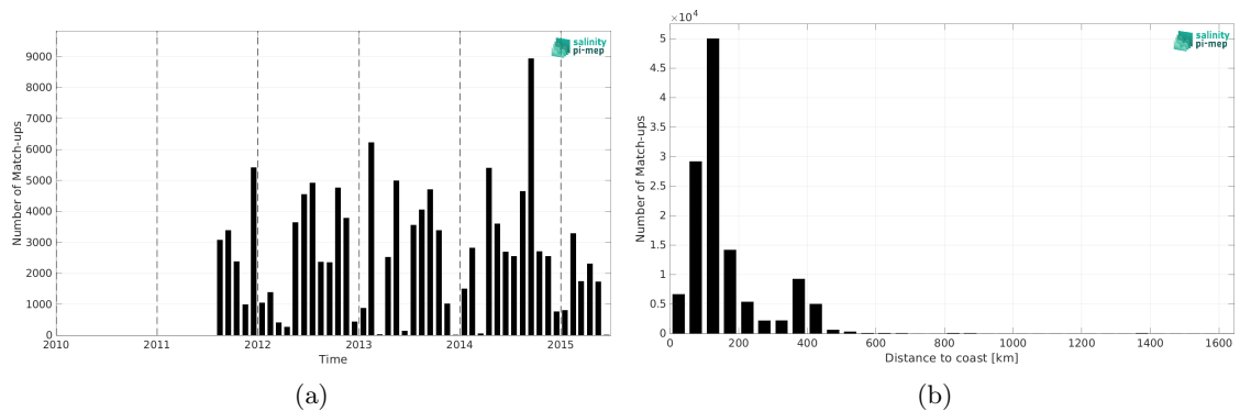
Figure 2: Number of match-ups between ICES and Aquarius SSS L2 OR v5 (NASA-GSFC) SSS as a function of time (a) and as function of the distance to coast (b) over the Atlantic Ocean Pi-MEP region and for the full satellite product period.
