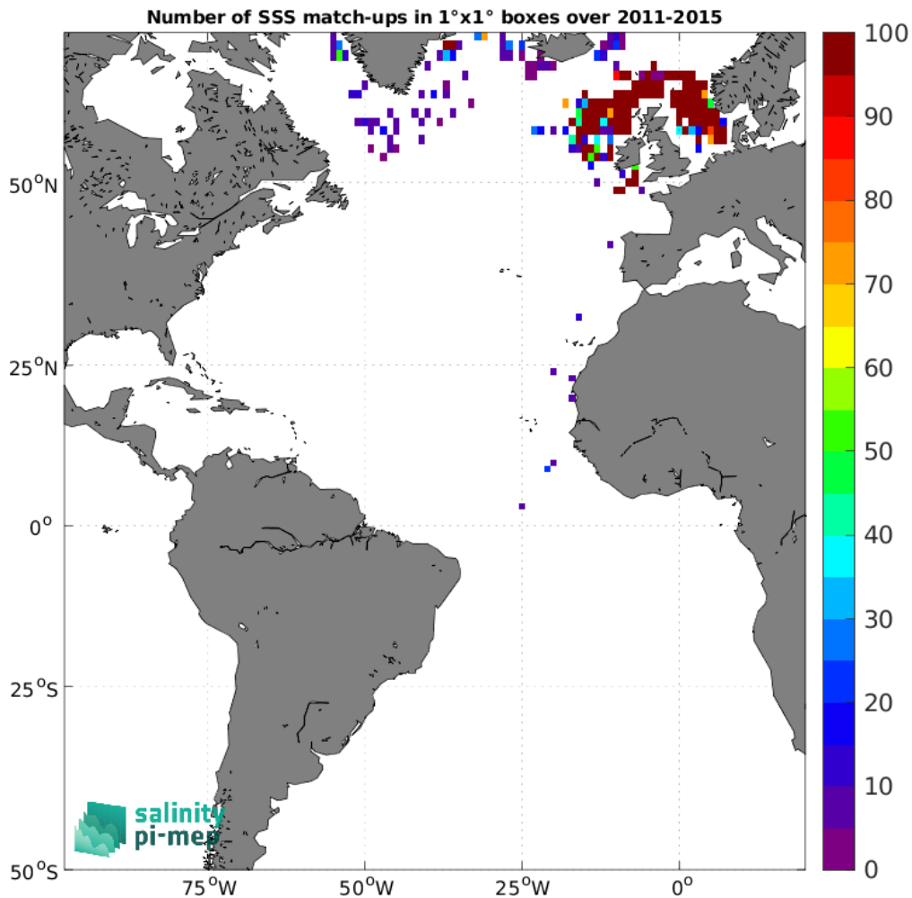
Figure 5: Number of SSS match-ups between ICES SSS and the Aquarius SSS L2 OR v5 (NASA-GSFC) SSS product for the Atlantic Ocean Pi-MEP region over 1^\circ \times 1^\circ boxes and for the full satellite product period.
