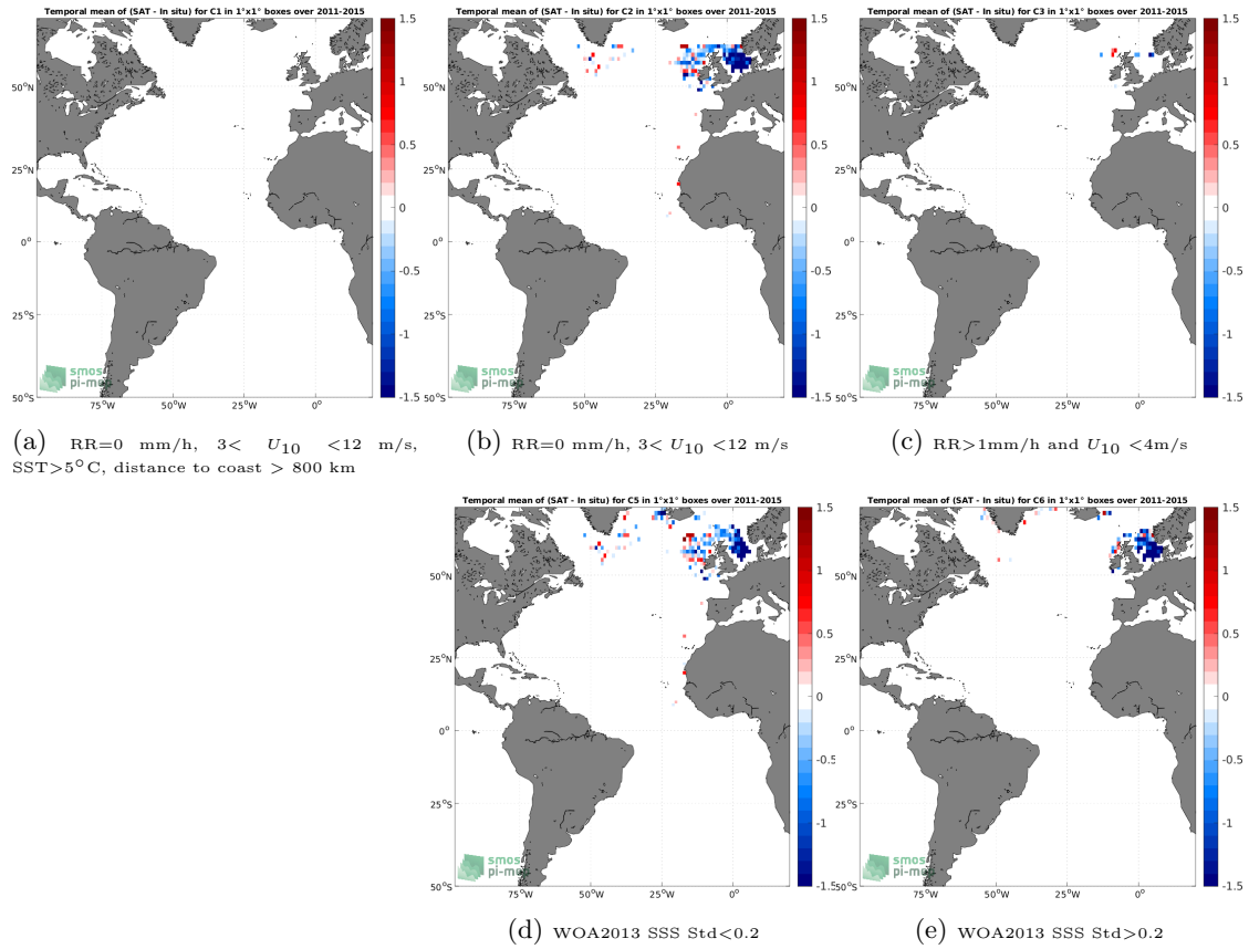
Figure 12: Temporal mean gridded over spatial boxes of size 1^\circ \times 1^\circ of \Delta SSS (Aquarius SSS L2 OR v5 (NASA-GSFC) - ICES) for 5 different subdatasets corresponding to:RR=0 mm/h, 3 < U_{10} < 12 m/s, SST >5^\circ\text{C} , distance to coast > 800 km (a), RR=0 mm/h, 3 < U_{10} < 12 m/s (b), RR >1 mm/h and U_{10} < 4 m/s (c), WOA2013 SSS Std <0.2 (d), WOA2013 SSS Std >0.2 (e).
