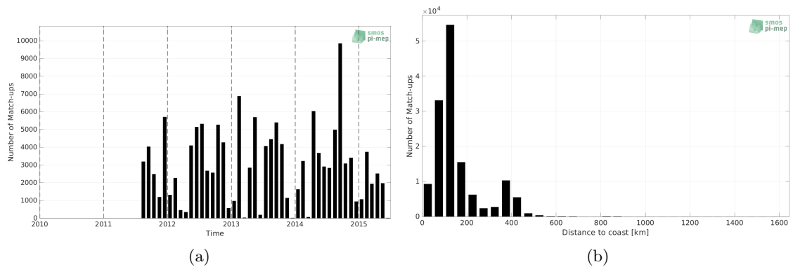
Figure 1: Number of match-ups between ICES and Aquarius SSS L2 OR v5 (NASA-GSFC) SSS as a function of time (a) and as function of the distance to coast (b) over the Atlantic Ocean Pi-MEP region and for the full satellite product period.
