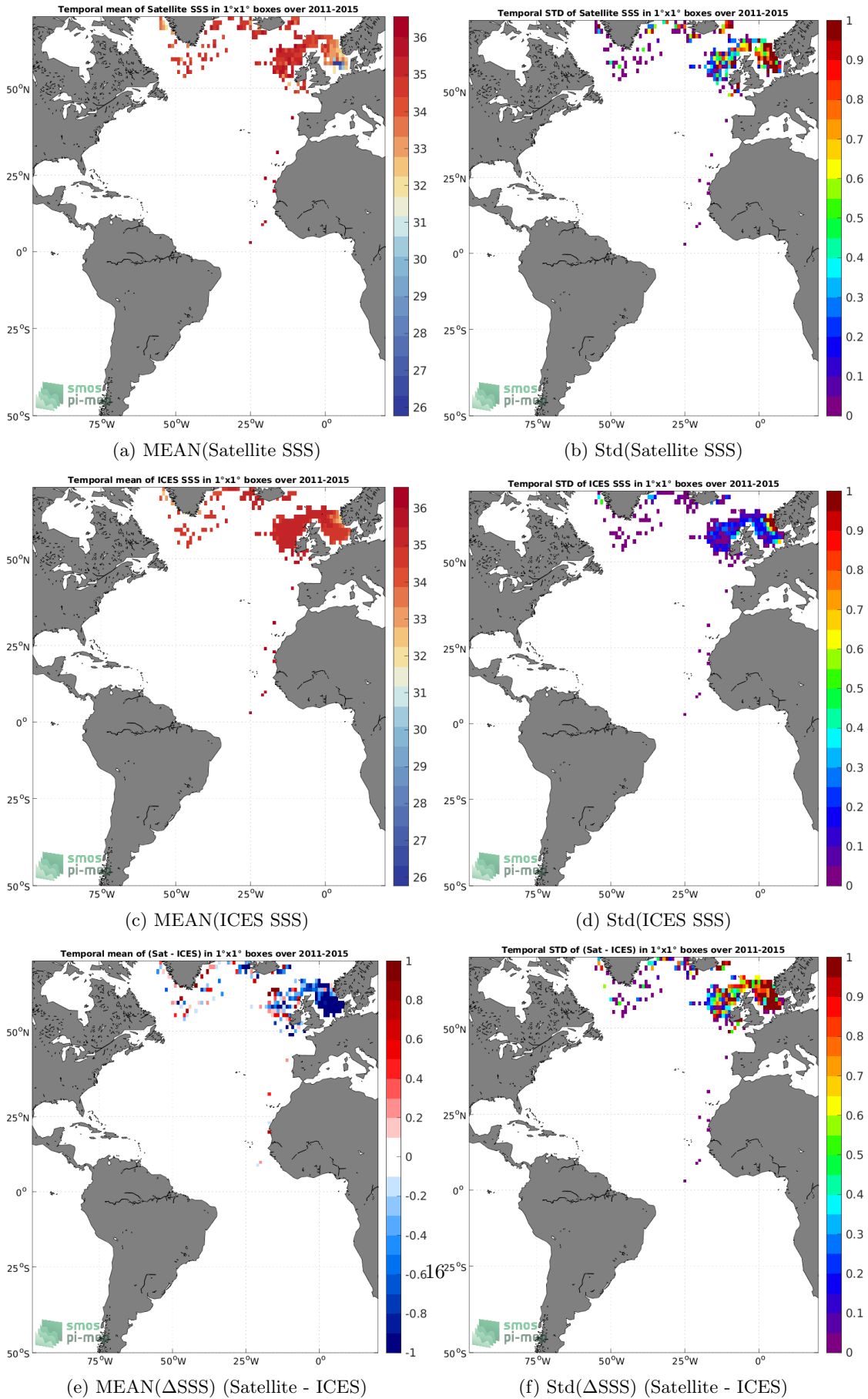
Figure 6: Temporal mean (left) and Std (right) of SSS from Aquarius SSS L2 OR v5 (NASA-GSFC) (top), ICES (middle), and of \Delta SSS (Satellite - ICES). Only match-up pairs are used to generate these maps.
