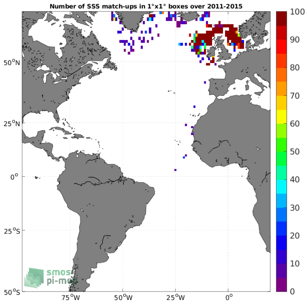
Figure 4: Number of SSS match-ups between ICES SSS and the Aquarius SSS L2 OR v5 (NASA-GSFC) SSS product for the Atlantic Ocean Pi-MEP region over 1°x1° boxes and for the full satellite product period.
