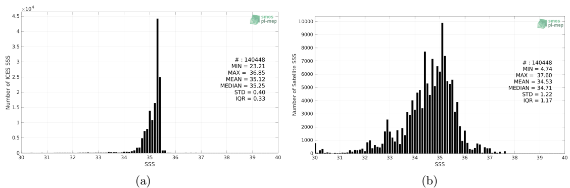
Figure 2: Histograms of SSS from ICES (a) and Aquarius SSS L2 OR v5 (NASA-GSFC) (b) considering all match-up pairs per bins of 0.1 over the Atlantic Ocean Pi-MEP region and for the full satellite product period.
