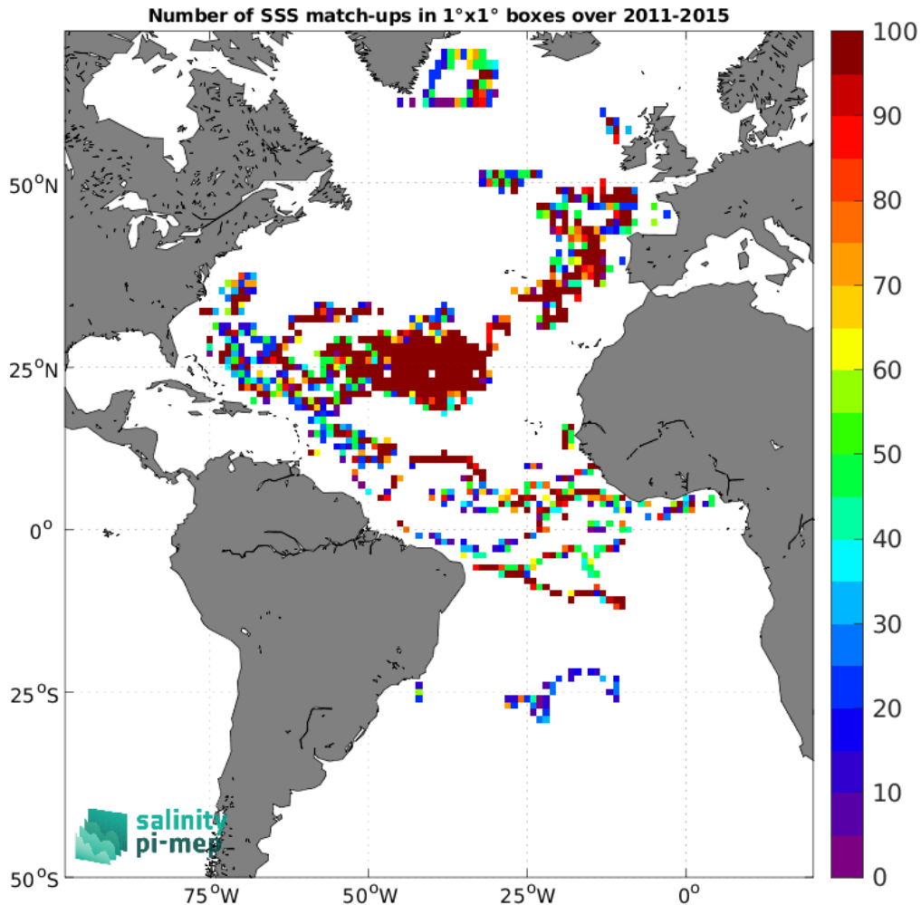
Figure 4: Number of SSS match-ups between Surface drifters SSS and the Aquarius SSS L2 OR v5 (NASA-GSFC) SSS product for the Atlantic Ocean Pi-MEP region over 1^\circ \times 1^\circ boxes and for the full satellite product period.
