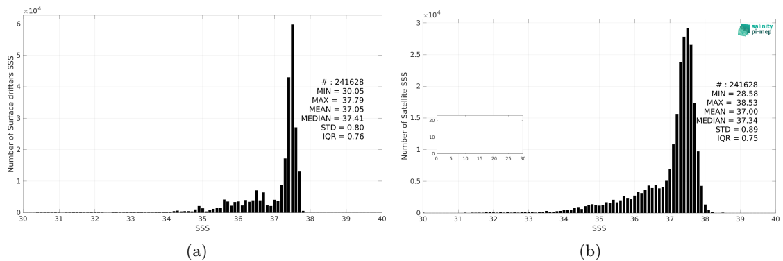
Figure 3: Histograms of SSS from Surface drifters (a) and Aquarius SSS L2 OR v5 (NASA-GSFC) (b) considering all match-up pairs per bins of 0.1 over the Atlantic Ocean Pi-MEP region and for the full satellite product period.
