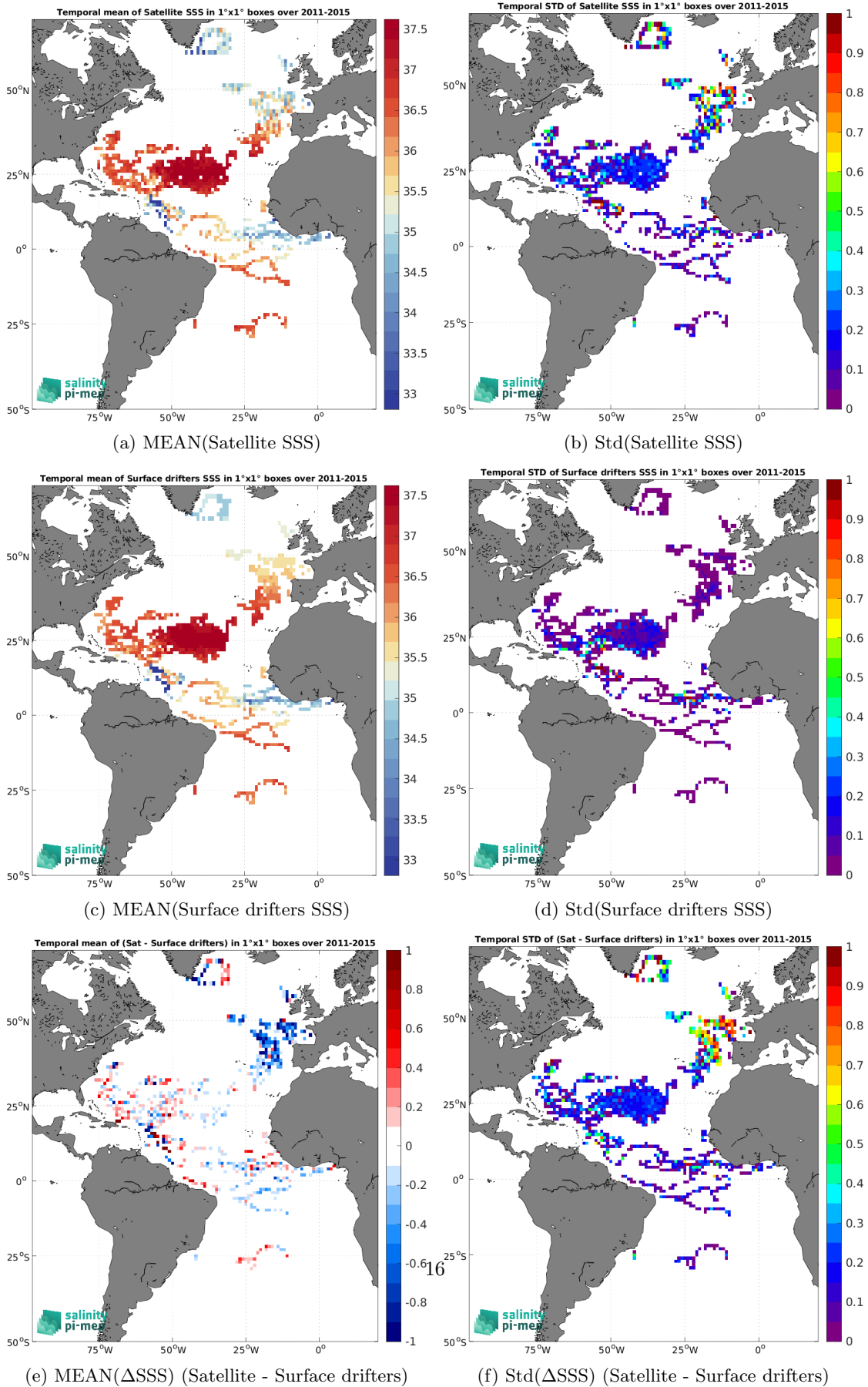
(e) MEAN( \Delta SSS) (Satellite - Surface drifters) (f) Std( \Delta SSS) (Satellite - Surface drifters) Figure 6: Temporal mean (left) and Std (right) of SSS from Aquarius SSS L2 OR v5 (NASA-GSFC) (top), Surface drifters (middle), and of \Delta SSS (Satellite - Surface drifters). Only match-up pairs are used to generate these maps.
