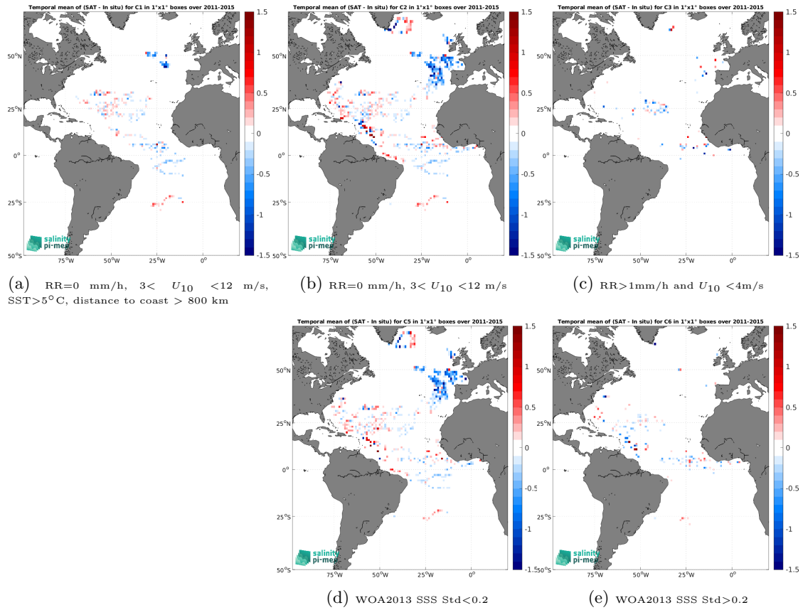
Figure 13: Temporal mean gridded over spatial boxes of size 1^\circ \times 1^\circ of \Delta\text{SSS} (Aquarius SSS L2 OR v5 (NASA-GSFC) - Surface drifters) for 5 different subdatasets corresponding to:RR=0 mm/h, 3 < U_{10} < 12 m/s, SST >5^\circ\text{C} , distance to coast > 800 km (a), RR=0 mm/h, 3 < U_{10} < 12 m/s (b), RR >1 mm/h and U_{10} < 4 m/s (c), WOA2013 SSS Std <0.2 (d), WOA2013 SSS Std >0.2 (e).
