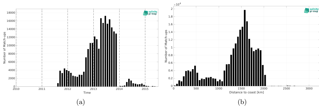
Figure 2: Number of match-ups between Surface drifters and Aquarius SSS L2 OR v5 (NASA-GSFC) SSS as a function of time (a) and as function of the distance to coast (b) over the Atlantic Ocean Pi-MEP region and for the full satellite product period.
