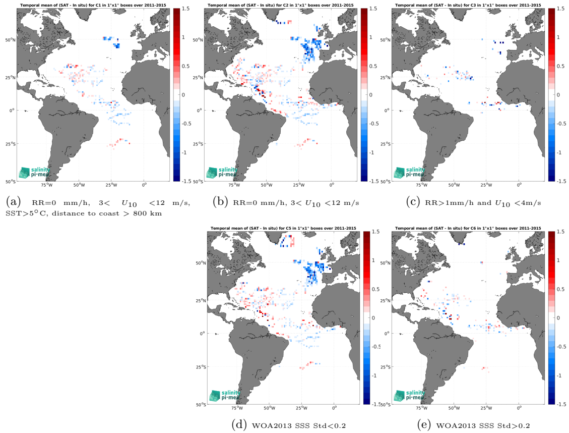
Figure 11: Temporal mean gridded over spatial boxes of size 1^\circ \times 1^\circ of \Delta\text{SSS} (Aquarius SSS L2 OR v5 (NASA-GSFC) - Surface drifters) for 5 different subdatasets corresponding to:RR=0 mm/h, 3 < U_{10} < 12 m/s, SST >5^\circ\text{C} , distance to coast > 800 km (a), RR=0 mm/h, 3 < U_{10} < 12 m/s (b), RR >1 mm/h and U_{10} < 4 m/s (c), WOA2013 SSS Std <0.2 (d), WOA2013 SSS Std >0.2 (e).
