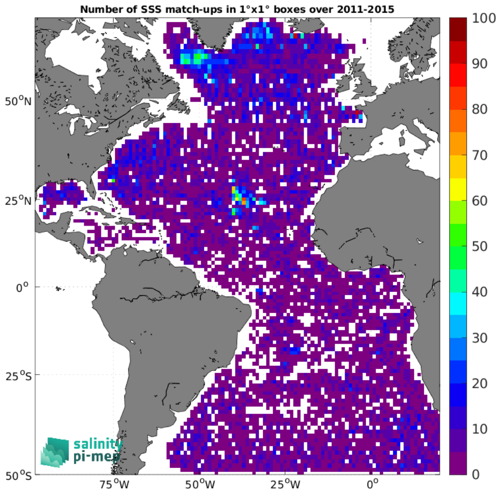
Figure 4: Number of SSS match-ups between Argo SSS and the Aquarius SSS L2 OR v5 (NASA-GSFC) SSS product for the Atlantic Ocean Pi-MEP region over 1°x1° boxes and for the full satellite product period.
