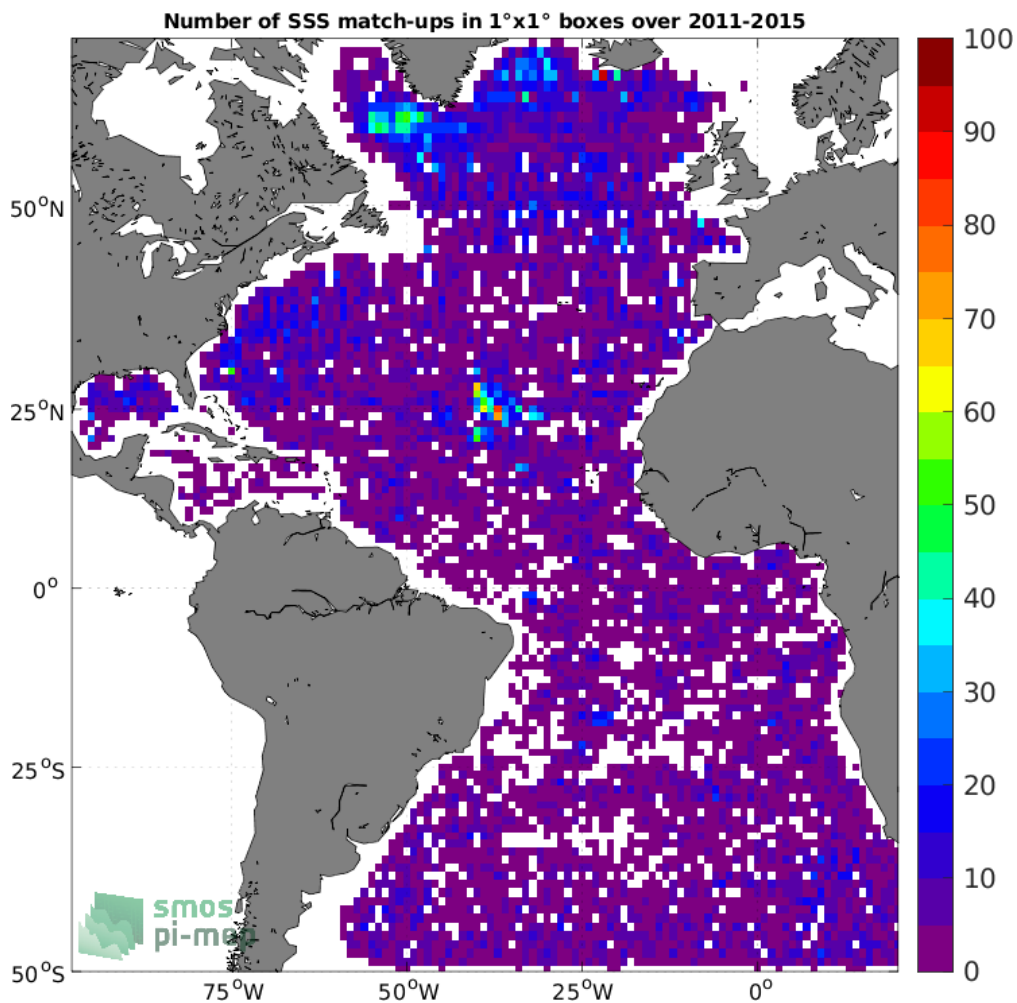
Figure 4: Number of SSS match-ups between Argo SSS and the Aquarius SSS L2 OR v5 (NASA-GSFC) SSS product for the Atlantic Ocean Pi-MEP region over 1°×1° boxes and for the full satellite product period.
