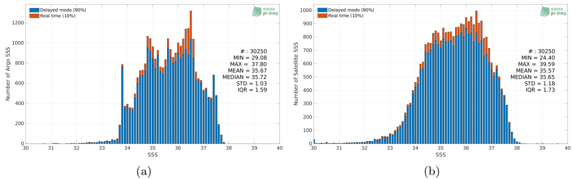
Figure 2: Histograms of SSS from Argo (a) and Aquarius SSS L2 OR v5 (NASA-GSFC) (b) considering all match-up pairs per bins of 0.1 over the Atlantic Ocean Pi-MEP region and for the full satellite product period.
