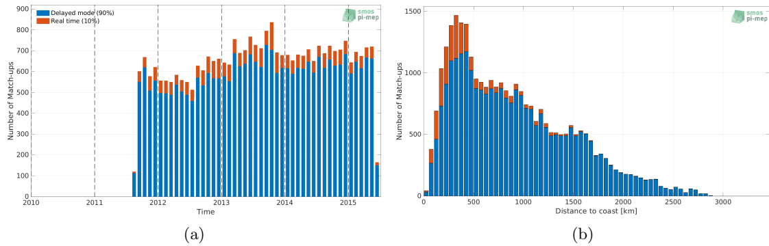
Figure 1: Number of match-ups between Argo and Aquarius SSS L2 OR v5 (NASA-GSFC) SSS as a function of time (a) and as function of the distance to coast (b) over the Atlantic Ocean Pi-MEP region and for the full satellite product period.
