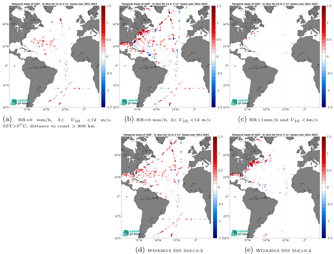
Figure 14: Temporal mean gridded over spatial boxes of size 1^\circ \times 1^\circ of \Delta\text{SSS} (Aquarius SSS L2 CAP v5 (JPL) - TSG (SAMOS)) for 5 different subdatasets corresponding to:RR=0 mm/h, 3 < U_{10} < 12 m/s, SST>5°C, distance to coast > 800 km (a), RR=0 mm/h, 3 < U_{10} < 12 m/s (b), RR>1mm/h and U_{10} < 4 m/s (c), WOA2013 SSS Std<0.2 (d), WOA2013 SSS Std>0.2 (e).
