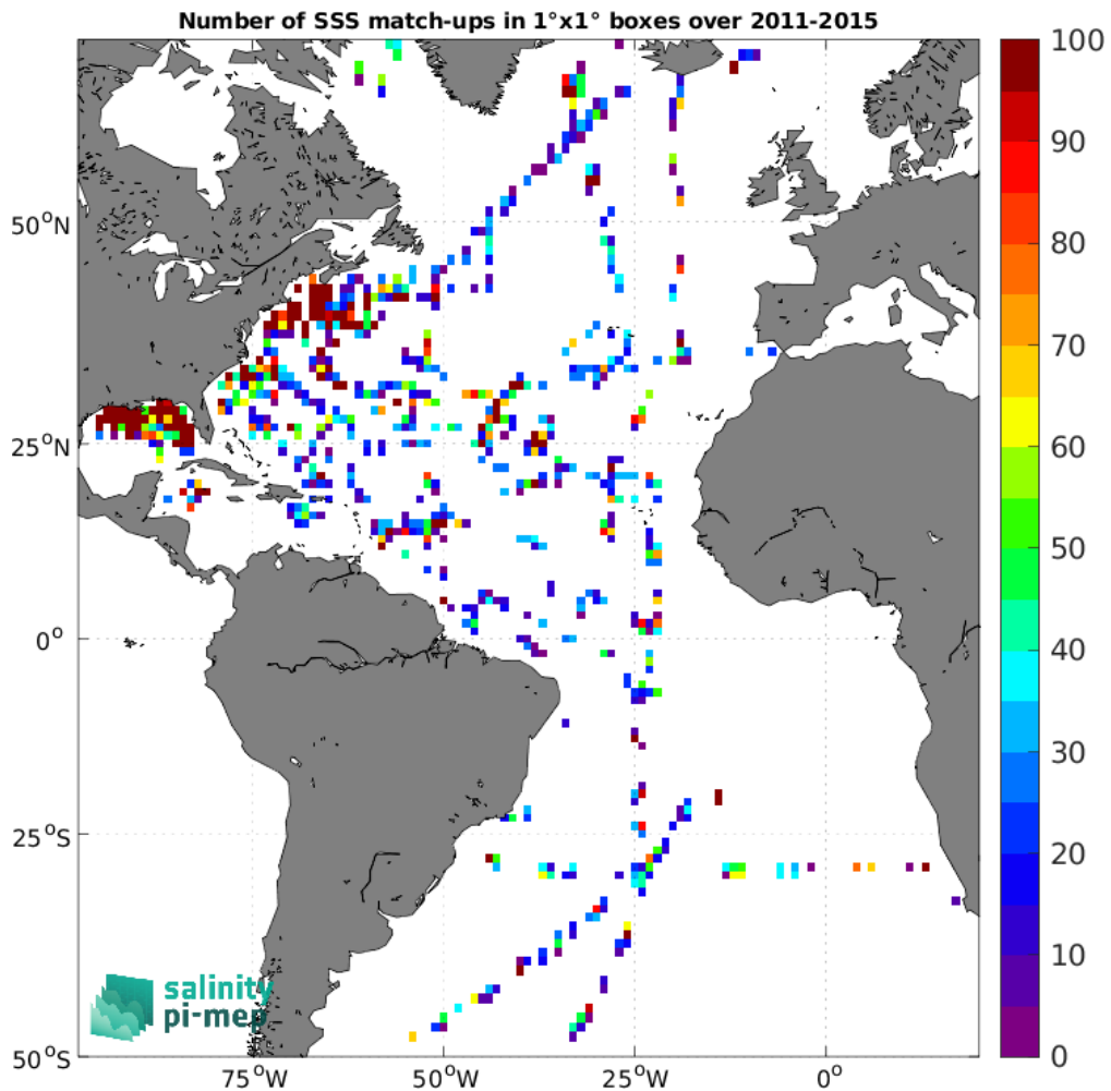
Figure 5: Number of SSS match-ups between TSG (SAMOS) SSS and the Aquarius SSS L2 CAP v5 (JPL) SSS product for the Atlantic Ocean Pi-MEP region over 1°x1° boxes and for the full satellite product period.
