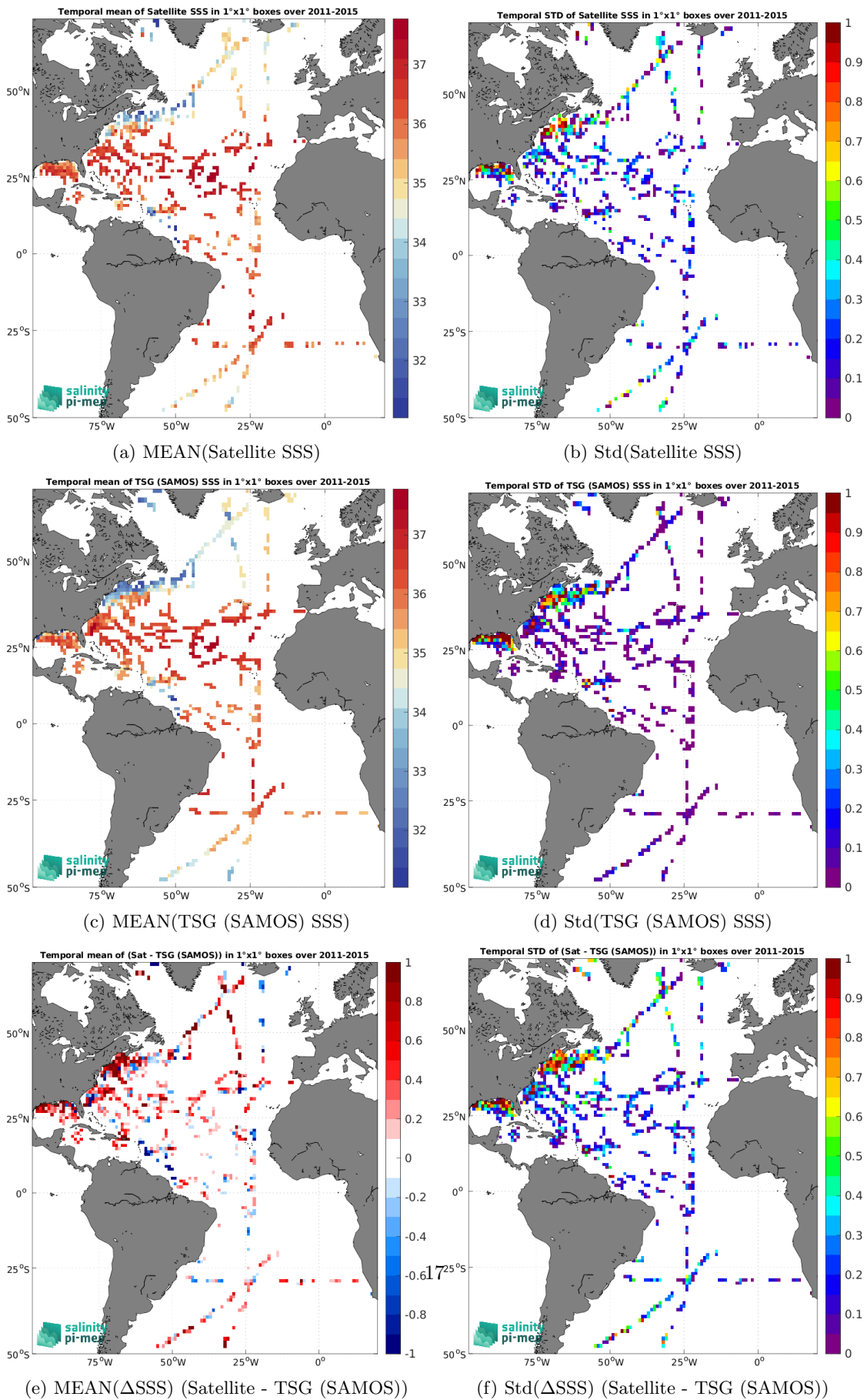
Figure 7: Temporal mean (left) and Std (right) of SSS from Aquarius SSS L2 CAP v5 (JPL) (top), TSG (SAMOS) (middle), and of \Delta SSS (Satellite - TSG (SAMOS)). Only match-up pairs are used to generate these maps.
