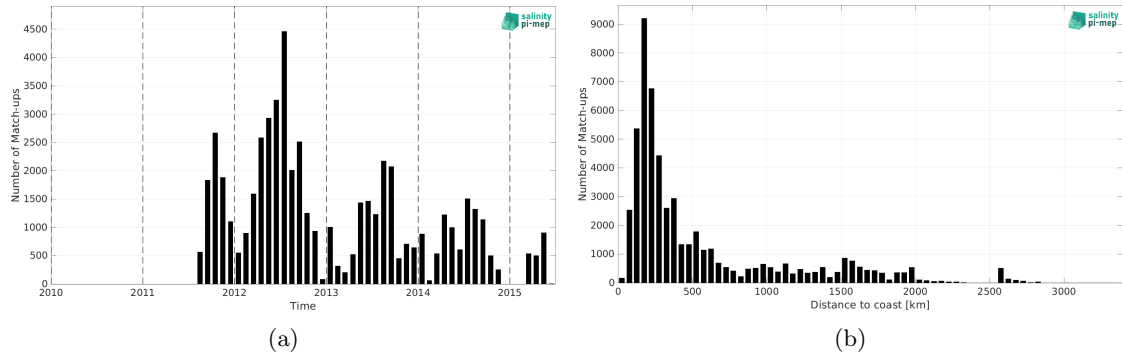
Figure 2: Number of match-ups between TSG (SAMOS) and Aquarius SSS L2 CAP v5 (JPL) SSS as a function of time (a) and as function of the distance to coast (b) over the Atlantic Ocean Pi-MEP region and for the full satellite product period.
