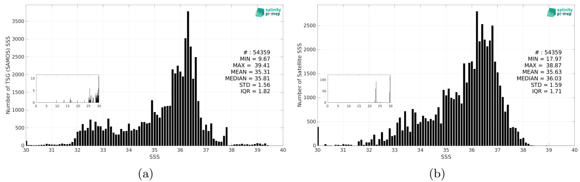
Figure 3: Histograms of SSS from TSG (SAMOS) (a) and Aquarius SSS L2 CAP v5 (JPL) (b) considering all match-up pairs per bins of 0.1 over the Atlantic Ocean Pi-MEP region and for the full satellite product period.
