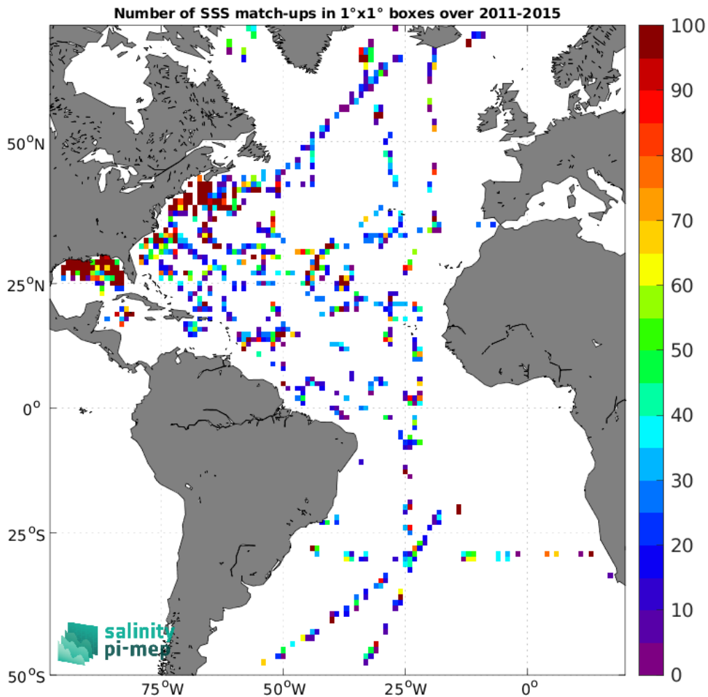
Figure 5: Number of SSS match-ups between TSG (SAMOS) SSS and the Aquarius SSS L2 CAP v5 (JPL) SSS product for the Atlantic Ocean Pi-MEP region over 1^\circ \times 1^\circ boxes and for the full satellite product period.
