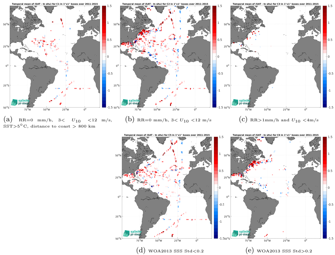
Figure 14: Temporal mean gridded over spatial boxes of size 1^\circ \times 1^\circ of \Delta SSS (Aquarius SSS L2 CAP v5 (JPL) - TSG (SAMOS)) for 5 different subdatasets corresponding to:RR=0 mm/h, 3 < U_{10} < 12 m/s, SST >5^\circ\text{C} , distance to coast > 800 km (a), RR=0 mm/h, 3 < U_{10} < 12 m/s (b), RR >1 mm/h and U_{10} < 4 m/s (c), WOA2013 SSS Std <0.2 (d), WOA2013 SSS Std >0.2 (e).
