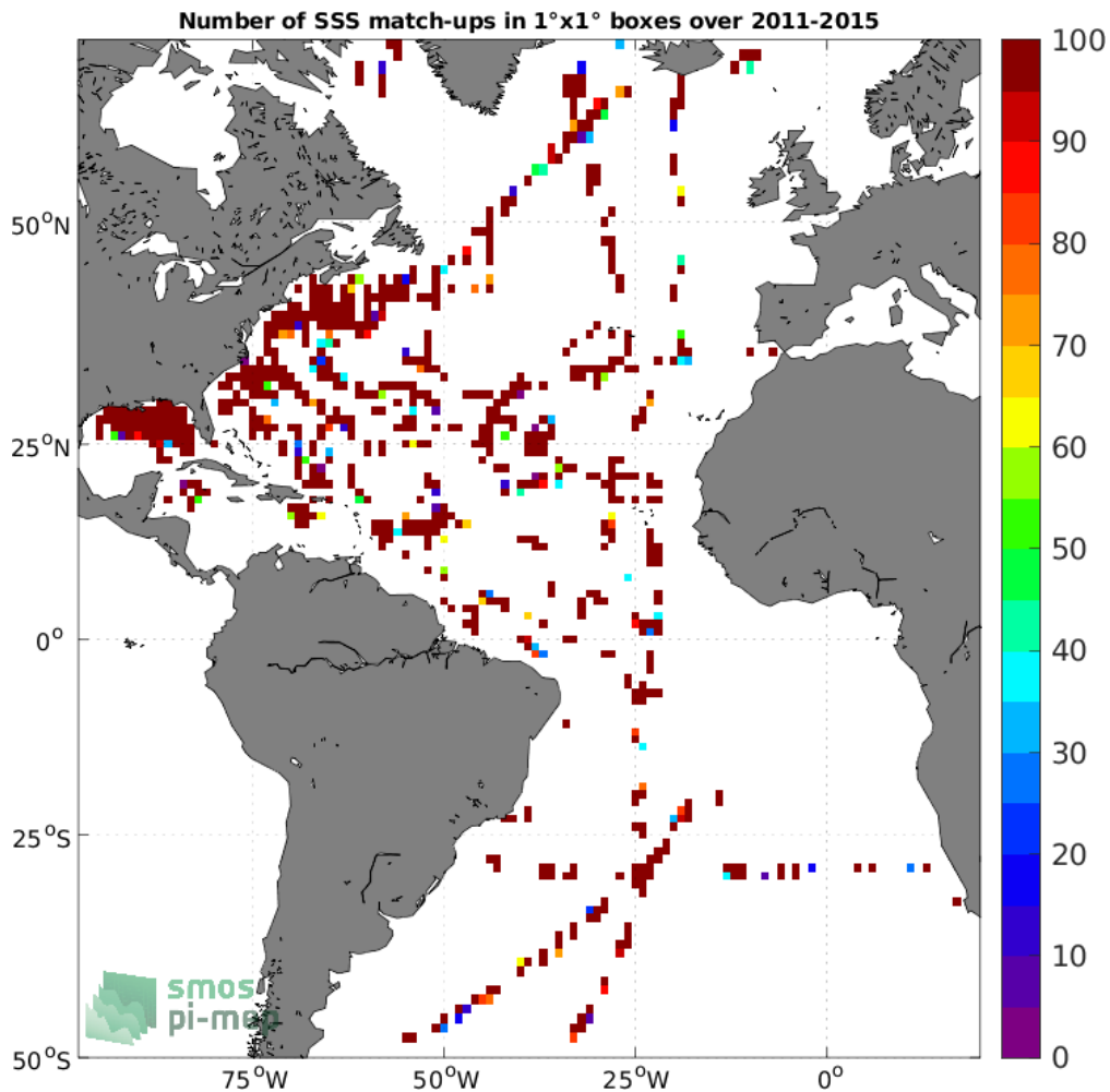
Figure 4: Number of SSS match-ups between TSG (SAMOS) SSS and the Aquarius SSS L2 CAP v5 (JPL) SSS product for the Atlantic Ocean Pi-MEP region over 1°x1° boxes and for the full satellite product period.
