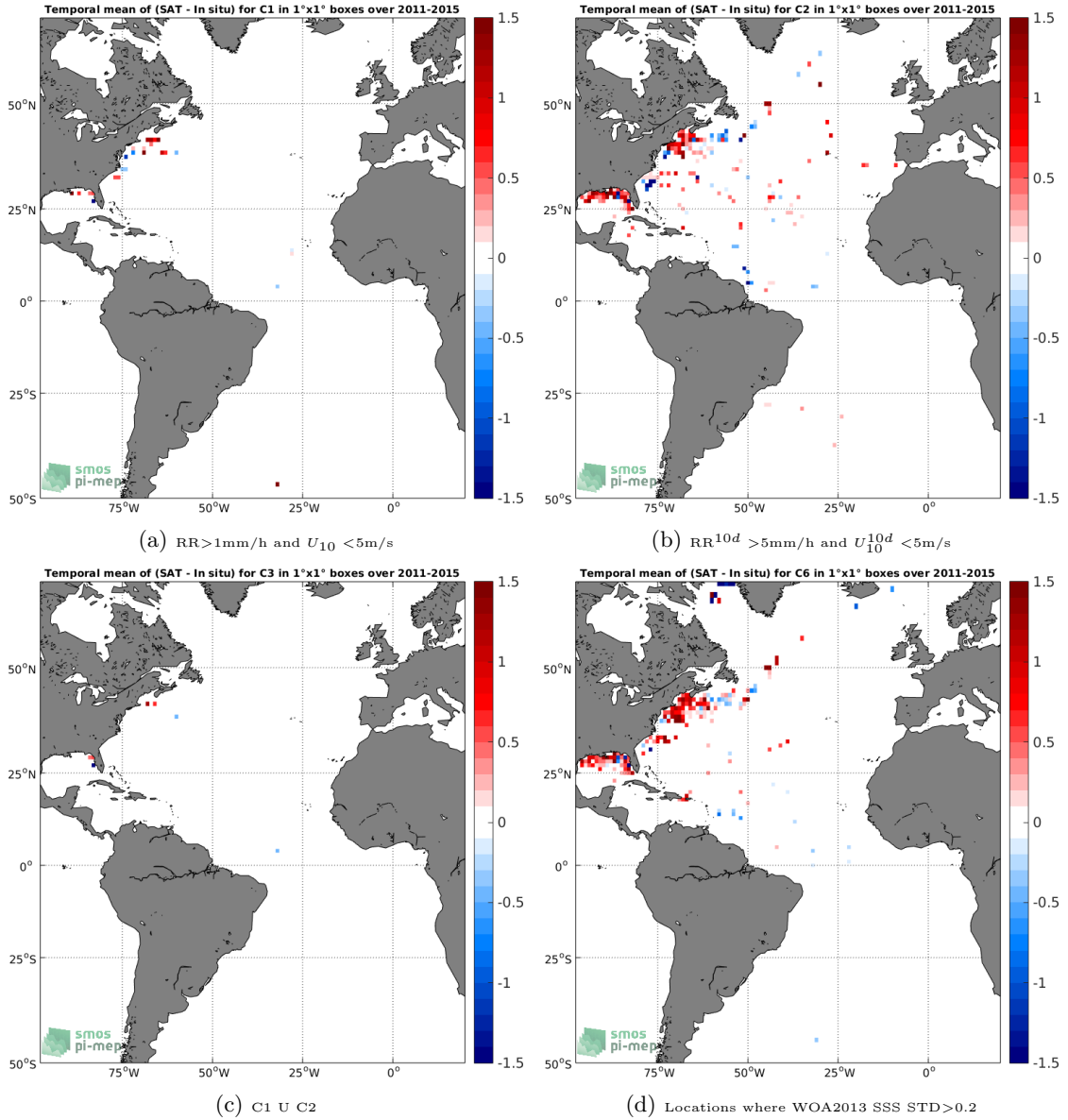
Figure 12: Temporal mean gridded over spatial boxes of size 1^\circ \times 1^\circ of \Delta SSS (Aquarius-L2-JPL-V5 - TSG-SAMOS) for 4 different subdatasets corresponding to: RR > 1mm/h and U_{10} < 5\text{m/s} (a), RR^{10d} > 5\text{mm/h} and U_{10}^{10d} < 5\text{m/s} (b), C1 U C2 (c), Locations where WOA2013 SSS STD > 0.2 (d).
