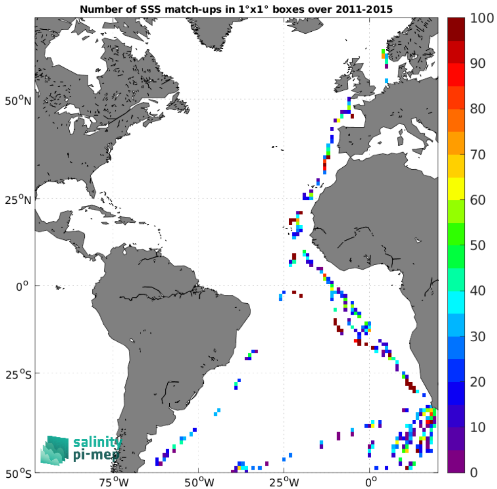
Figure 5: Number of SSS match-ups between TSG (Polarstern) SSS and the Aquarius SSS L2 CAP v5 (JPL) SSS product for the Atlantic Ocean Pi-MEP region over 1°×1° boxes and for the full satellite product period.
