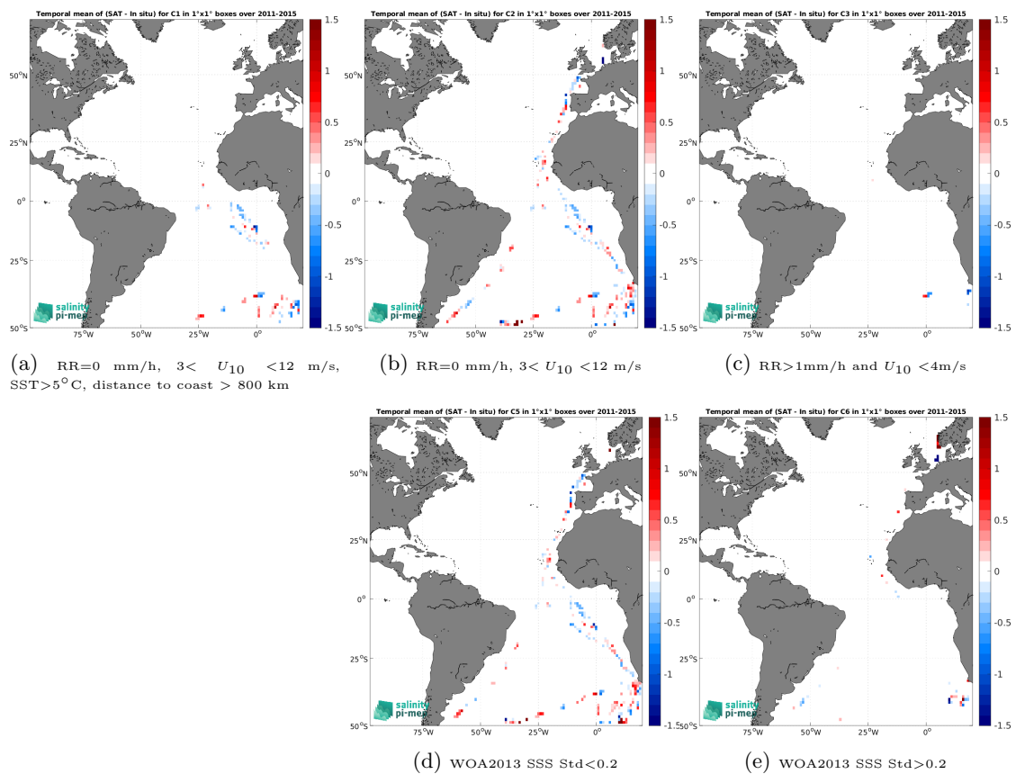
Figure 14: Temporal mean gridded over spatial boxes of size 1^\circ \times 1^\circ of \Delta SSS (Aquarius SSS L2 CAP v5 (JPL) - TSG (Polarstern)) for 5 different subdatasets corresponding to:RR=0 mm/h, 3 < U_{10} < 12 m/s, SST >5^\circ\text{C} , distance to coast > 800 km (a), RR=0 mm/h, 3 < U_{10} < 12 m/s (b), RR >1 mm/h and U_{10} < 4 m/s (c), WOA2013 SSS Std <0.2 (d), WOA2013 SSS Std >0.2 (e).
