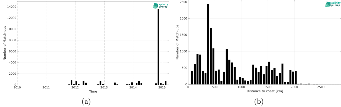
Figure 2: Number of match-ups between TSG (Polarstern) and Aquarius SSS L2 CAP v5 (JPL) SSS as a function of time (a) and as function of the distance to coast (b) over the Atlantic Ocean Pi-MEP region and for the full satellite product period.
