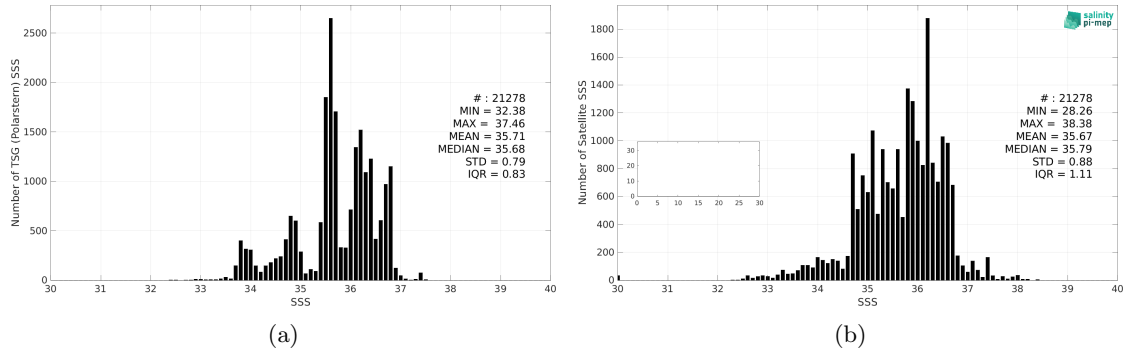
Figure 3: Histograms of SSS from TSG (Polarstern) (a) and Aquarius SSS L2 CAP v5 (JPL) (b) considering all match-up pairs per bins of 0.1 over the Atlantic Ocean Pi-MEP region and for the full satellite product period.
