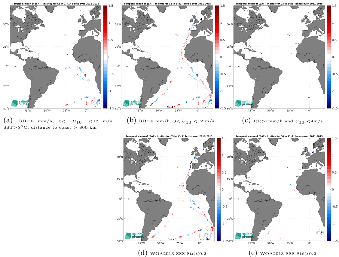
Figure 12: Temporal mean gridded over spatial boxes of size 1^\circ \times 1^\circ of \Delta SSS (Aquarius SSS L2 CAP v5 (JPL) - TSG (Polarstern)) for 5 different subdatasets corresponding to:RR=0 mm/h, 3 < U_{10} < 12 m/s, SST >5^\circ\text{C} , distance to coast > 800 km (a), RR=0 mm/h, 3 < U_{10} < 12 m/s (b), RR >1 mm/h and U_{10} < 4 m/s (c), WOA2013 SSS Std <0.2 (d), WOA2013 SSS Std >0.2 (e).
