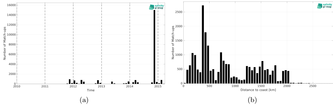
Figure 1: Number of match-ups between TSG (Polarstern) and Aquarius SSS L2 CAP v5 (JPL) SSS as a function of time (a) and as function of the distance to coast (b) over the Atlantic Ocean Pi-MEP region and for the full satellite product period.
