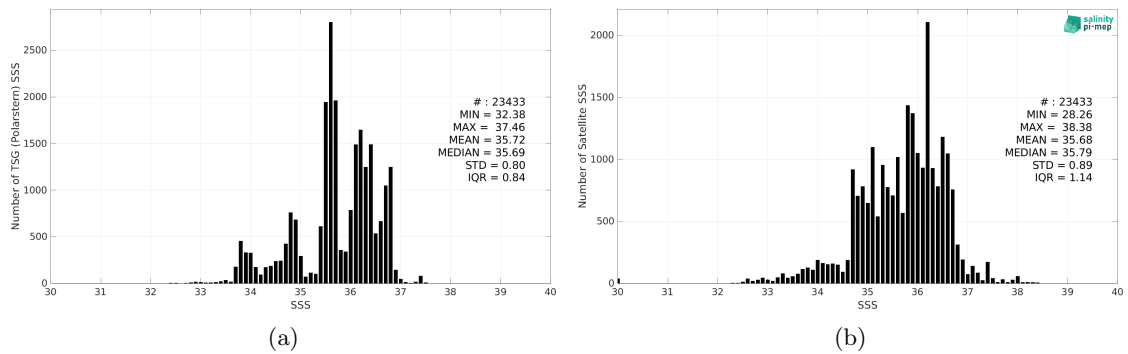
Figure 2: Histograms of SSS from TSG (Polarstern) (a) and Aquarius SSS L2 CAP v5 (JPL) (b) considering all match-up pairs per bins of 0.1 over the Atlantic Ocean Pi-MEP region and for the full satellite product period.
