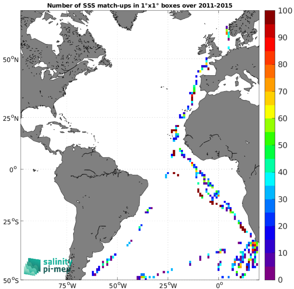
Figure 4: Number of SSS match-ups between TSG (Polarstern) SSS and the Aquarius SSS L2 CAP v5 (JPL) SSS product for the Atlantic Ocean Pi-MEP region over 1°×1° boxes and for the full satellite product period.
